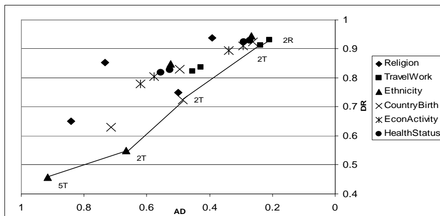
Figure 1. R-U confidentiality map with DR (proportion of unperturbed unique cells) on the y-axis and the AD (distance metric) on the x-axis for all Census tables
