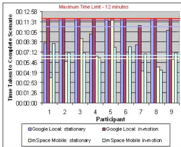
FIGURE 2: Graph showing the performance times of each participant in the four conditions
