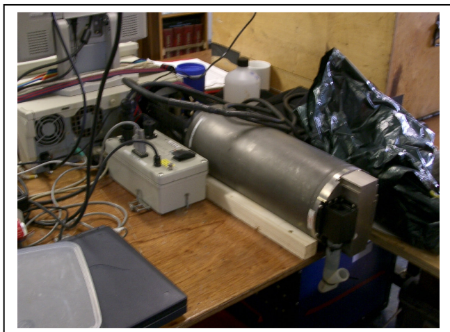
Figure 2. Chelsea Instruments Fast Rate Repetition Fluorometer.
