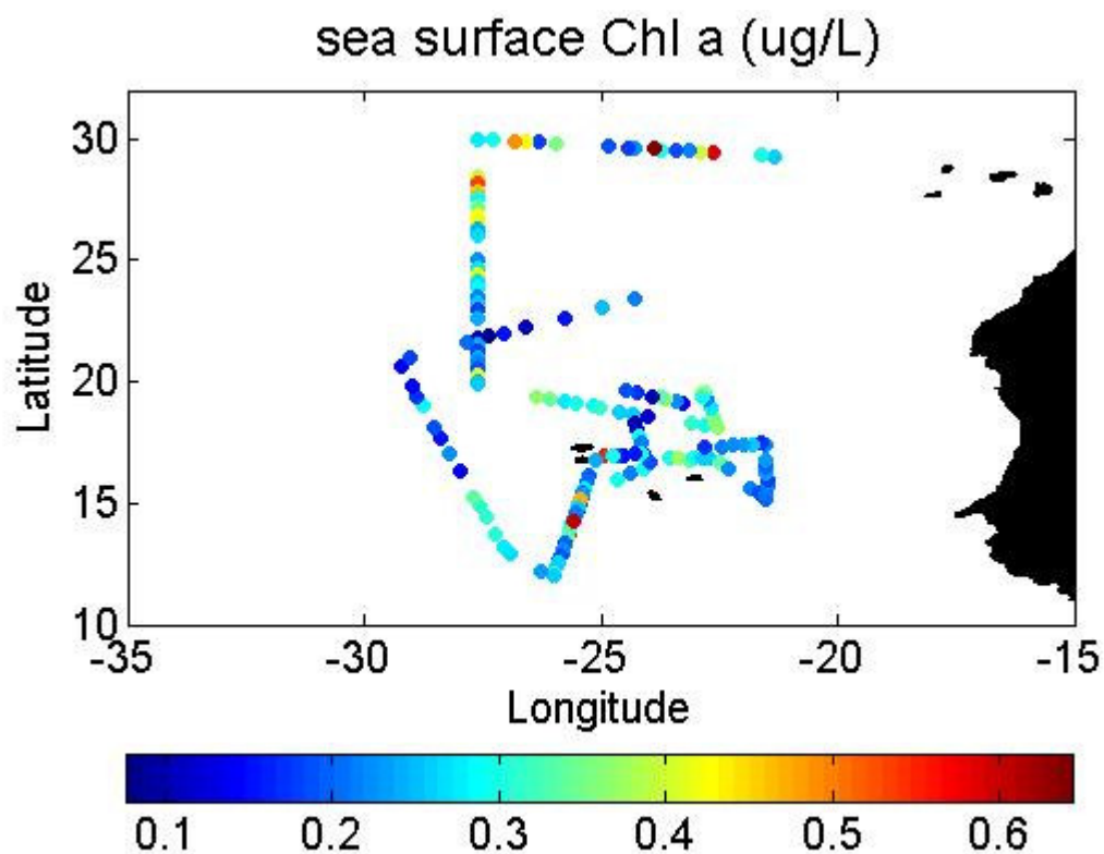
Figure 6. The geographical distribution of the sea surface concentration of chlorophyll a during the UKSOLAS Poseidon 332 cruise.
