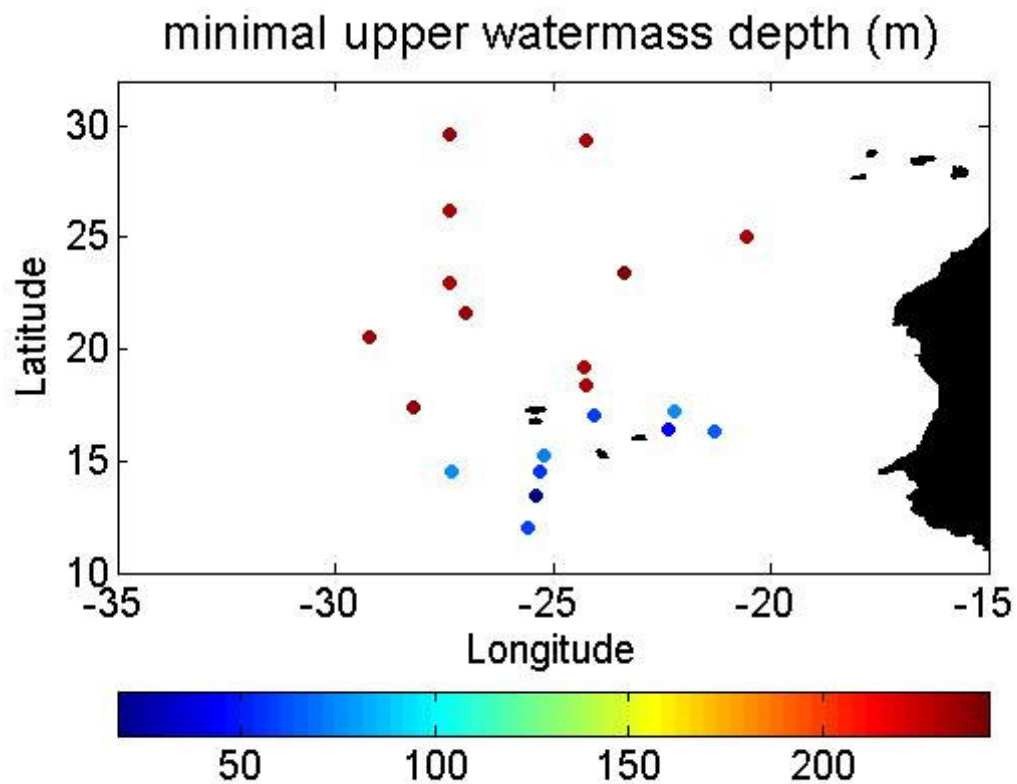
Figure 4. The minimal depth of the mixed layer according to the temperature-salinity property-property plots. The salinity and temperature data of the CTD log sheets were used as the full salinity and temperature data set from the CTD was not yet available.
