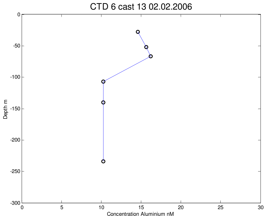
Figure 1. CTD 6 profile
