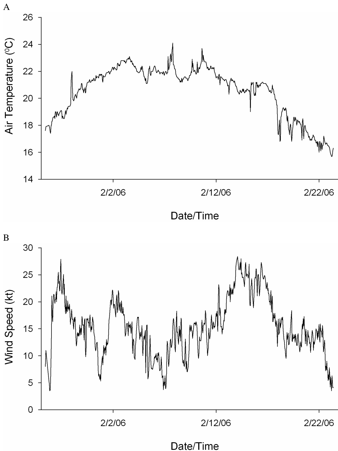
Figure 5. A) The air temperature (°C), and B) the absolute wind speed (knots) during the UKSOLAS Poseidon 332 cruise.
