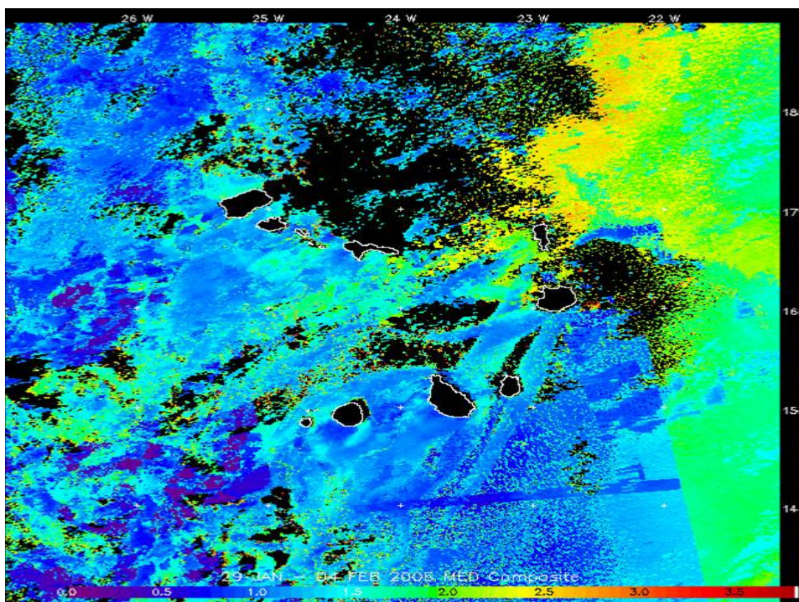
Figure 7. Composite (29 Jan.-4 Feb., 2006) Modis image of the tau865 (aerosol optical thickness at 865 nm).
