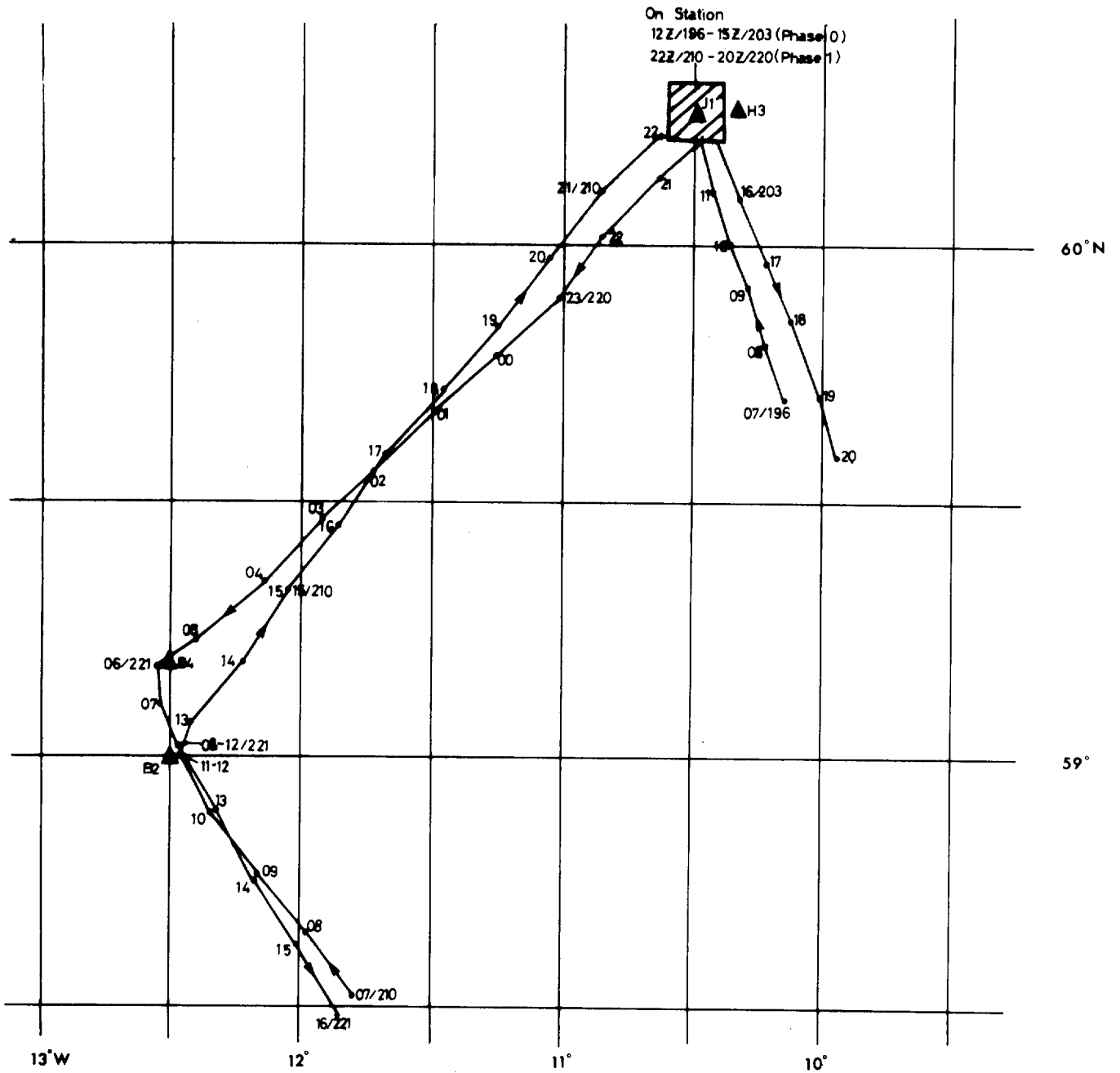
Fig. 2 Track chart (JASIN area, legs 1 and 2). Solid circles indicate hourly positions when steaming. Numbers alongside circles indicate Time (GMT)/Julian Day. Hatched areas show where the vessel remained within a few miles of station for long periods.
