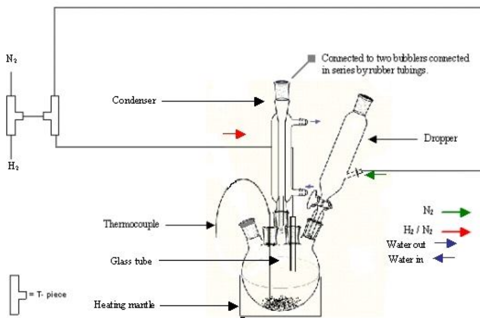
Figure 2- 3 Schematic diagram of the reactor used for CSR
