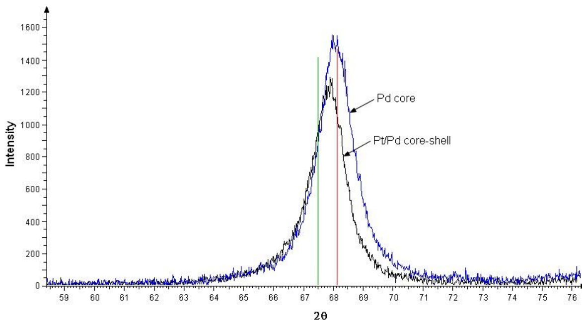
Figure 3 - 9 Representation of (220) diffraction for the Pd core and the Pt/Pd core-shell.
