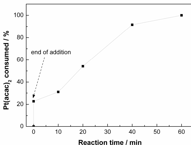
Figure 3 - 7 Consumption of Pt(acac) 2 during CSR. The reaction time t = 0 corresponds to the end of the precursor addition to the vessel.
