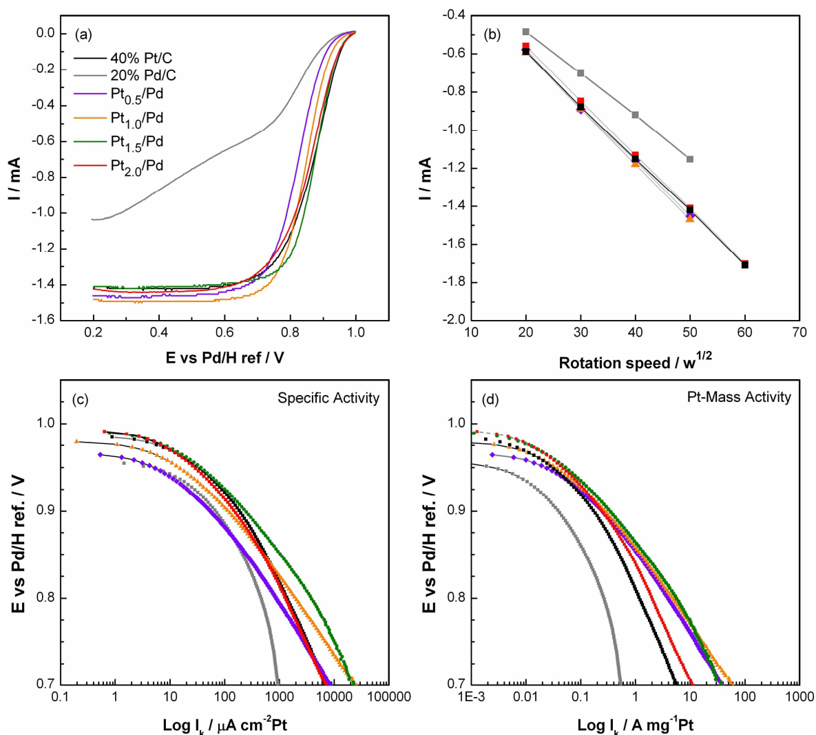
Figure 4- 18 Polarisation curves (backward scans) for the ORR on Pt_x/Pd core-shell catalysts and 40% Pt/C (a). Levich plots (b). Tafel plots corrected for the electrochemical area (c) and for the Pt mass (d). Electrode geometric area: 0.196 cm 2 .
