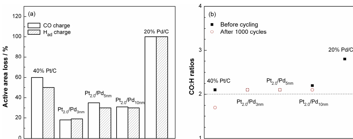
Figure 5- 17 Calculated loss of active area (a) and the corresponding CO:H ratio (b) for the voltammograms shown in Figure 5-16.
