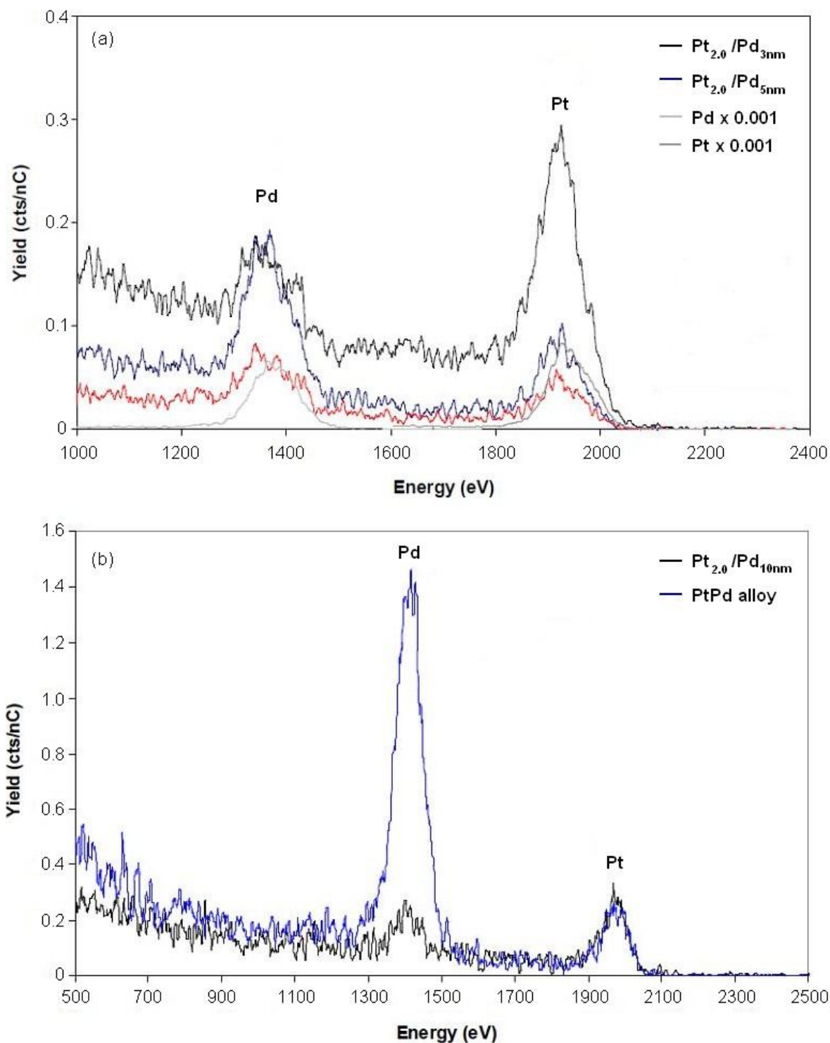
Figure 5- 13 3keV ^{20}\text{Ne}^+ spectra of the Pt_{2.0}/Pd_{3nm} and Pt_{2.0}/Pd_{5nm} after the reduction treatment, compared to the spectra for the Pd and Pt reference (a). The spectra for the references have been multiplied by 0.001 to facilitate comparison. 3keV ^{20}\text{Ne}^+ spectra of the Pt_{2.0}/Pd_{10nm} and a PtPd of same bulk composition after the reduction treatment (b).
