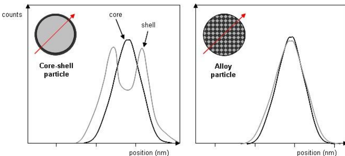
Figure 3 - 10 Models of the EDX line profile for core-shell and alloy particles along red scan line, as depicted in Figures 3-12 and 3-13.
