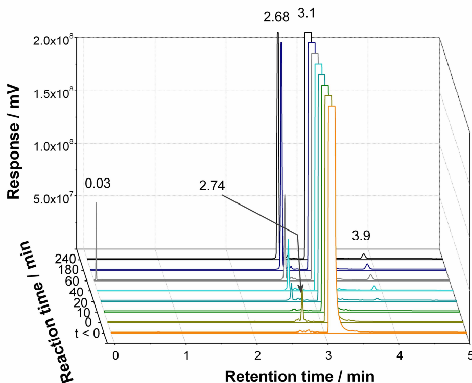
Figure 3 - 3 Evolution of the reaction mixture composition during the reaction as formed by GC. Retention times are identified in Table 3-3.
