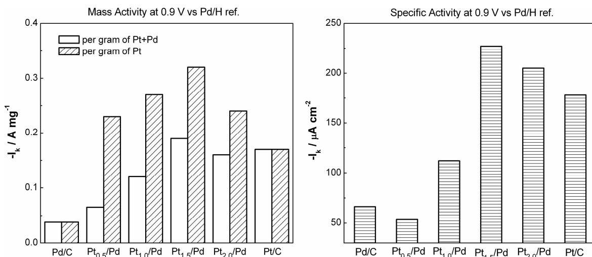
Figure 4- 19 Relationship between the Pt coverage and the ORR mass activity (a) and specific activity (b) at 0.9 V vs Pd/H ref. determined by analysis of the polarisation curves reported in Figure 4-18(a).
