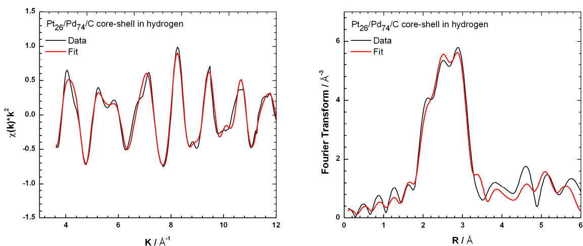
Figure 3 - 15 Pt/Pd core-shell: k^2 -weighed \chi(k) spectrum collected at Pt L III edge obtained in H 2 atmosphere; (right) k^2 -weighed Fourier transform of the \chi(k) data.
