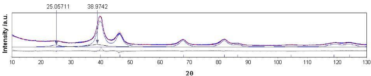
Figure 4- 2 Rietveld profile fitting for Pt_{2.0}/Pd XRD pattern.
