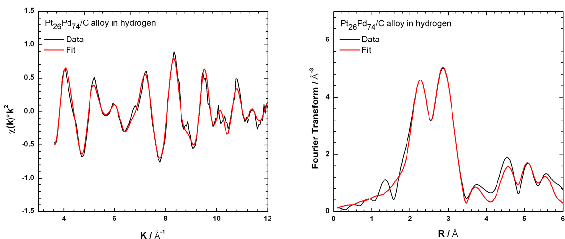
Figure 3 - 16 Pt-Pd alloy: k^2 -weighed \chi(k) spectrum collected at Pt L III edge obtained in H 2 atmosphere; (right) k^2 -weighed Fourier transform of the \chi(k) data.
