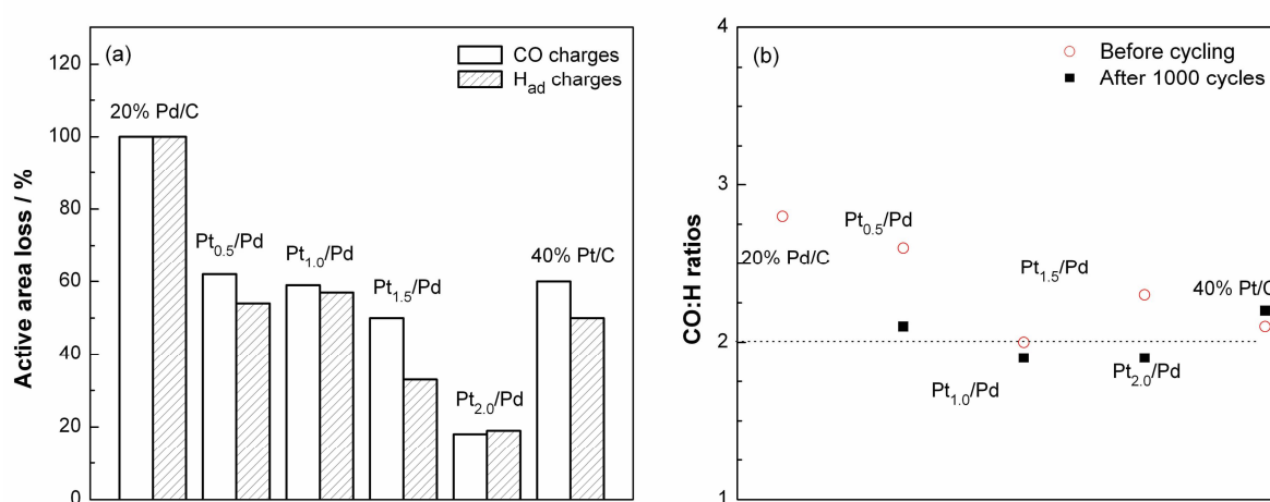
Figure 4- 15 Calculated loss of hydrogen sorbed charges for the voltammograms shown in Figure 4-14.
