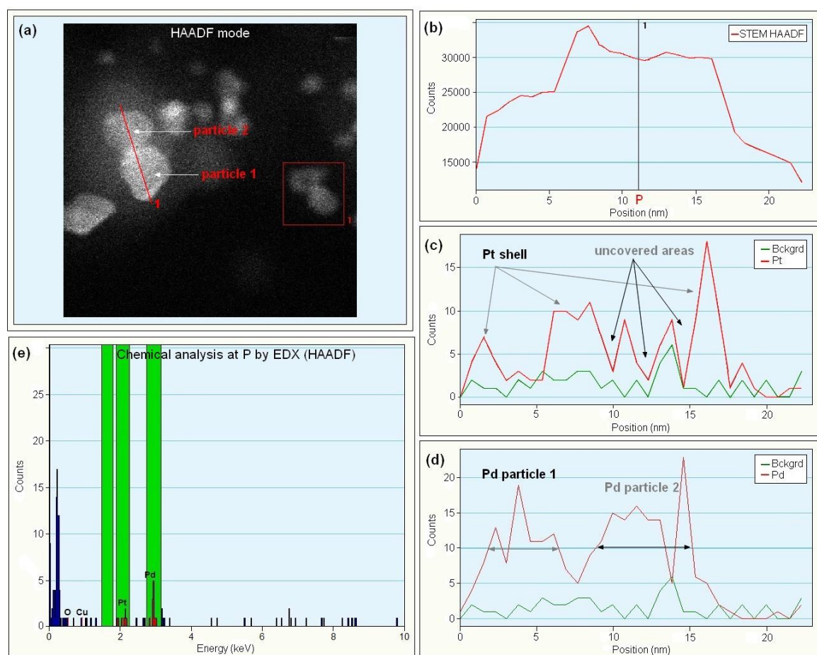
Figure 5- 12 STEM micrographs of Pt_{2.0}/Pd_{10nm} particles in HAADF mode (a). EDX profiles for the sum (Pt+Pd) counts (b), the Pt counts (c) and the Pd counts across the two core-shell particles following the red line in picture a (d). Chemical analysis at position P (e).
