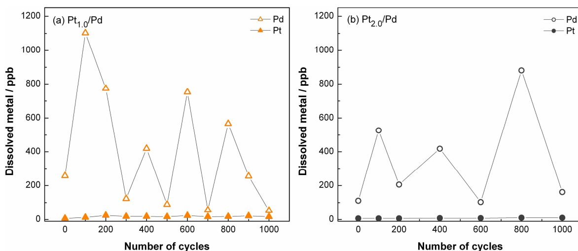
Figure 4- 17 Pd and Pt dissolution during stability test for Pt_{1.0}/Pd (a) and Pt_{2.0}/Pd (b).
