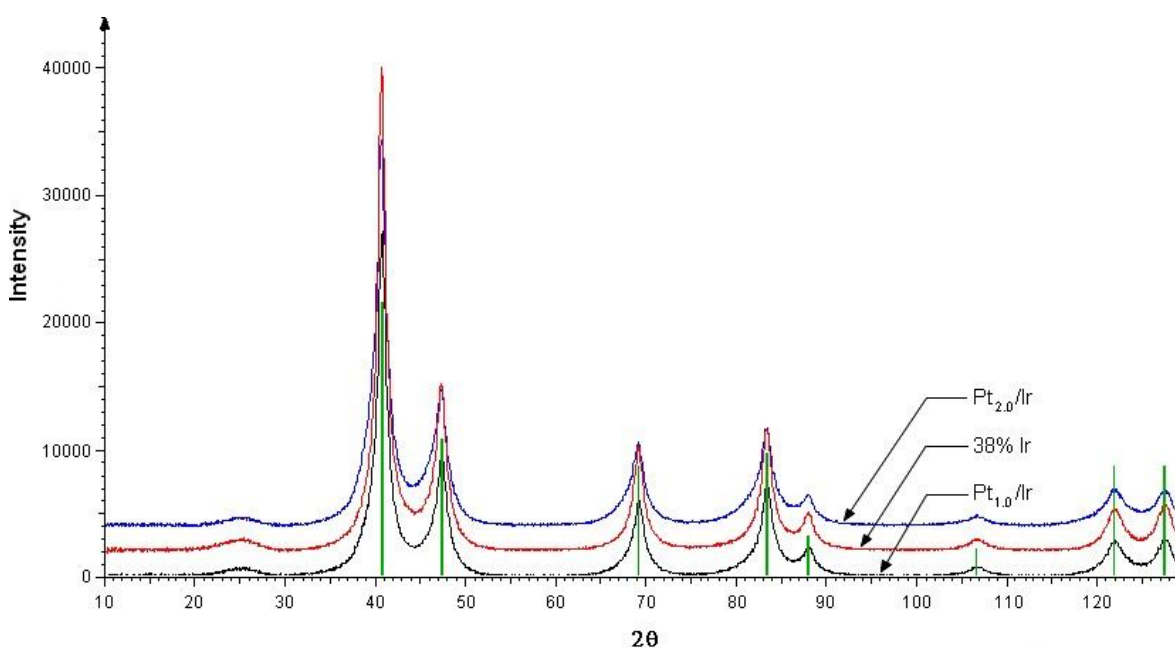
Figure 6 - 1 Overlaid XRD patterns of 38% Ir/C, Pt_{1.0}/Ir and Pt_{2.0}/Ir . The green lines represented the documented Ir diffraction lines.
