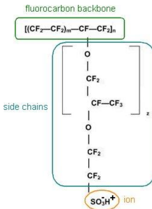
Figure 1- 3 Chemical structure of Nafion™ (by Dupont) membrane material
