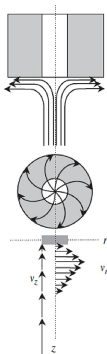
Figure 2- 16 Streamlines for flow and vector representation of fluid velocities near a rotating disc electrode (16).
