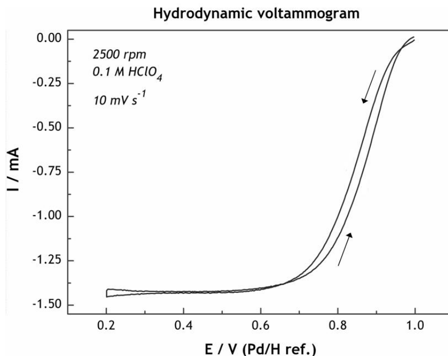
Figure 2- 17 Typical rotating disk voltammogram for a carbon-supported Pt catalyst in 0.1 M \text{HClO}_4 , at 10 \text{ mV s}^{-1} , from 1.0 V to 0.2 V at a rotating speed of 2500 rpm.
