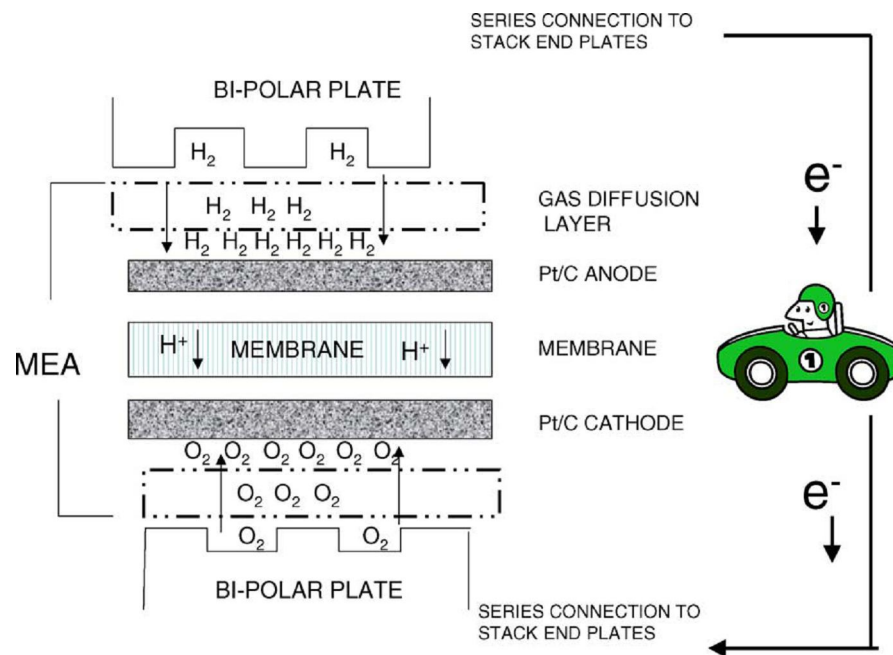
Figure 1- 1 Membrane electrode assembly arranged in a stack (11)
