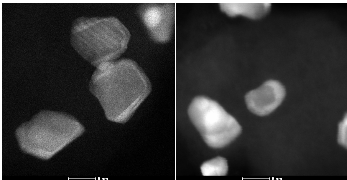
Figure 3 - 11 Aberration corrected STEM images of Pt/Pd/C core-shell.
