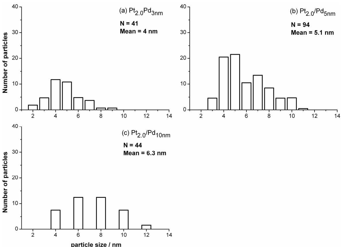
Figure 5-9 Particle size distribution bar charts for Pt_{2.0}/Pd_{3nm} (a), Pt_{2.0}/Pd_{5nm} (b) and Pt_{2.0}/Pd_{10nm} (c).
