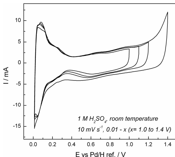
Figure 6 - 10 Window opening experiment on 38% Ir/C, in which the anodic limit was changed (1.0, 1.1, 1.2, 1.4 V), in 1 dm^3 H_2SO_4 , Scan rate: 10 mV s^{-1} .
