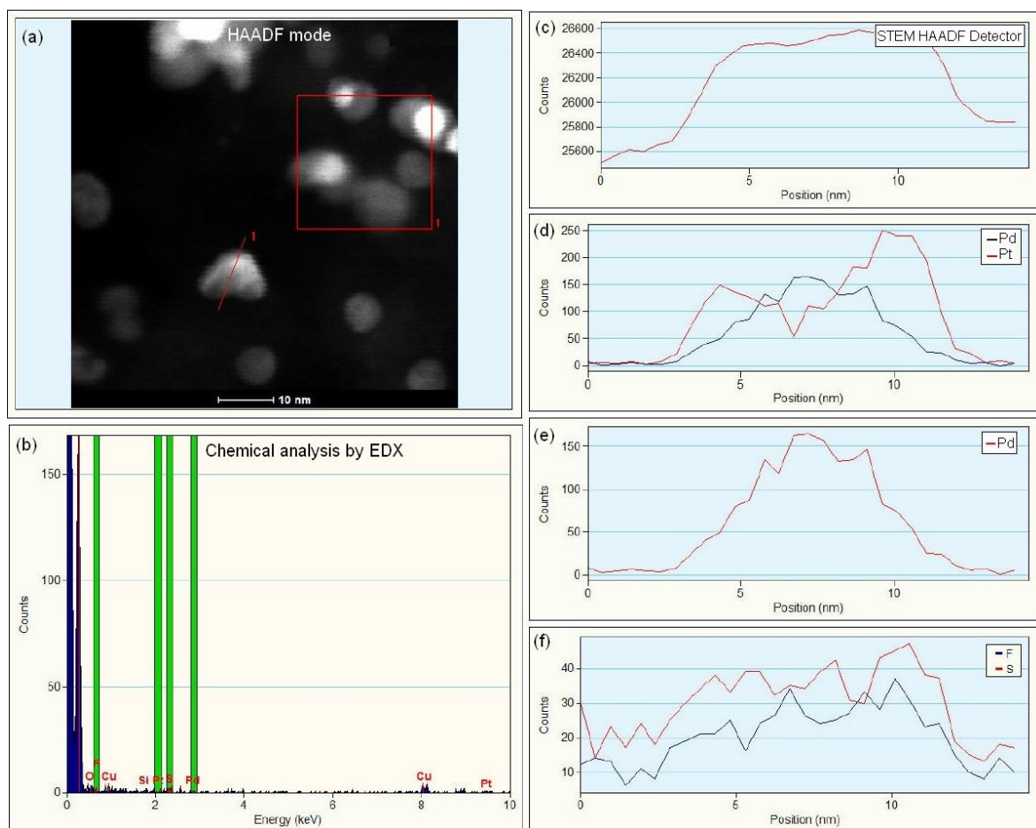
Figure 5- 20 HRTEM/EDX analyses of Pt_{2.0}/Pd_{5nm} electrode after cycling. HRTEM micrographs of Pt_{2.0}/Pd_{5nm} particles in HAADF mode (a). Chemical analysis (b). EDX profiles for total HRTEM signal (c), those of Pt and Pd (d), that of Pd only (e) and those of F and S across the two core-shell particles following the red line in picture (f).
