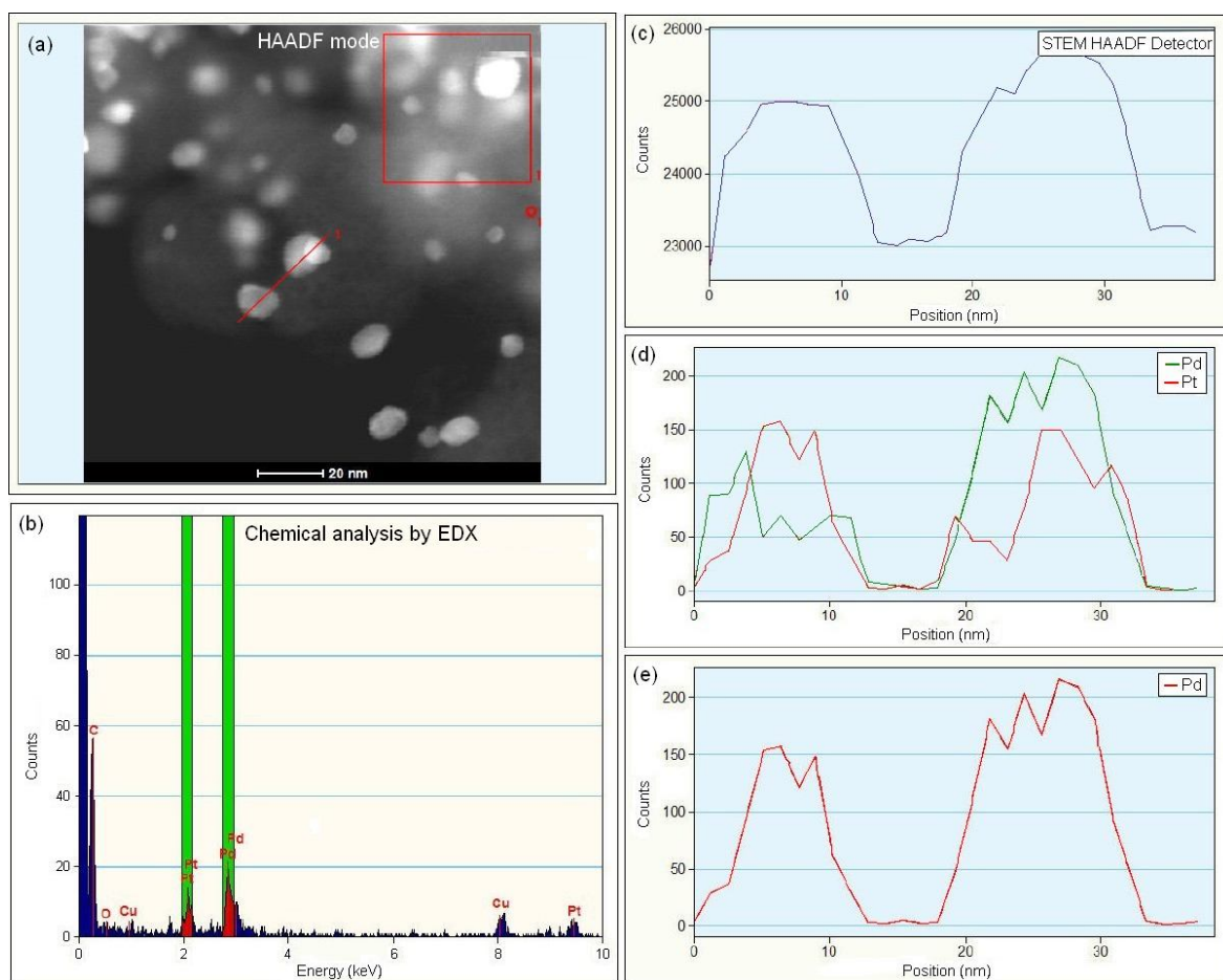
Figure 5- 19 HRTEM/EDX analyses of Pt_{2.0}/Pd_{5nm} electrode before cycling. HRTEM micrographs of Pt_{2.0}/Pd_{5nm} particles in HAADF mode (a). Chemical analysis (b). EDX profiles for total HRTEM signal (c), the Pt and Pd counts (d) and the Pd counts across the two core-shell particles following the red line in picture (a) (e).
