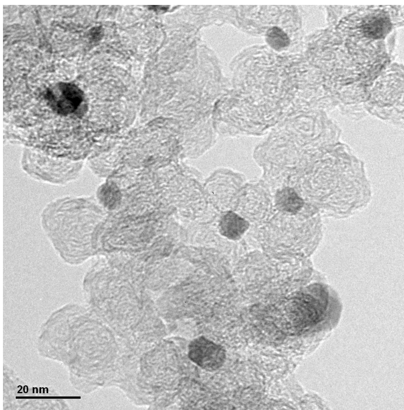
Figure 5- 3 TEM micrograph of carbon-supported Pd 10nm . Scale bar: 20 nm.
