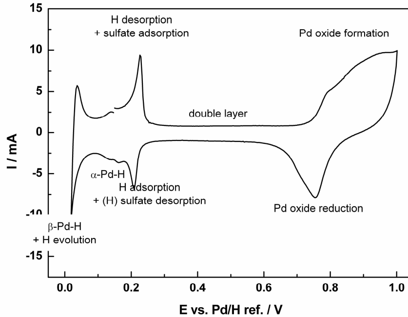
Figure 4-10 Cyclic voltammogram of 20% Pd/C ( 0.18 \text{ mgPt/cm}^2 ) in 1 M \text{H}_2\text{SO}_4 at 80^\circ\text{C}
