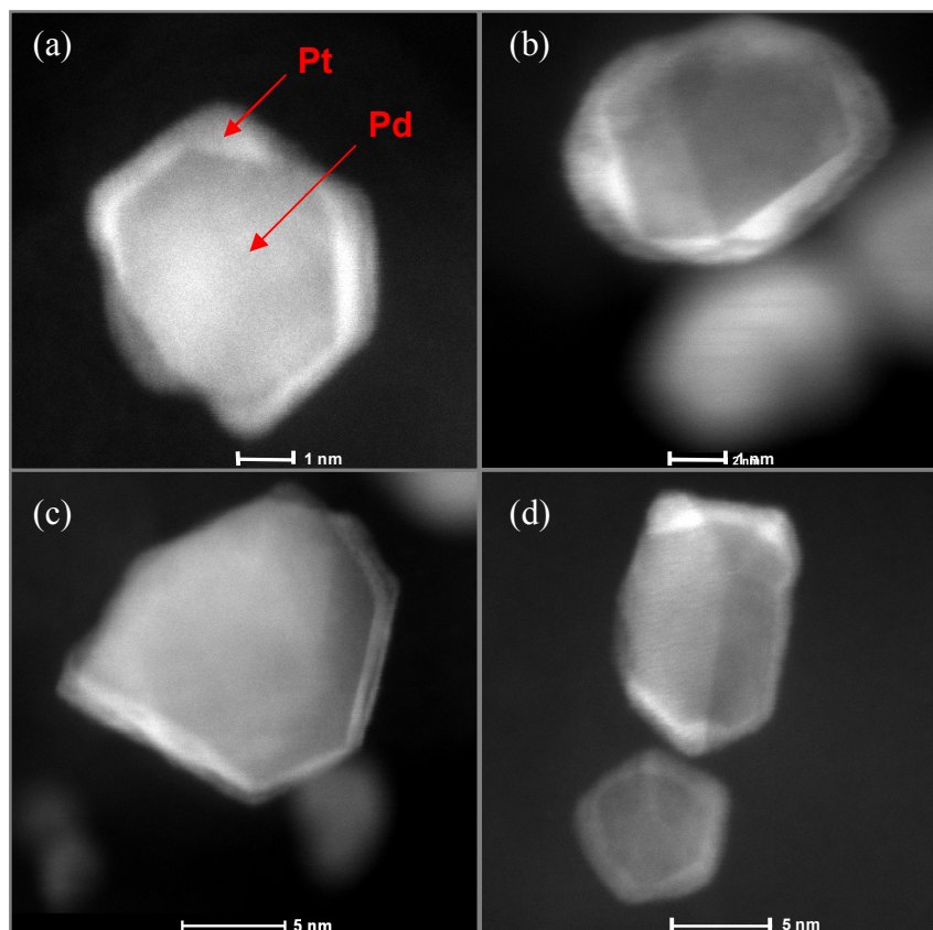
Figure 4- 6 Aberration-corrected STEM images of Pt_{2.0}/Pd core-shell catalyst.
