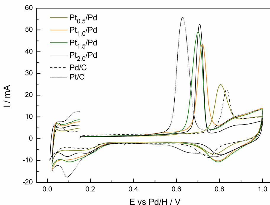
Figure 4- 13 CO cyclic voltammograms of 20% Pd/C, Pt_{0.5}/Pd , Pt_{1.0}/Pd , Pt_{1.5}/Pd , Pt_{2.0}/Pd and 40% Pt/C in 1 M H_2SO_4 at 80 °C
