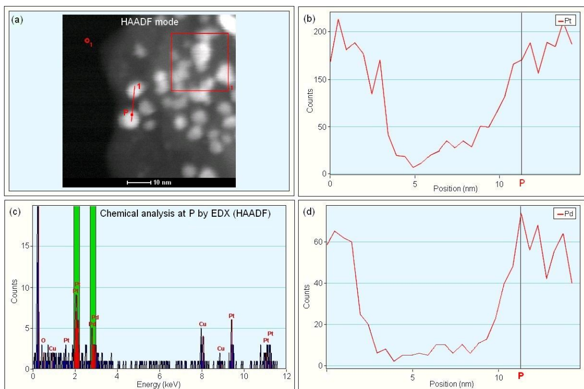
Figure 5- 10 HRTEM micrographs of Pt_{2.0}/Pd_{3nm} particles in HAADF mode (a). EDX Pt profile across two core-shell particles following the red line in picture a (b). Chemical analysis at position P (c). EDX Pd profile across the two core-shell particles (d).
