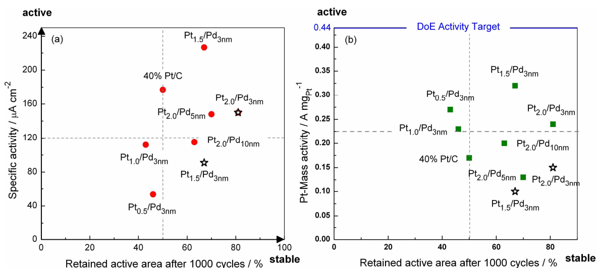
Figure 7- 2 Classification of the Pt/Pd core-shell electrocatalysts by specific activity (a), Pt-mass activity and electrochemical stability. The star symbol signifies the activity was measured in a single cell.
