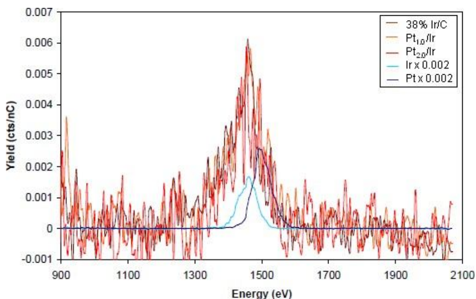
Figure 6 - 7 The 8keV ^{84}Kr^+ ToF Filtered LEIS spectra, after background subtraction, for Pt_{1.0}/Ir , Pt_{2.0}/Ir and 38% Ir/C.
