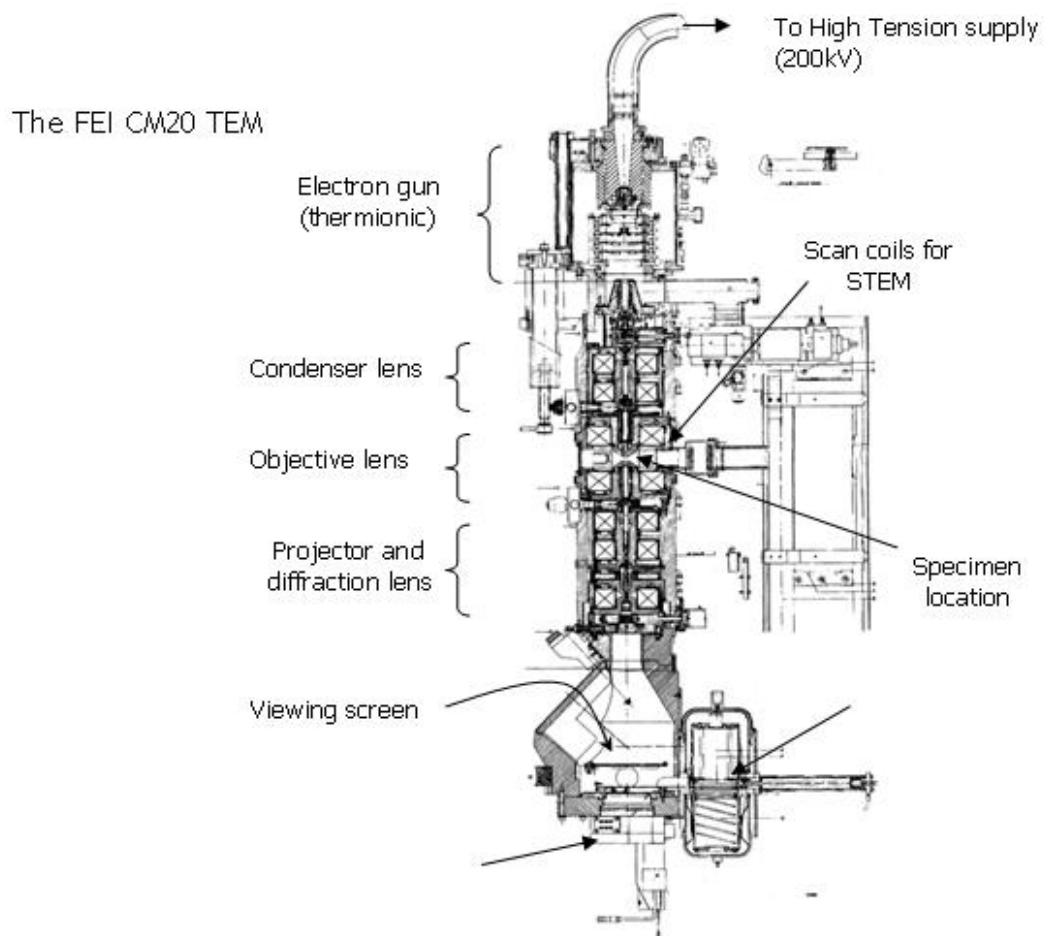
Figure 2- 4 Transmission electron microscope similar to the one used in this study.
