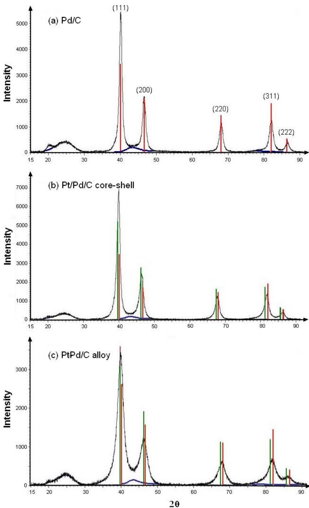
Figure 3 - 8 XRD patterns for Pd/C core catalyst (a), the Pt/Pd/C core-shell catalyst (b) and the PtPd/C alloy. The red and green lines represent the documented diffraction peaks of Palladium and Platinum respectively. The blue pattern is the contribution of the carbon support.
