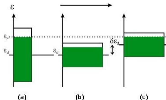
Figure 1- 4 Illustration of the effect of tensile strain on the d band centre (25).
