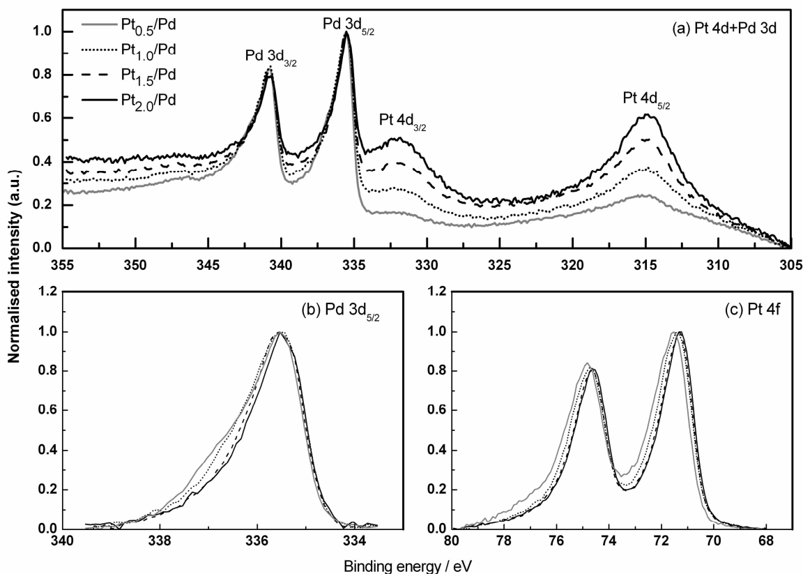
Figure 4- 8 Intensity normalised (a) Pt 4d and Pd 3d and (b) Pd 3d and (c) Pt 4f (background subtracted) XPS spectra for Pt 1.0 /Pd, Pt 1.5 /Pd, Pt 2.0 /Pd.
