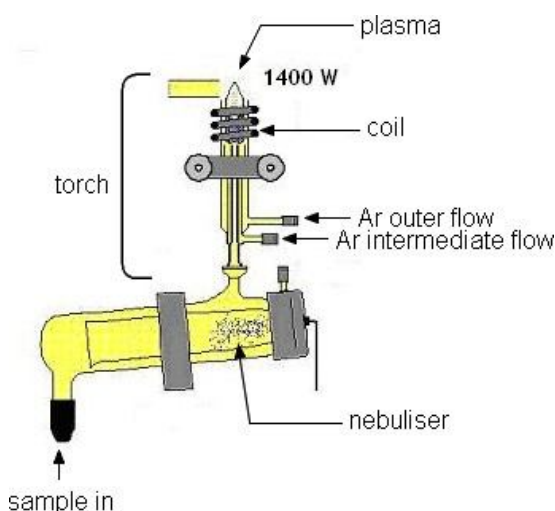
Figure 2- 7 Scheme of an ICP source.
