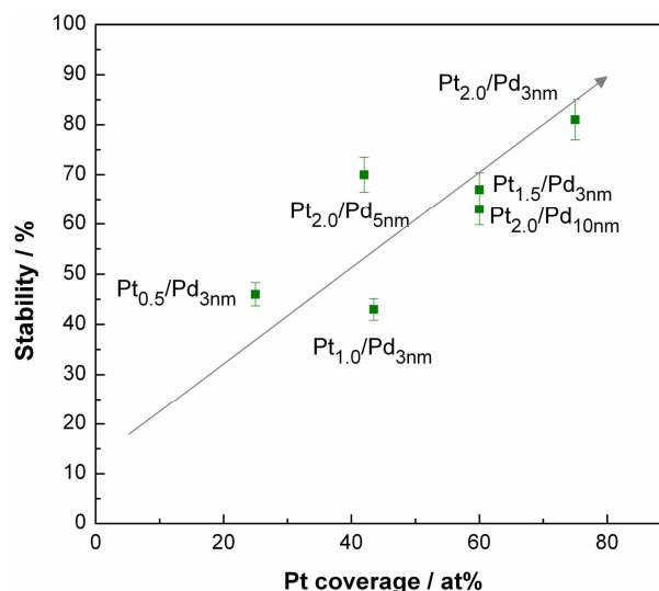
Figure 7- 1 Correlation between the core-shell electrocatalyst stability and their XPS-deduced Pt atomic composition. The stability is defined as the retained active area after 1000 cycles between 0.6 and 1.0 V at 80 °C in 1 M H 2 SO 4 .
