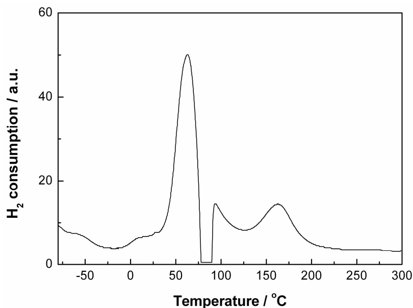
Figure 3 - 2 H 2 -TPR 20%Pd/C.
