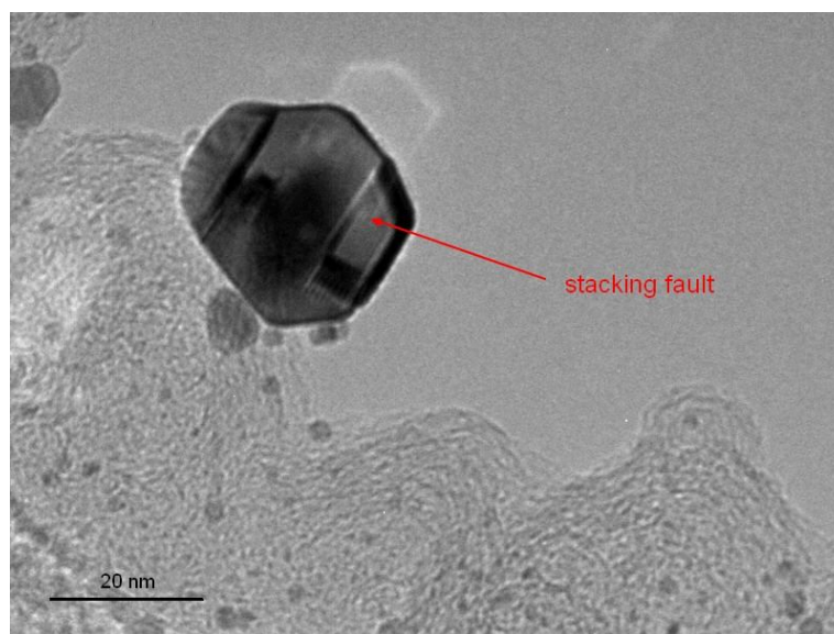
Figure 6 - 3 HRTEM micrographs of 38% Ir/C particles showing a stacking fault.
