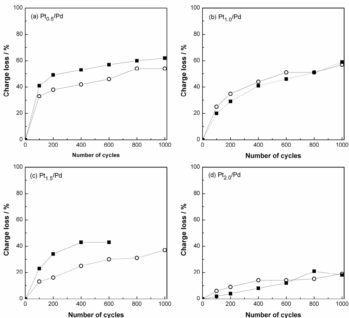
Figure 4- 16 Evolution of H and CO charges as a function of the number of polarisation scans for Pt_{0.5}/Pd (a), Pt_{1.0}/Pd (b), Pt_{1.5}/Pd (c) and Pt_{2.0}/Pd (d).
