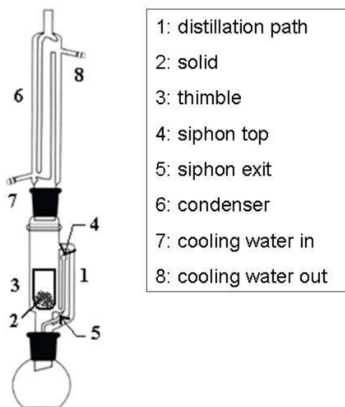
Figure 2- 1 A schematic representation of a Soxhlet extractor.
