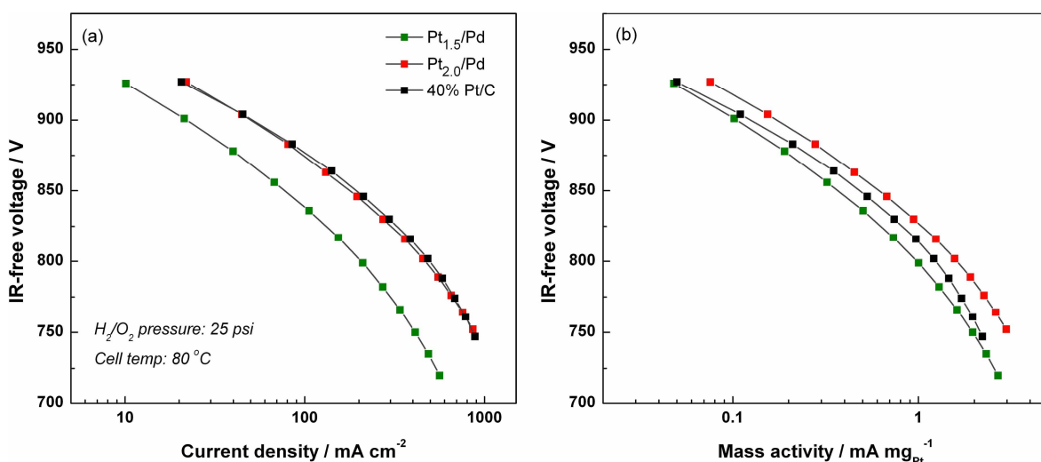
Figure 4- 20 Performances of MEAs prepared with Pt_{1.5}/Pd ( 0.21 \text{ mgPt cm}^{-2} ), Pt_{2.0}/Pd ( 0.29 \text{ mgPt cm}^{-2} ) and 40%Pt/C ( 0.4 \text{ mgPt cm}^{-2} ) as the cathode catalysts, in H_2/O_2 single cell. The results are presented as cell voltage corrected for the IR drop versus the current density (a) and the Pt-mass activity (b).
