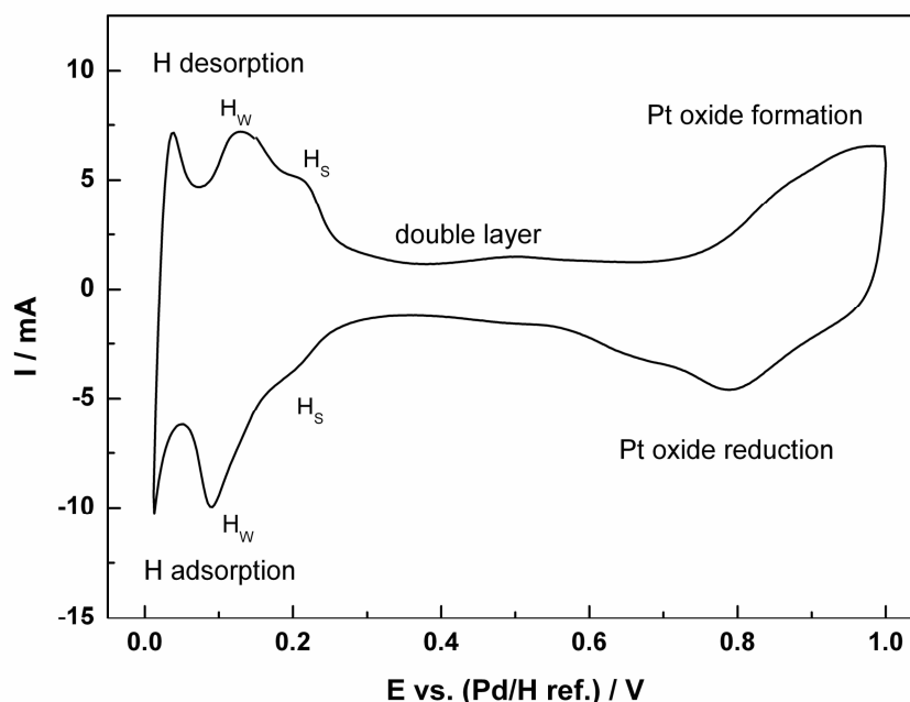
Figure 4- 9 Cyclic voltammogram of 40% Pt/C ( 0.4 \text{ mgPt}/\text{cm}^2 ) in 1 \text{ M H}_2\text{SO}_4 , 80^\circ\text{C} .
