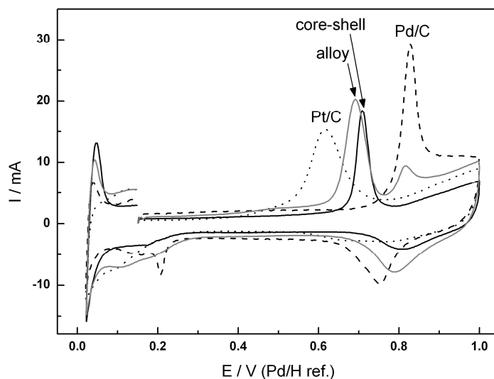
Figure 3 - 17 CV of carbon-supported Pt (dotted line), \text{Pt}_{26}\text{Pd}_{74}/\text{C} core-shell (dark grey line), \text{Pt}_{26}\text{Pd}_{74}/\text{C} alloy (light grey line) and Pd (dashed line), after CO saturation, in 1 M \text{H}_2\text{SO}_4 at 80 °C. Scanning rate 10 \text{ mV s}^{-1} , 0.01 - 1.0 V (Pd/H ref.).
