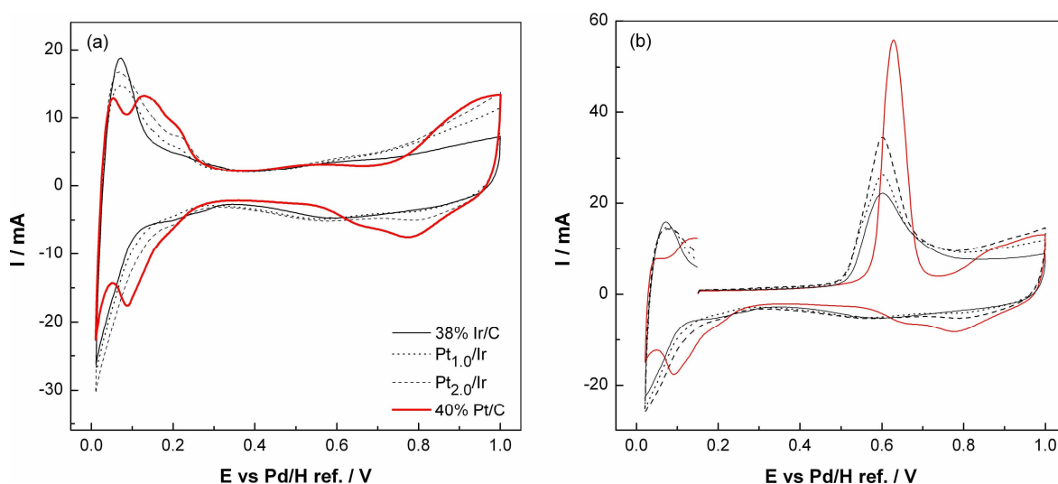
Figure 6 - 11 Cyclic voltammograms of the Pt_{1.0}/Ir , the Pt_{2.0}/Ir , 40%Pt/C and 38% Ir/C catalysts in 1 M H_2SO_4 at 80^\circ C , 10\text{ mV s}^{-1} .
