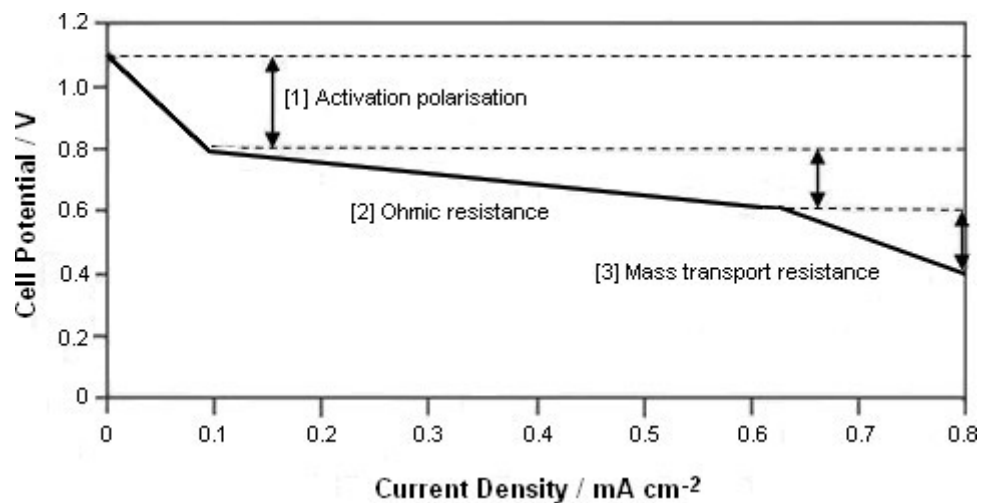
Figure 1- 2 Typical PEM Fuel Cell polarisation curve.
