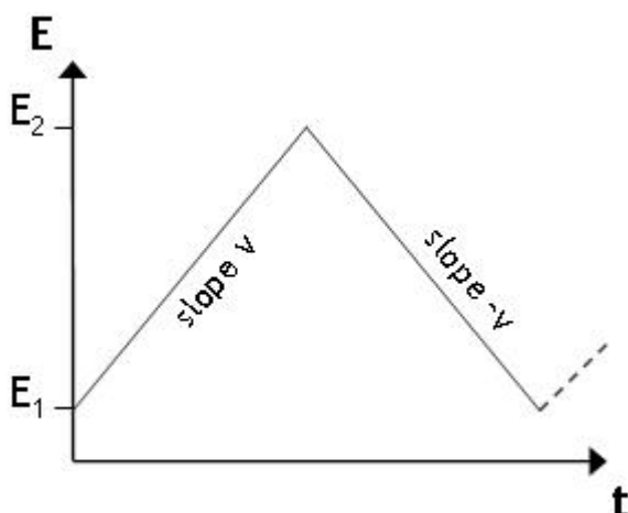
Figure 2- 14 Potential - time profile used in cyclic voltammetry
