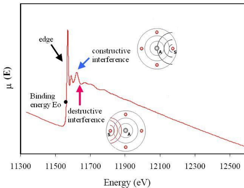
Figure 2- 9 EXAFS spectrum for an atomic species. The constructive interference corresponds to a maxima, whereas a destructive interference corresponds to minima in the EXAFS plot. They are represented by the interference between the waves coming from the absorbing atom (A) and the scattering atom (S).
