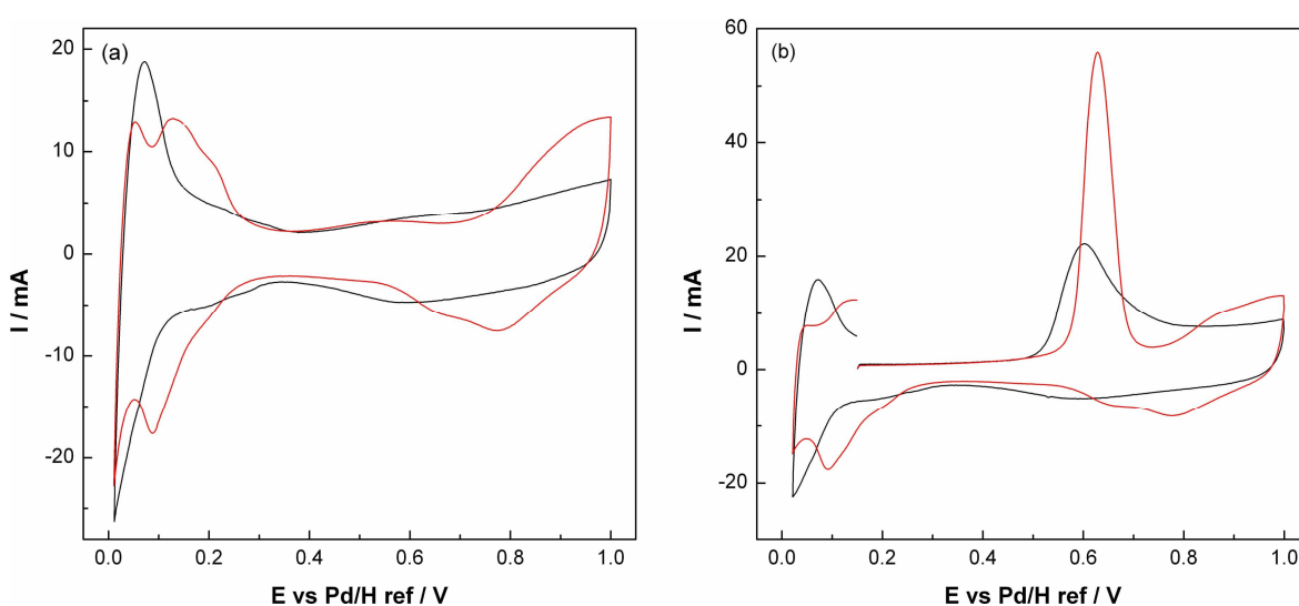
Figure 6 - 9 (a) Cyclic voltammograms and (b) CO electrooxidation voltammograms of 38%Ir/C (black line) and 40%Pt/C (red line) in 1 M H_2SO_4 , at 10 mV/s at 80°C. Electrode area: 3.14 cm 2
