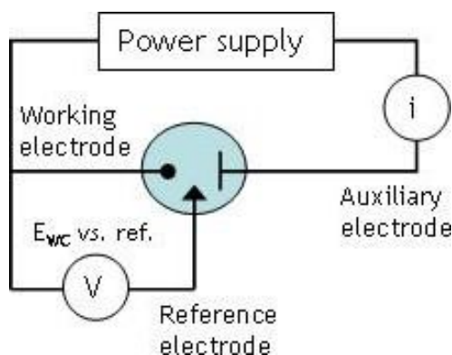
Figure 2- 13 Electrical circuit for a three-electrode cell
