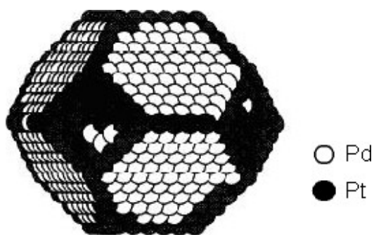
Figure 3 - 14 Representation of a cubooctahedral Pd particle covered with Pt only at the corners and edges.
