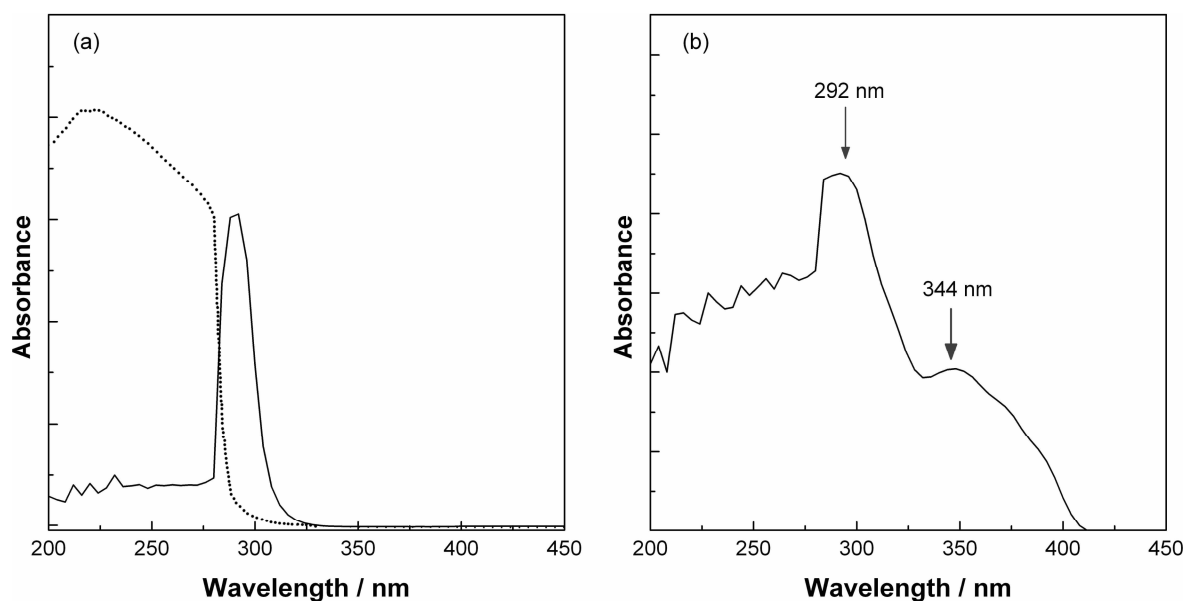
Figure 3 - 5 UV spectra for (a) toluene (dotted line) and acetylacetone diluted in toluene (solid line) and (b) for Pt(acac) 2 dissolved in toluene.
