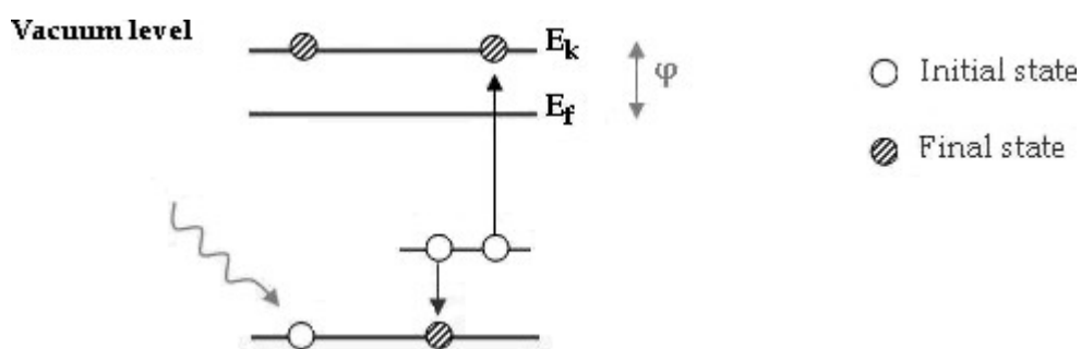
Figure 2- 6 XPS emission processes for a model atom
