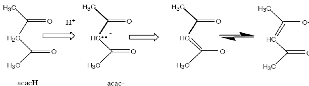
Figure 2- 2 In the presence of base, acetylacetone (acacH), readily loses a proton to form the acetylacetonate anion, acac.
