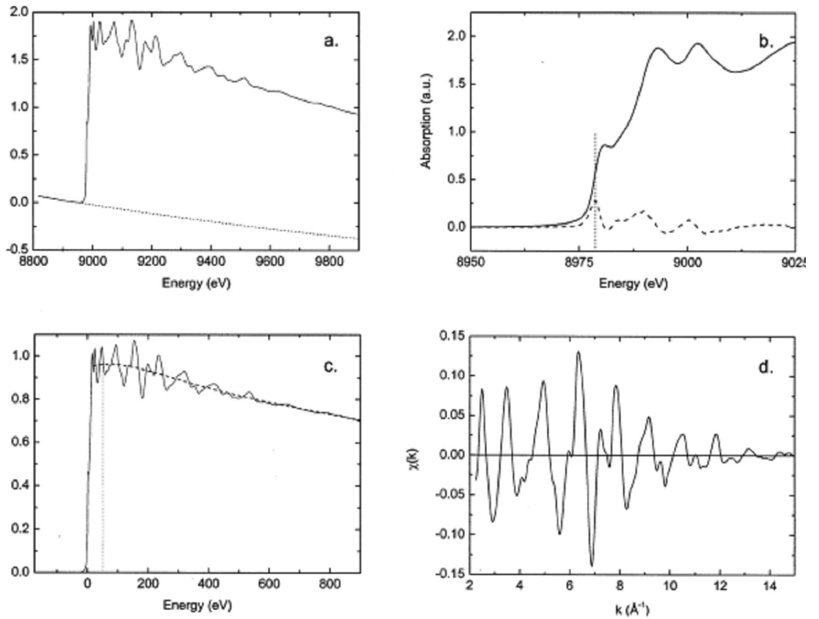
Figure 2- 10 EXAFS data analysis scheme. (a) Subtraction of Pre-edge. (b) Determination of the absorption edge. (c) Subtraction of the background and normalisation. (d) Produced EXAFS data.
