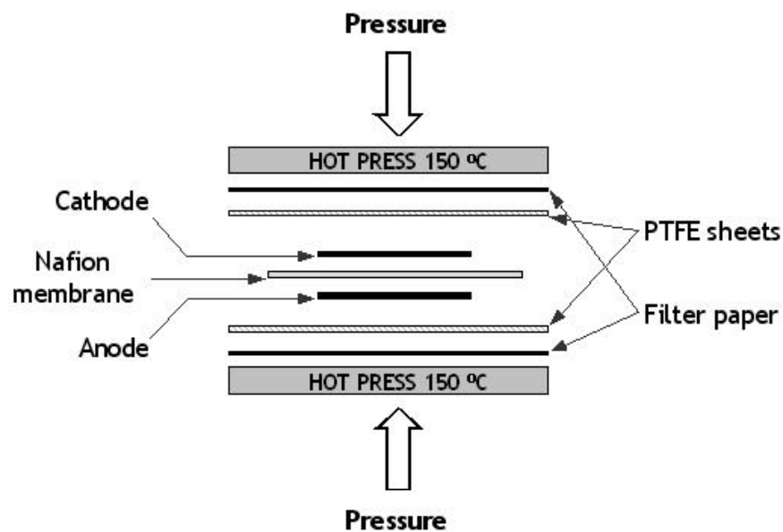
Figure 2- 18 Arrangement used for hot pressing MEAs.
