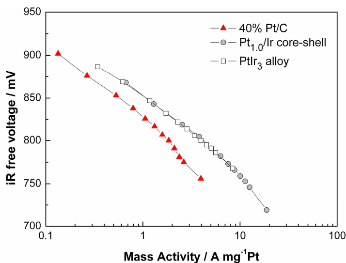
Figure 6 - 16 H_2/O_2 corrected performance of Pt_{1.0}/Ir , PtIr_3 alloy, and 40% Pt in 49 \text{ cm}^2 hardware at 50 \text{ kPa}_{\text{gauge}} at 80^\circ\text{C} , 100\% RH_{\text{anode/cathode}} (relative humidity)
