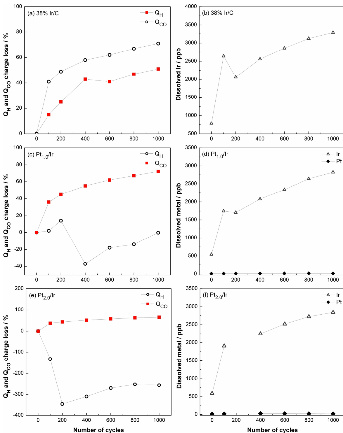
Figure 6 - 13 Change in Q_H and Q_{CO} charges (a, c and e) and in the amount of dissolved Pt and Ir (b, d and f) during the cycling test for 38% Ir/C, Pt_{1.0}/Ir and Pt_{2.0}/Ir .
