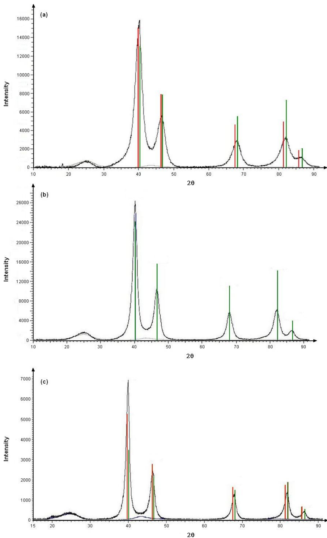
Figure 5- 6 XRD patterns of Pt_{2.0}/Pd_{3nm} (a), Pt_{2.0}/Pd_{5nm} (b) and Pt_{2.0}/Pd_{10nm} (c). The vertical lines represent the documented diffraction peaks of Palladium (in green) and Platinum (in red).
