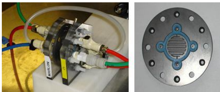
Figure 2- 19 Miniature PEMFC on the left. Graphite plate current collector on the right.
