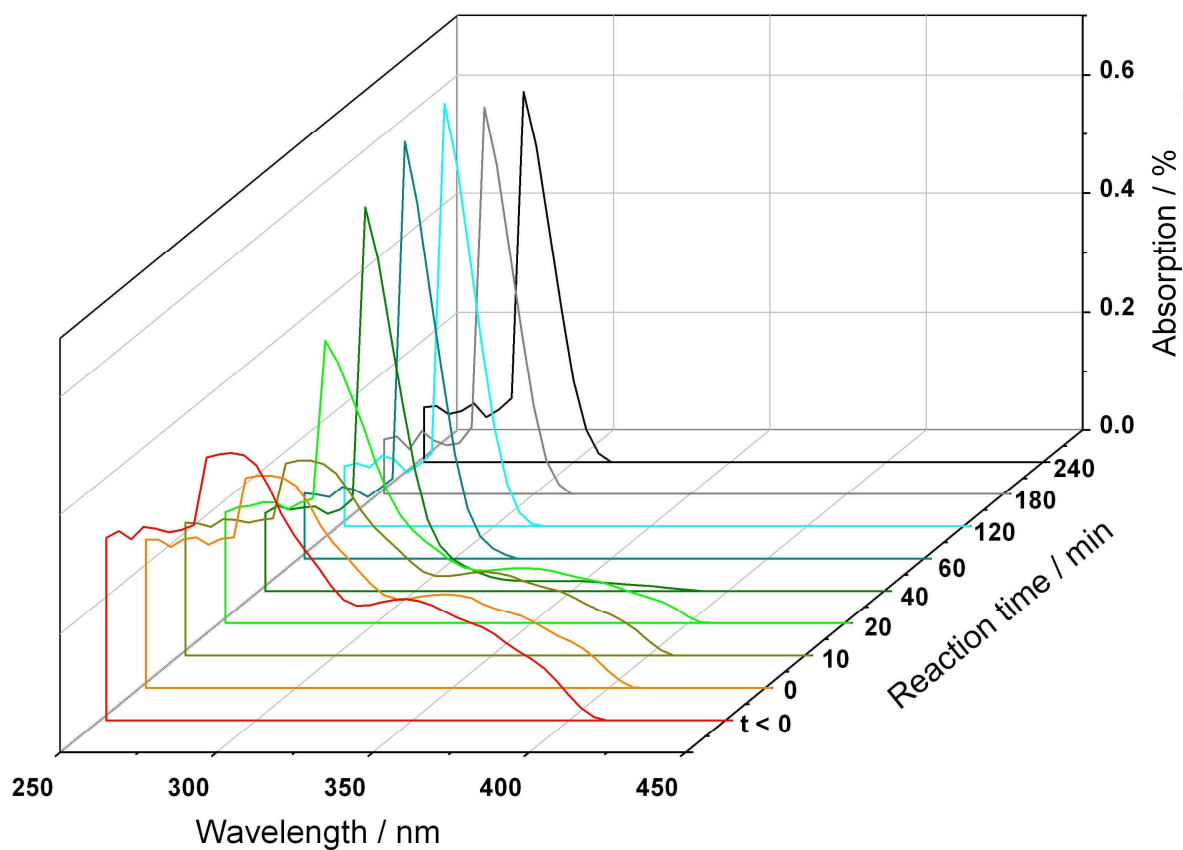
Figure 3 - 6 UV spectra following the CSR reaction between Pd/C and Pt(acac) 2 as a function of time.
