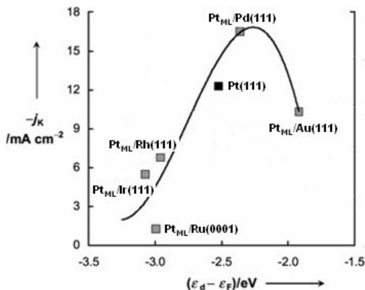
Figure 1- 5 Kinetic current densities ( j_K ) at 0.8 V for O_2 reduction on the Pt monolayers supported on different crystals in a 0.1M HClO_4 solution as functions of calculated d-band centre ( \epsilon_d - \epsilon_F ; relative to the Fermi level) of the respective clean Pt monolayers (14).
