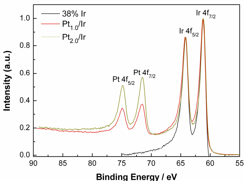
Figure 6 - 8 Normalised Pt 4f and Ir 4f XPS spectra for 38% Ir/C, Pt 1.0 /Ir and Pt 2.0 /Ir catalysts.
