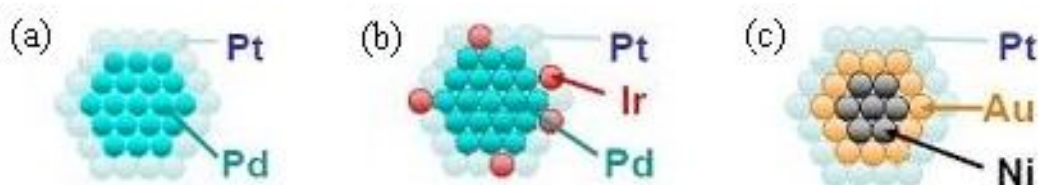
Figure 1- 6 Core-shell structures. (a) Pt monolayer on a Pd core (b) Mixed-metal Pt and Ir monolayer on a Pd core (c) Pt monolayer on a noble/non-noble core-shell nanoparticles (35).
