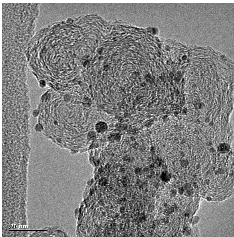
Figure 5- 1 TEM micrograph of carbon-supported Pd 3nm . Scale bar: 20 nm.
