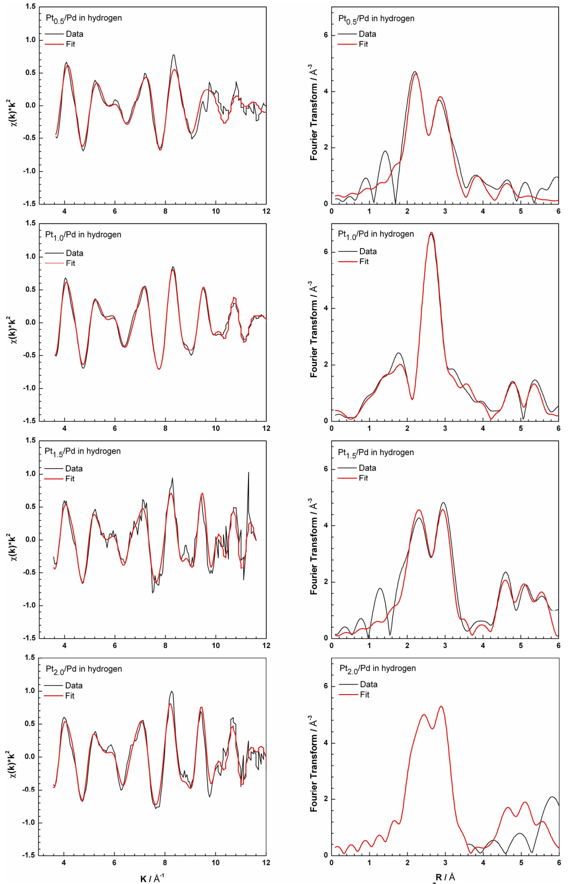
Figure 4- 3 EEXAFS plots for Pt_{0.5}/Pd , Pt_{1.0}/Pd , Pt_{1.5}/Pd , Pt_{2.0}/Pd . (left) k^2 -weighed \chi(k) spectrum collected at Pt L_{III} edge obtained in hydrogen; (right) k^2 -weighed Fourier transform of the \chi(k) data.
