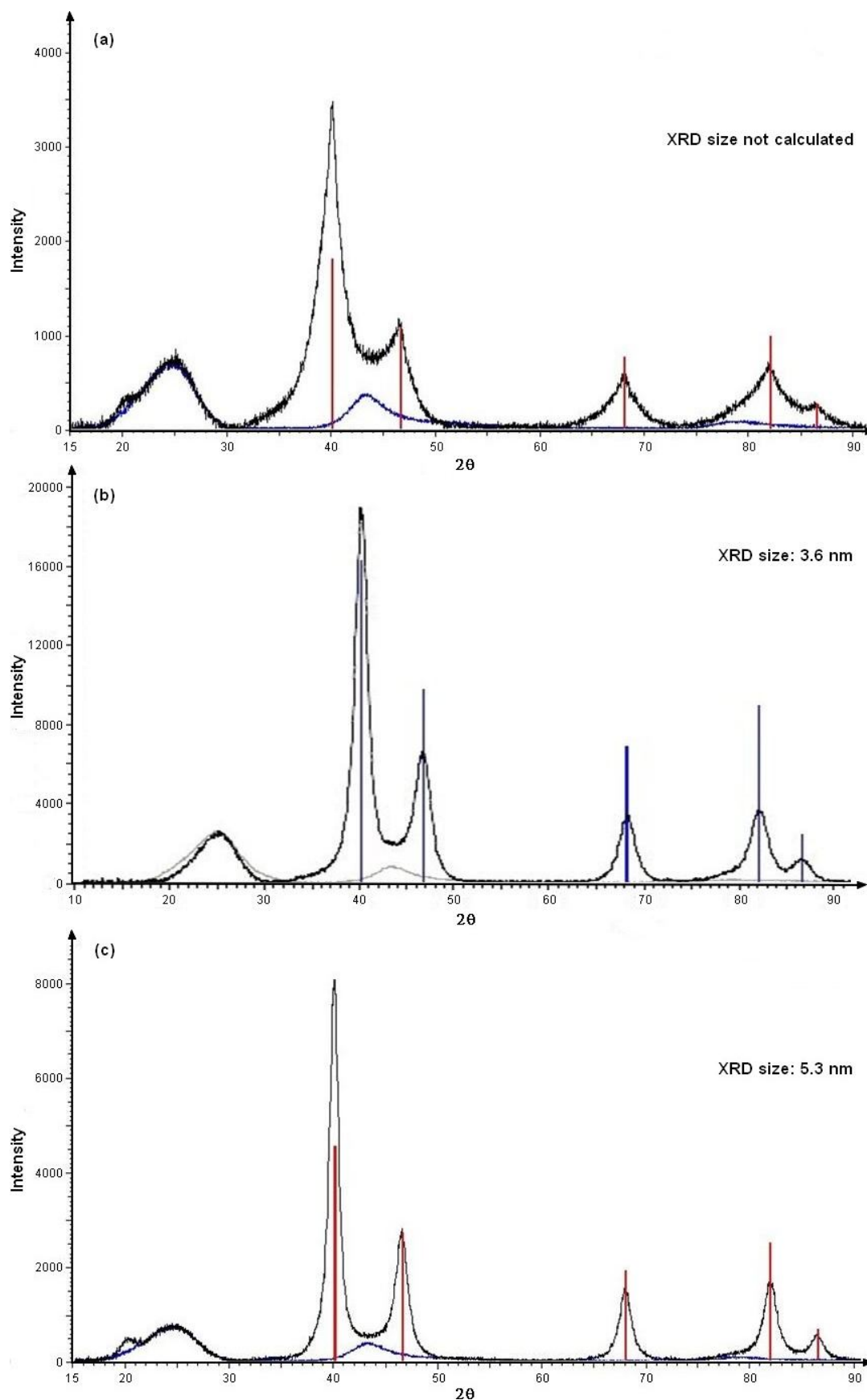
Figure 5- 5 XRD patterns of Pd_{3nm} (a), Pd_{5nm} (b) and Pd_{10nm} (c). The vertical lines represent the documented diffraction peaks of Palladium and the blue pattern represents the carbon contribution.
