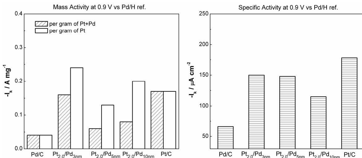
Figure 5- 22 Relationship between the Pt coverage and the ORR mass activity (a) and specific activity (b) at 0.9 V vs Pd/H ref. determined by analysis of the polarisation curves reported in Figure 5-21(a).
