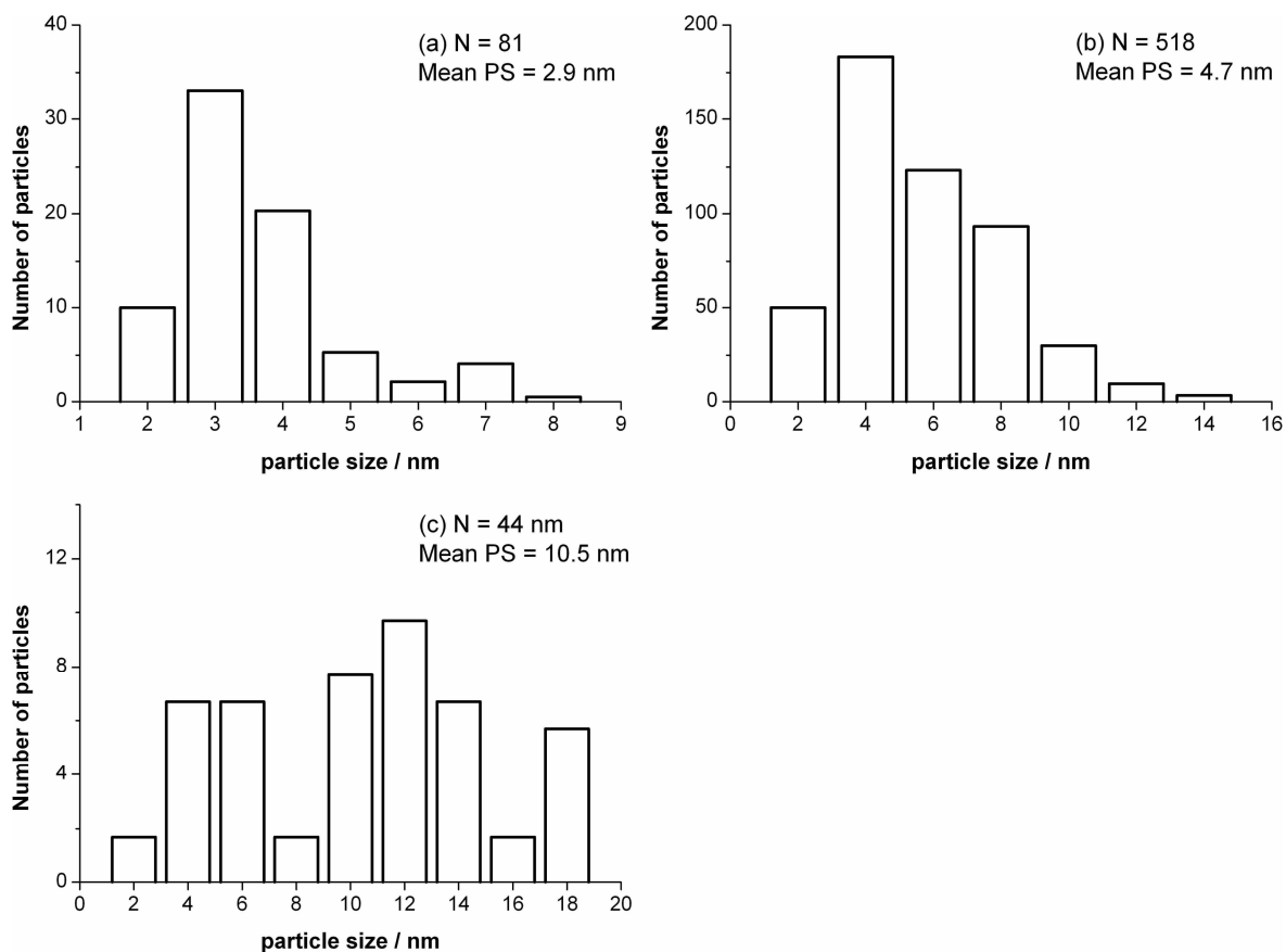
Figure 5- 4 Particle size distribution bar charts for Pd 3nm (a), Pd 5nm (b) and Pd 10nm (c).
