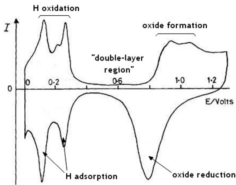
Figure 2- 15 Cyclic voltammogram of a Pt electrode in 0.5 M \text{H}_2\text{SO}_4 at 25 °C at 100 \text{mV s}^{-1}
