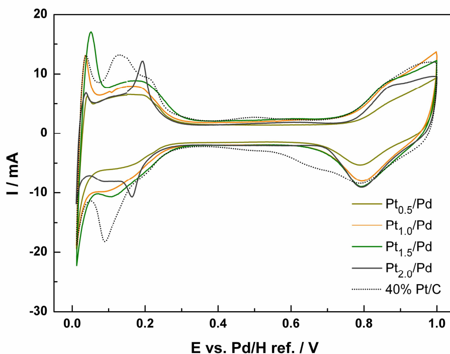
Figure 4- 11 Cyclic voltammogram of Pt/Pd/C core-shell painted button electrodes (0.6 mg carbon/cm 2 ) in 1 M H 2 SO 4 , at 10 mV/s at 80°C. Electrode area: 3.14 cm 2 .
