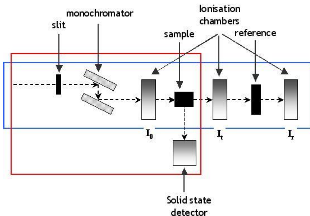
Figure 2- 11 Scheme of the set-ups for the transmission detection mode (inside blue rectangle) and for the fluorescence detection mode (inside red rectangle). The dashed line represents the pathway of the beam.
