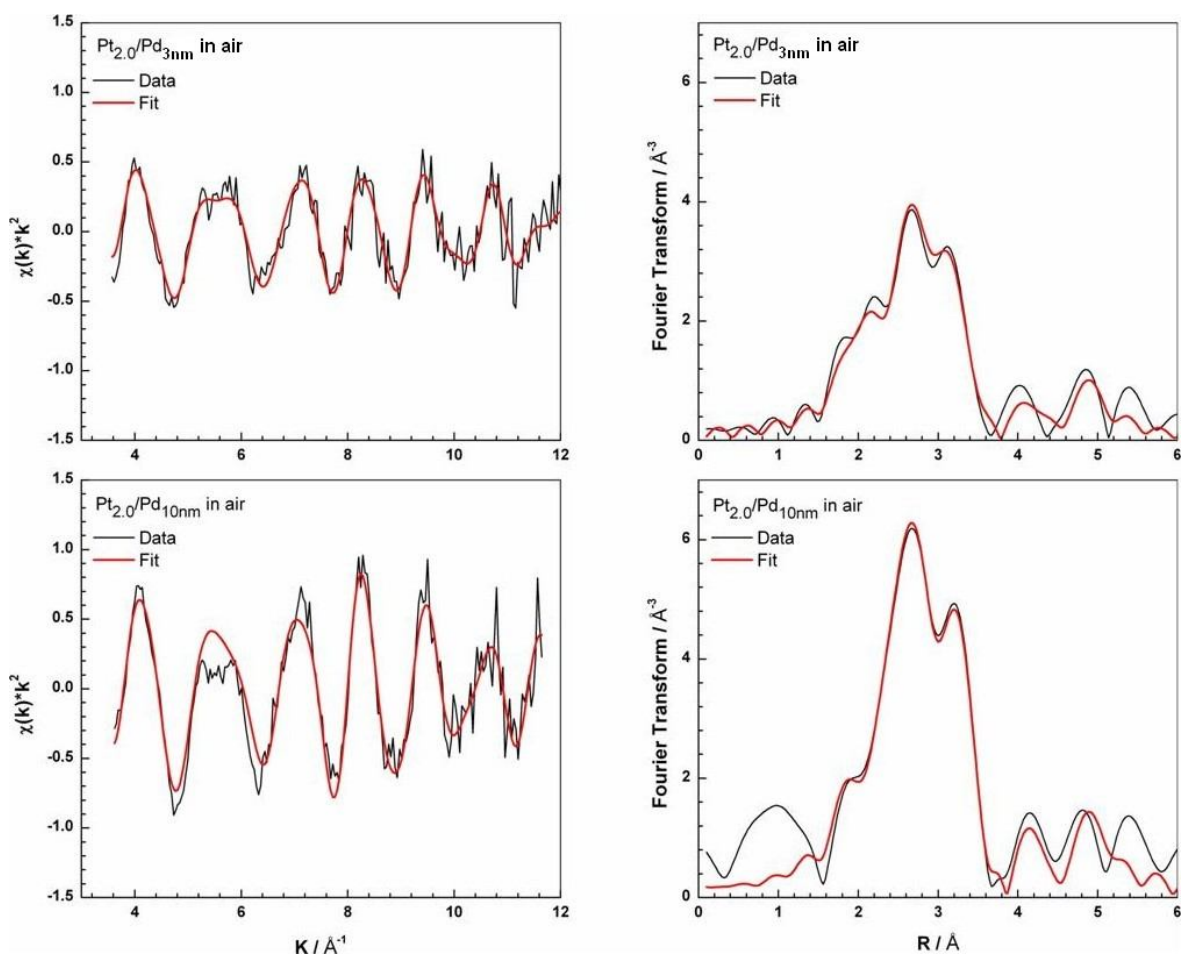
Figure 5- 8 EXAFS plots for Pt_{2.0}/Pd_{3nm} , Pt_{2.0}/Pd_{5nm} and Pt_{2.0}/Pd_{10nm} . (left) k^2 -weighed \chi(k) spectra collected at Pt L_{III} edge in air; (right) k^2 -weighed Fourier transforms of the \chi(k) data.
