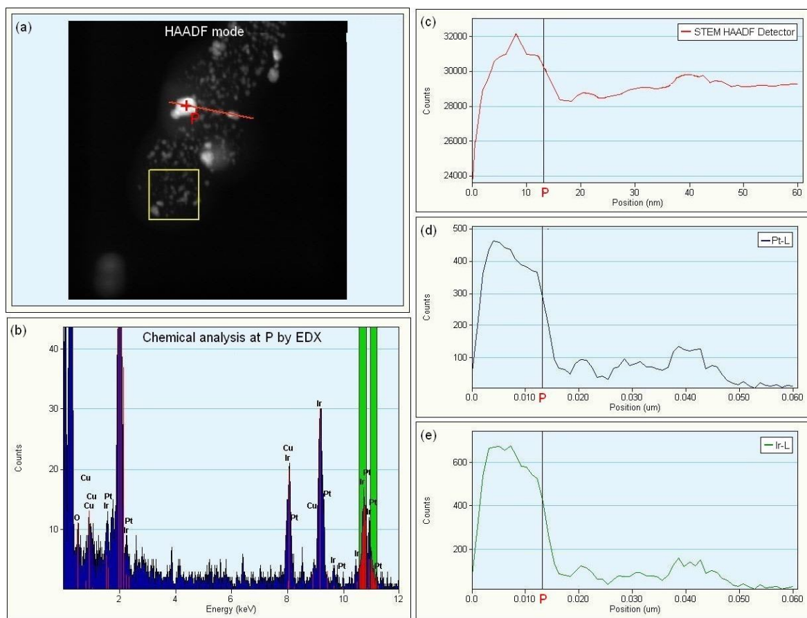
Figure 6 - 6 HRTEM micrographs of Pt_{2.0}/Ir particles in HAADF mode (a). Chemical analysis at position P (b). EDX total count profile across two core-shell particles following the red line in picture a (c). EDX Pt profile (d). EDX Ir profile (e).
