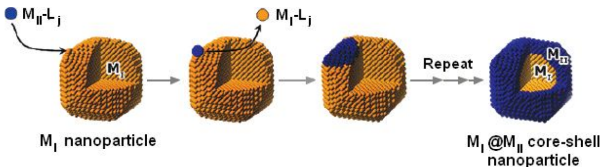
Figure 1- 7 Metal ions of reactant metal complexes ( M_{II}-L_j ) are reduced on the surface of M_I core nanoparticles while M_I atoms are oxidised to M_I^+ by forming a M_I -ligand complex ( M_I-L_j ) (52).
