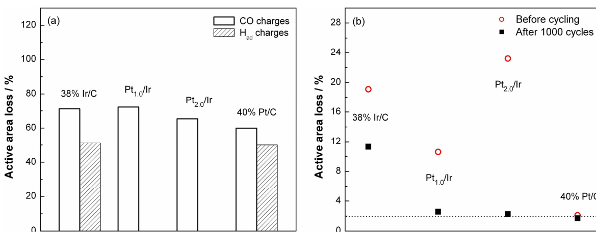
Figure 6 - 14 CO and H charge losses after 1000 cycles (a) and their ratios CO:H before and after 1000 cycles (b)
