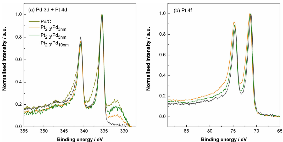
Figure 5- 14 Intensity normalised (a) Pt 4d and Pd 3d and (b) Pt 4f (Shirley-type background subtracted) XPS spectra for Pt_{2.0}/Pd_{3nm} , Pt_{2.0}/Pd_{5nm} , Pt_{2.0}/Pd_{10nm} .
