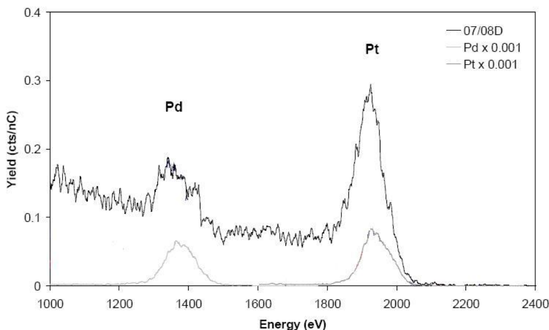
Figure 4- 7 The 3keV ^{20}Ne^+ spectrum of Pt_{2.0}/Pd after the reduction treatment, compared to the spectra for the Pd and Pt reference. The spectra for the references have been multiplied by 0.001 to facilitate comparison.
