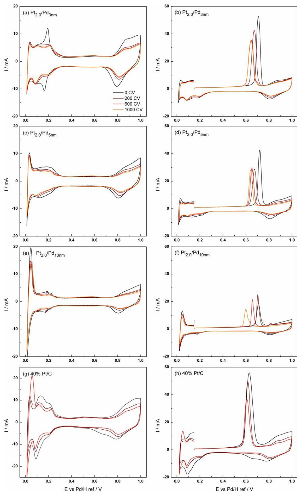
Figure 5- 16 CVs (on the left) and CO electrooxidation voltammograms (on the right) of Pt_{2.0}/Pd_{3nm} , Pt_{2.0}/Pd_{5nm} , Pt_{2.0}/Pd_{10nm} and 40%Pt/C recorded after 0, 200, 600 and 1000 polarisation scans (0.6-1.0 V) in 1 M H_2SO_4 , v = 10 \text{ mV s}^{-1} , at 80 °C.
