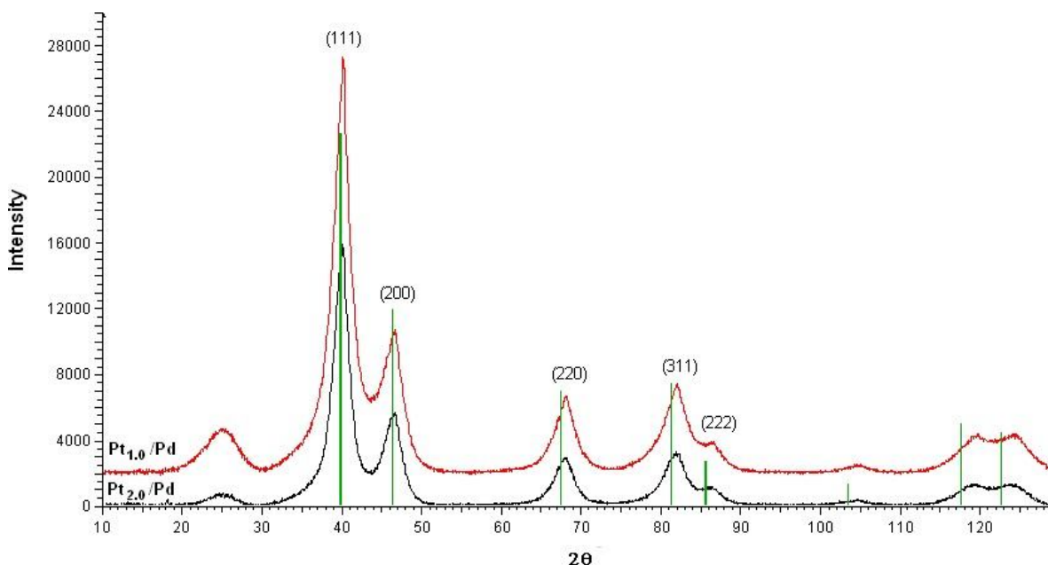
Figure 4- 1 XRD patterns of Pt_{1.0}/Pd (red spectrum) and Pt_{2.0}/Pd (black spectrum). The green vertical lines represent the documented diffraction peaks of Platinum.
