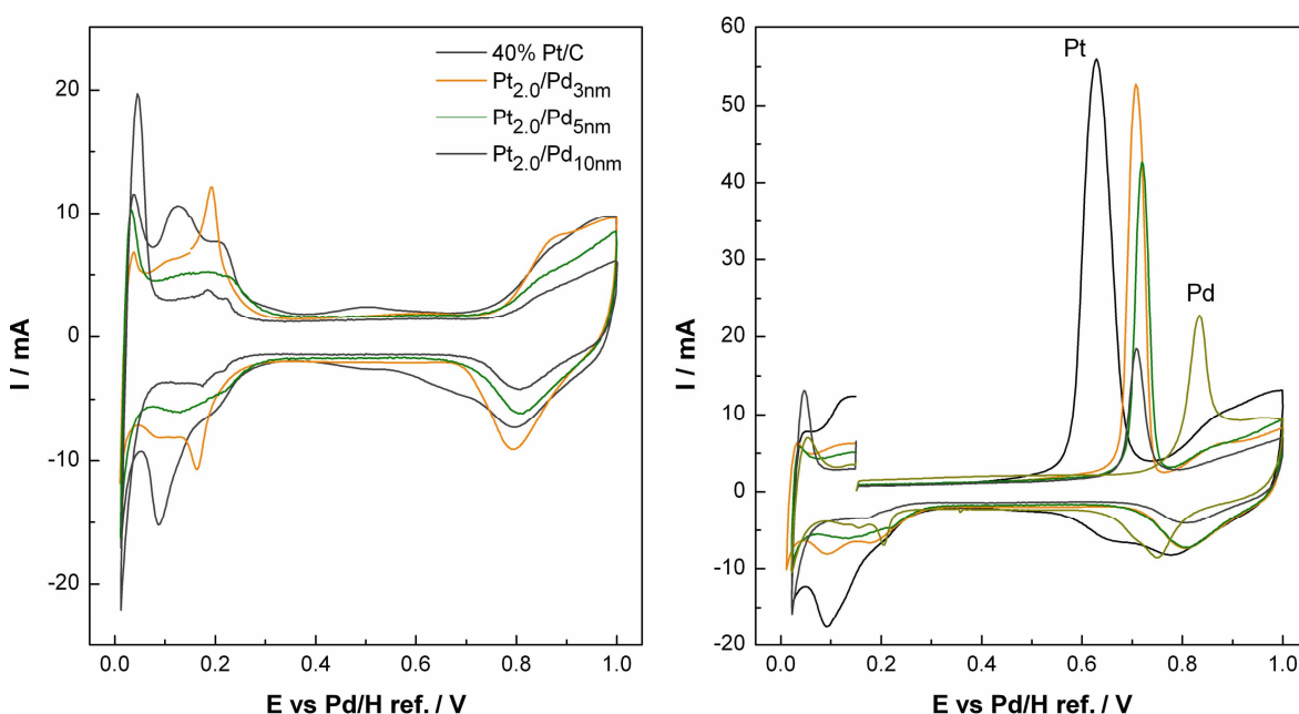
Figure 5- 15 Cyclic voltammograms of Pt_{2.0}/Pd core-shells and 40%Pt/C in 1 \text{ dm}^{-3} at 80^\circ\text{C} , 10 \text{ mV s}^{-1} .
