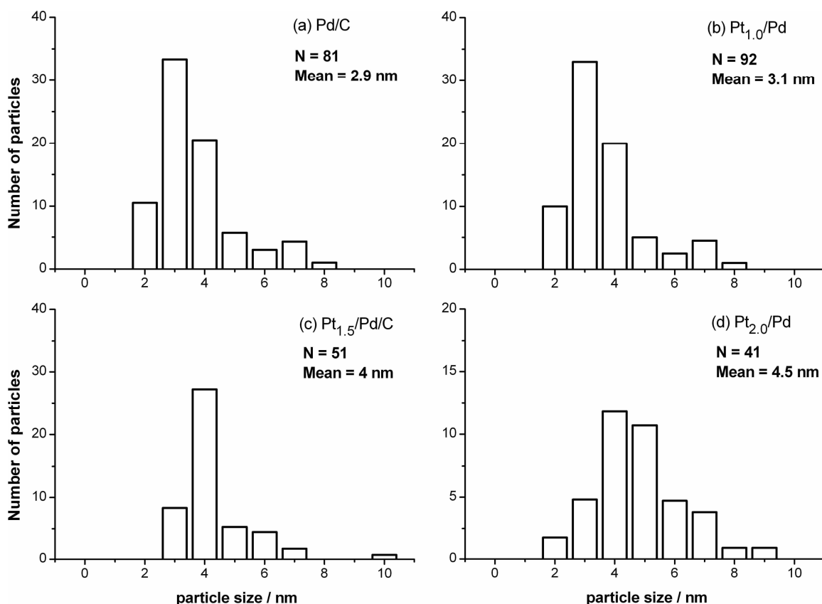
Figure 4- 5 Particle size distribution bar charts for (a) Pd/C, (b) Pt_{1.0}/Pd , (c) Pt_{1.5}/Pd and (d) Pt_{2.0}/Pd
