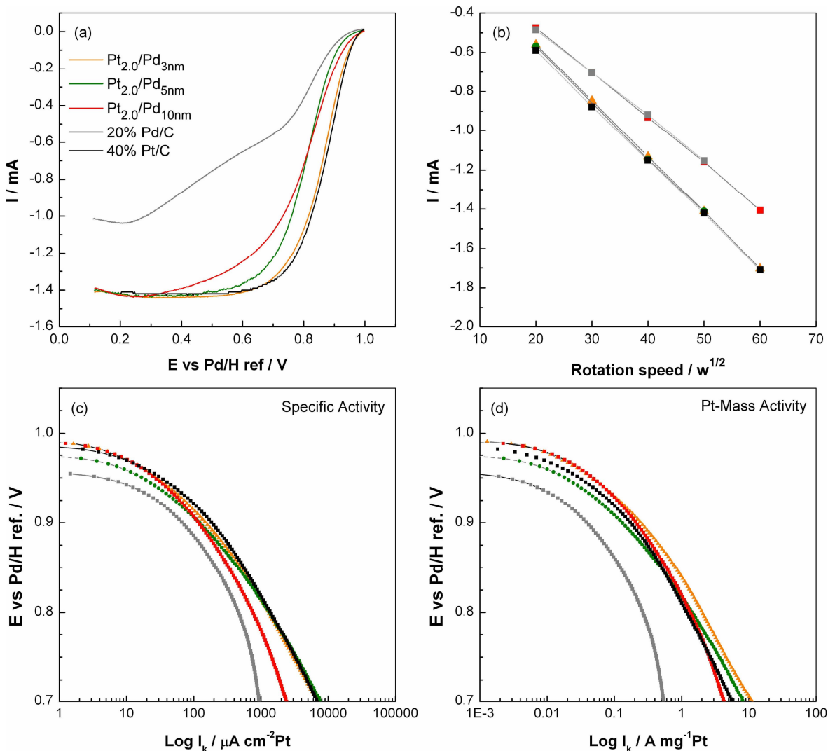
Figure 5- 21 Polarisation curves (backward scans) for the Pt_{2.0}/Pd core-shell, 20% Pd/C and 40% Pt/C electrocatalysts in 0.1 M HClO 4 . Scan rate of 10 mV s -1 . Levich plots (b). Tafel plots corrected for the electrochemical area (c) and for the Pt mass (d). Electrode geometric area: 0.196 cm 2 .
