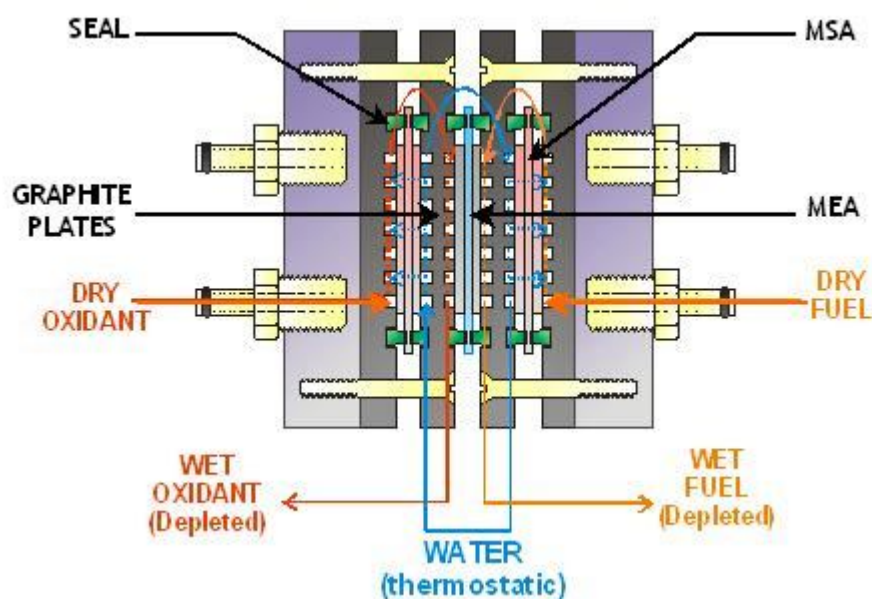
Figure 2- 20 Scheme of single cell PEM
