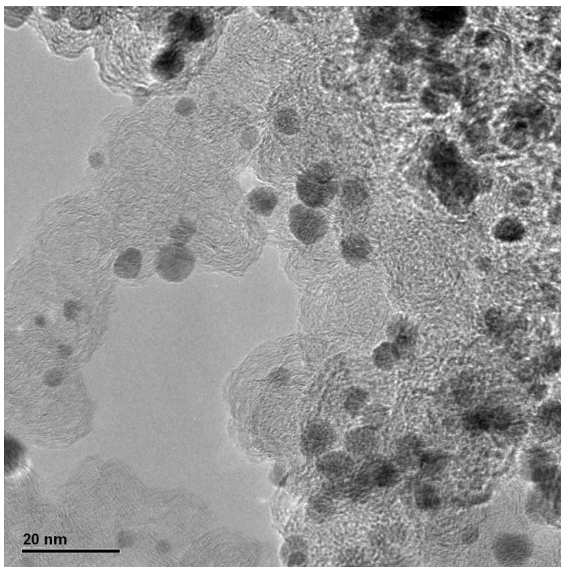
Figure 5- 2 TEM micrograph of carbon-supported Pd 5nm . Scale bar: 20 nm.
