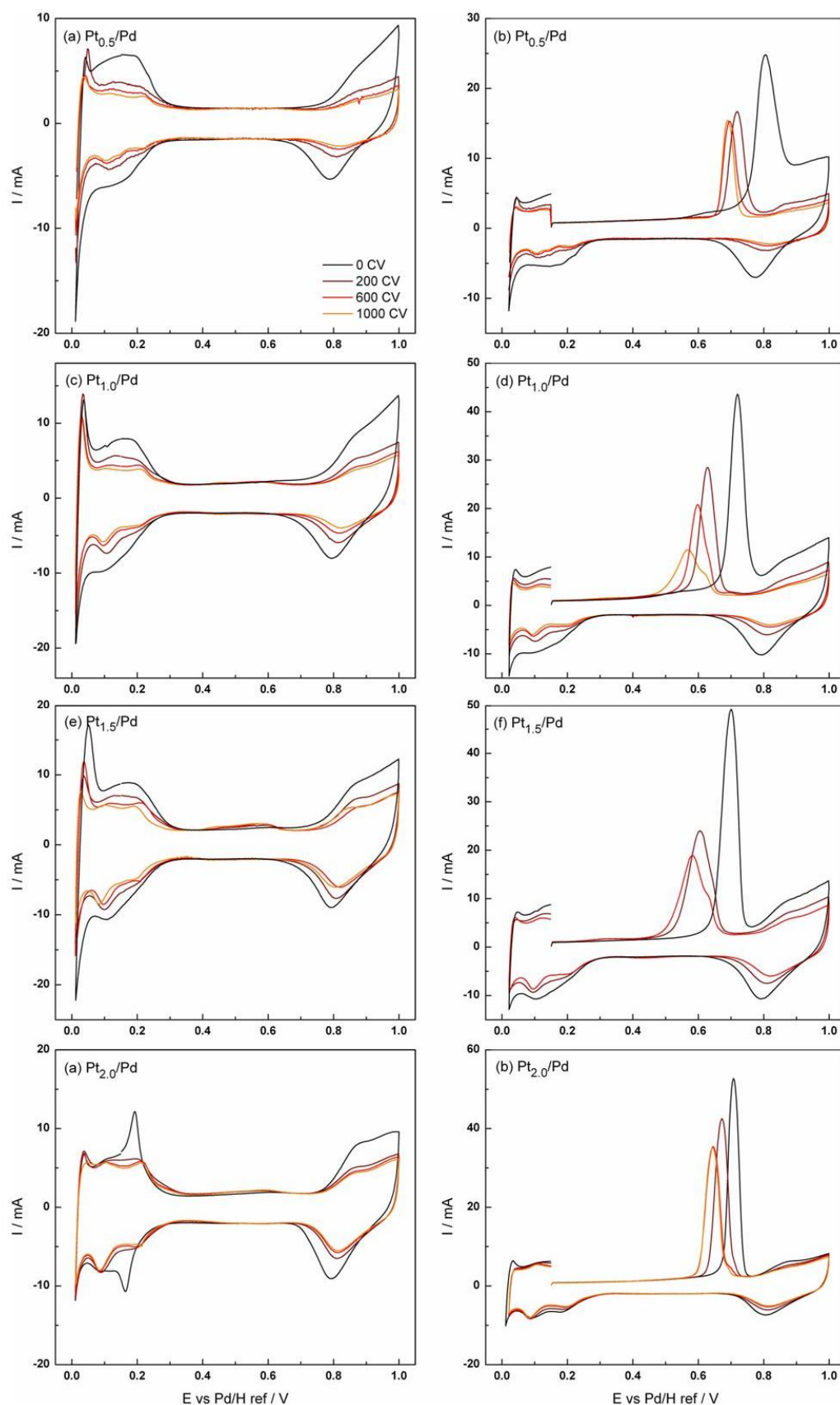
Figure 4-14 CV (on the left) and CO electrooxidation voltammograms (on the right) of Pt_{0.5}/Pd , Pt_{1.0}/Pd , Pt_{1.5}/Pd and Pt_{2.0}/Pd recorded after 0, 200, 600 and 1000 polarisation scans (0.6-1.0 V) in 1 M H_2SO_4 , v = 10 \text{ mV s}^{-1} , at 80^\circ\text{C} .
