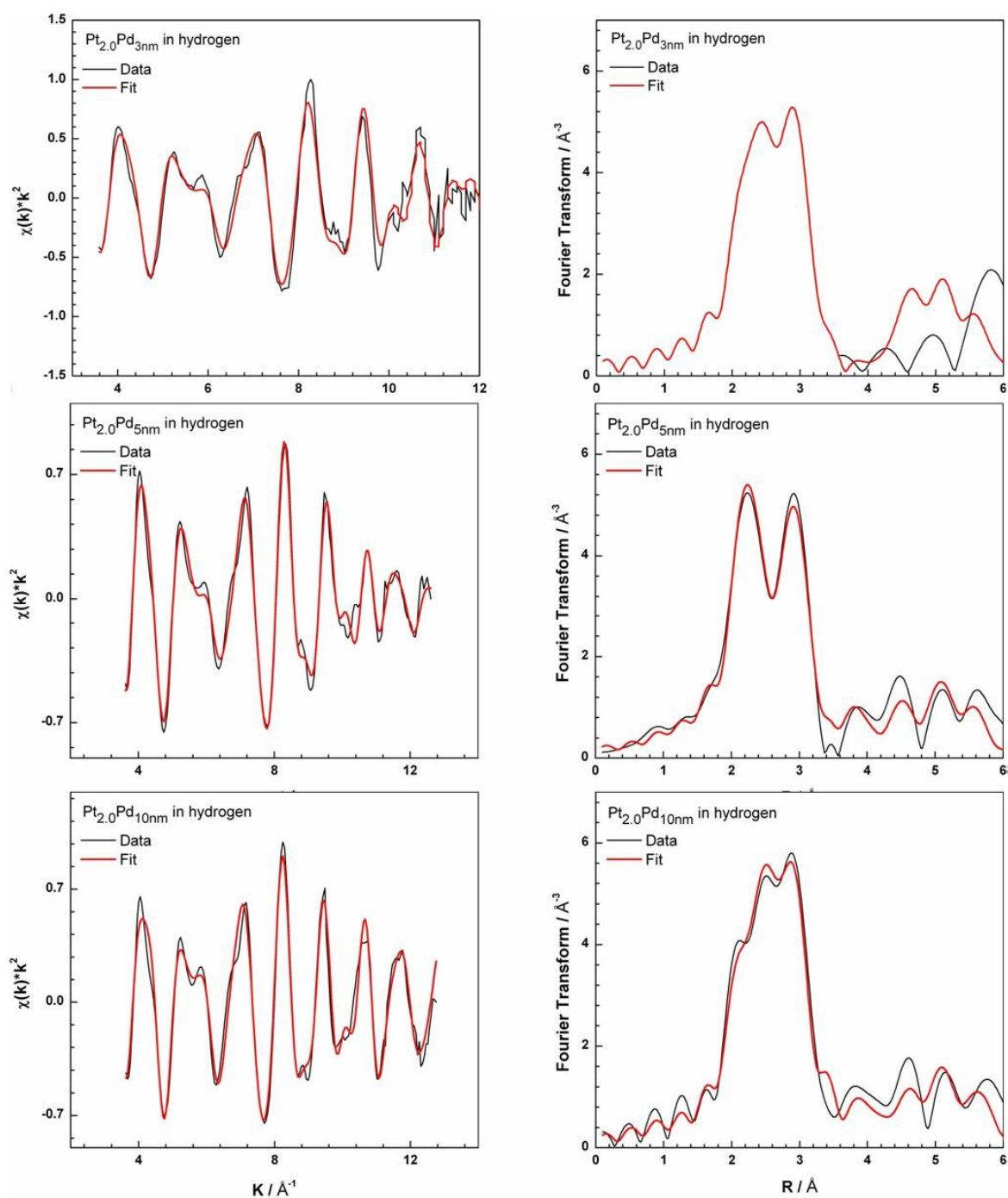
Figure 5- 7 EXAFS plots for Pt 2.0 /Pd 3nm , Pt 2.0 /Pd 5nm and Pt 2.0 /Pd 10nm . (left) k^2 -weighed \chi(k) spectra collected at Pt L III edge in hydrogen; (right) k^2 -weighed Fourier transforms of the \chi(k) data.
