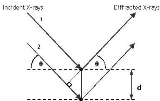
Figure 2- 5 Deriving Bragg's Law reflection geometry.
