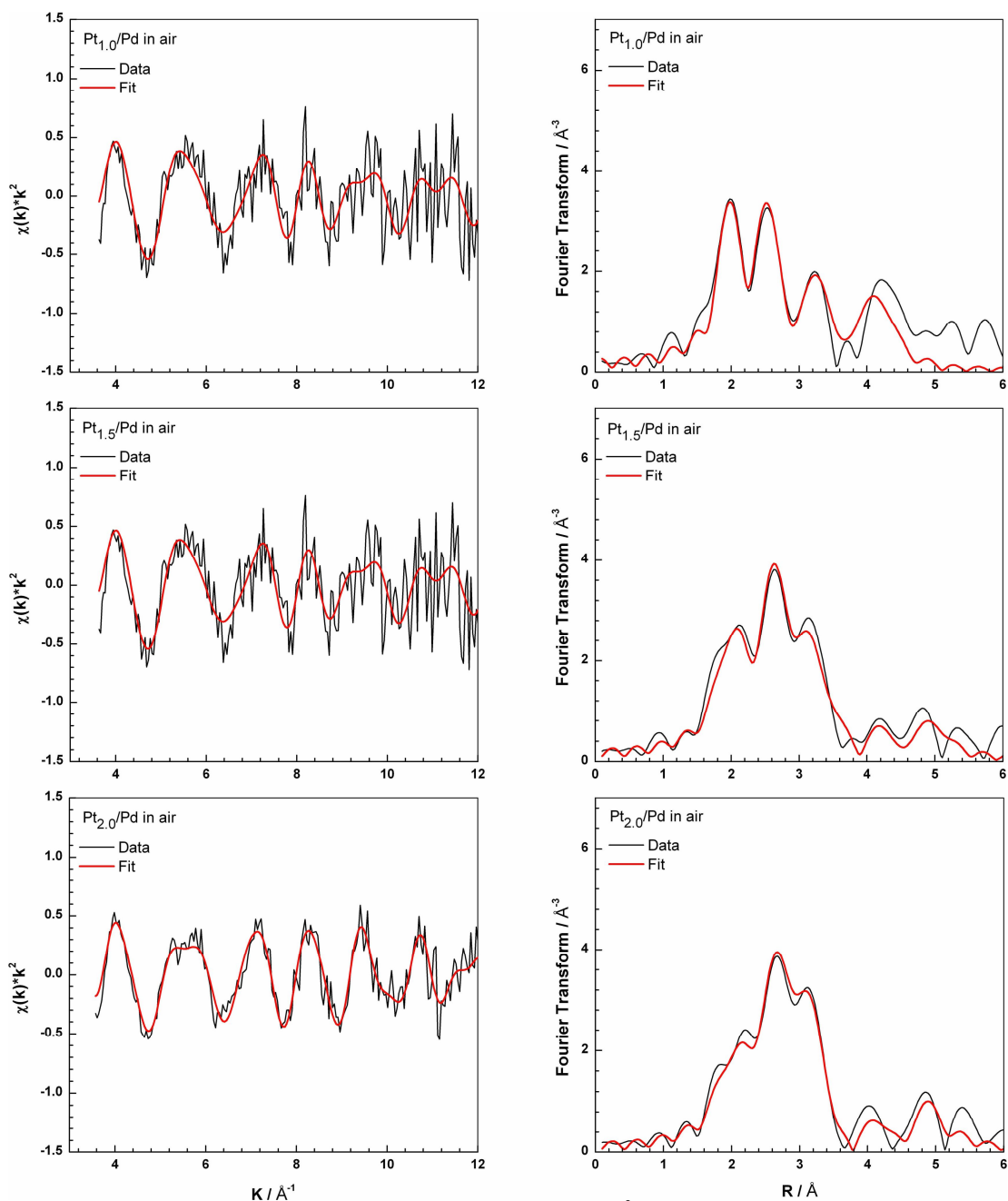
Figure 4- 4 EXAFS plots for Pt 1.0 /Pd, Pt 1.5 /Pd, Pt 2.0 /Pd. (left) k^2 -weighed \chi(k) spectrum collected at Pt L III edge obtained in air; (right) k^2 -weighed Fourier transform of the \chi(k) data.
