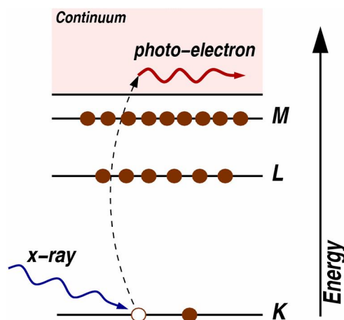
Figure 2- 8 Photoelectron emission mechanism
