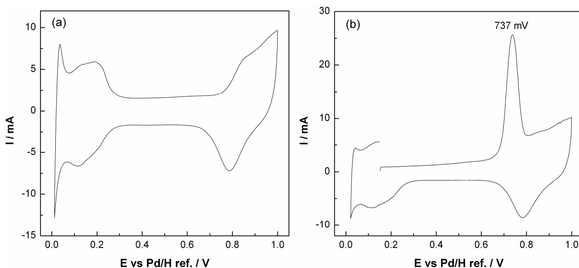
Figure 4- 12 Cyclic voltammogram (a) and CO electrooxidation voltammograms (b) of PtPd/C alloy painted button electrode in 1M H_2SO_4 , at 10 mV/s, at 80°C. Electrode area: 3.14 cm 2 .
