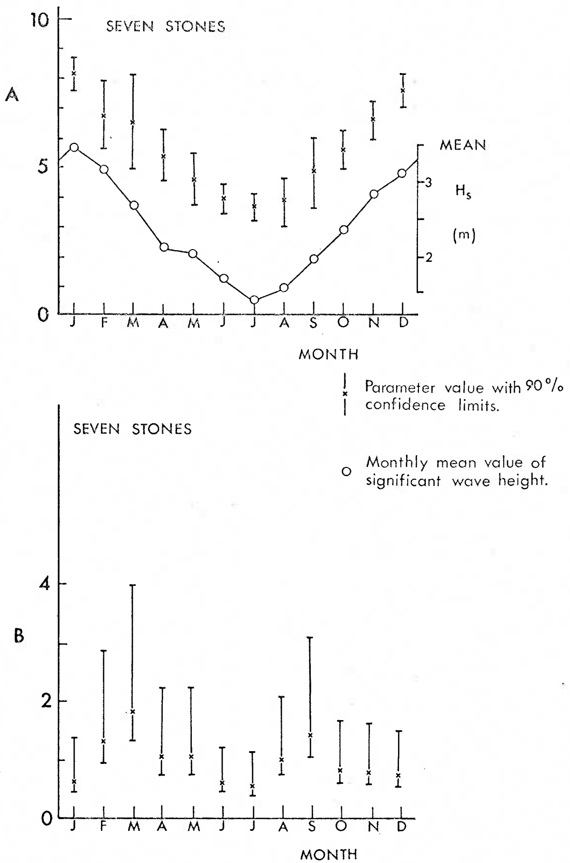
FIG. 5. Month-to-month variations in the value of the Fisher-Tippet Type I distribution parameters A & B defined by equation 1.
