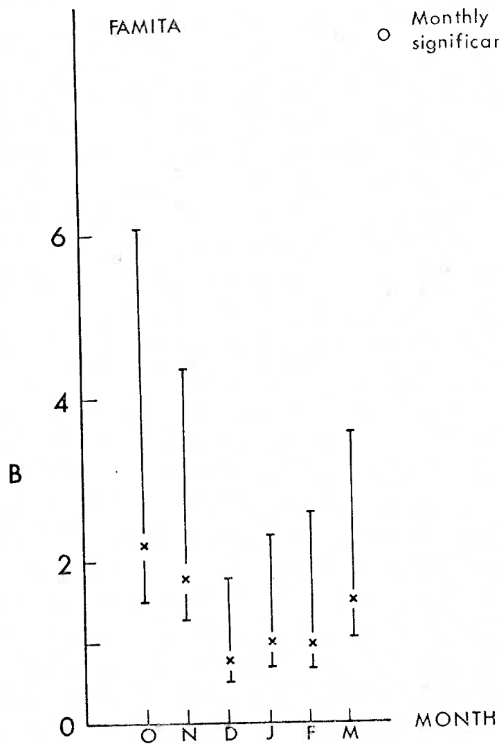
FIG. 6. Month-to-month variations in the values of the Fisher-Tippet Type I distribution parameters A & B defined by equation 1.
