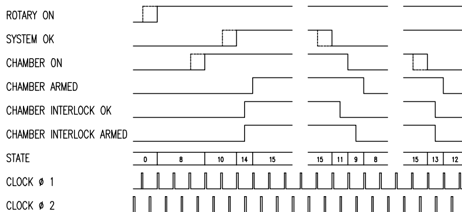
Figure 3. Timing diagram showing state machine operation via feedback. Only once normal running has been achieved may the monitor interlocks interrupt operation. All signals are shown at the latch outputs (as labelled in figure 2); ROTARY ON, CHAMBER ON and CHAMBER ARMED are inputs to the EPROM, while CHAMBER INTERLOCK OK and CHAMBER INTERLOCK ARMED are outputs. SYSTEM OK represents a combination of inputs, as explained in the text.
