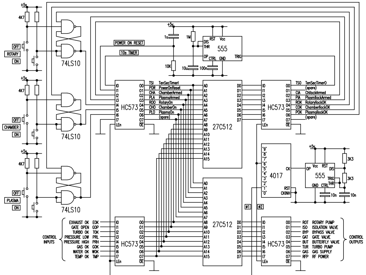
Figure 2. Schematic circuit diagram of the main controller logic. The circuit is based around a pair of EPROMs, with input and output latches driven in antiphase, which acts as a look-up table to convert inputs into output signals. Three inputs from user-set bistables and a fourth from a 10 second timer may be reset by the controller. Feedback from the outputs to the inputs allows internal states that correspond to data bits, allowing simple non-unitary processing.
