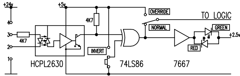
Figure 4. Generic input stage, allowing both logic level and contact closure signals of either polarity.
