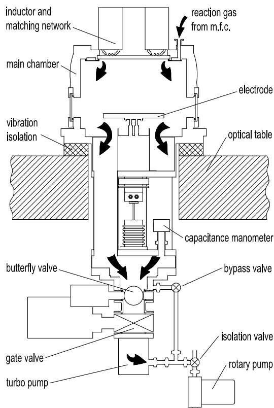
Figure 1. The inductively coupled radio-frequency plasma chamber and associated apparatus.
