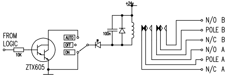
Figure 5. The output drives a DPDT relay, and may be manually overridden to be set either on or off. Operation is indicated by an LED.
