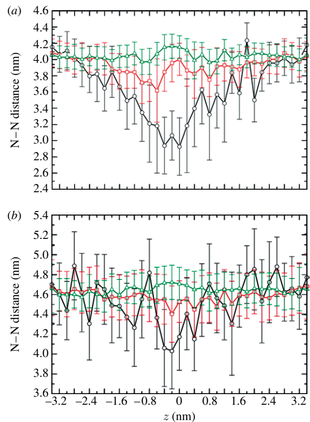
Figure 10. Local bilayer deformation of the bilayer for (a) DMTAP or (b) DPPC lipids as a function of z , indicated by the average distance (calculated over the final 5 ns of each umbrella sampling window production run) between upper- and lower-leaflet choline (N) particles ( d_{NN} ) within 0.5 (black), 1.5 (red) and 2.5 nm (green) of the DNA molecule's centre of mass. Error bars represent standard deviation over the 5 ns.
