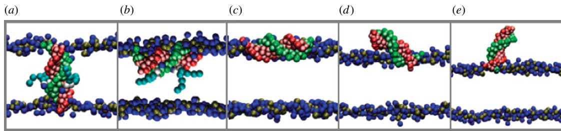
Figure 7. Representative simulation snapshots for different umbrella sampling windows, centred around z=(a) 0, (b) 1, (c) 2.4, (d) 3 and (e) 4 nm. The colour scheme for DNA is as in figure 4. The lipid DPPC and DMTAP headgroups are shown in space-filling format, with phosphate groups in brown and choline groups in blue. Selected DMTAP molecules whose headgroups have significantly penetrated the membrane core are shown in their entirety, with the glycerol backbone in white and lipid tails in cyan.
