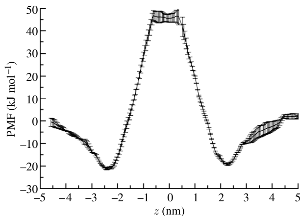
Figure 8. PMF for transfer of a DNA molecule across the normal ( z ) of a mixed DPPC/DMTAP bilayer and into the bulk solvent. Error bars represent the difference between PMFs calculated for the first and second halves of each simulation.
