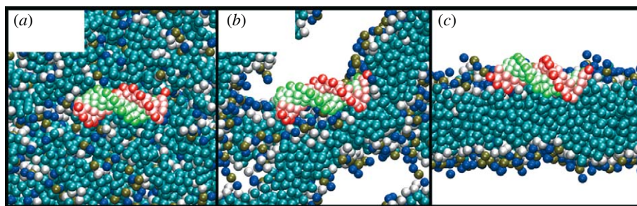
Figure 4. Space-filling representation of the formation of a lipid bilayer in the presence of a DNA molecule. (a) Randomly placed lipids around a DNA dodecamer (0 ns), (b) the formation of a lamellar phase (1 ns) and (c) DNA located at the lipid headgroup-water interface (30 ns). Water particles are omitted for clarity. Lipid tails are cyan and DNA strands are red and green with the backbone coloured darker than the bases.
