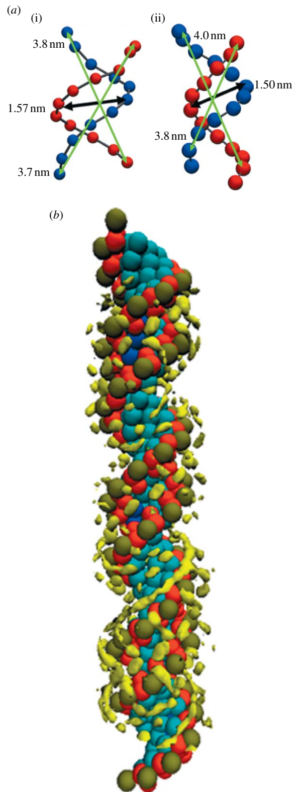
Figure 3. (a) Space-filling representation of phosphate atoms (i) in the X-ray structure of the DNA dodecamer d(\text{CGCGAATTCGCG})_2 (pdb code 1BNA; Drew et al. 1981) and (ii) in the CG DNA after 30 ns of simulation. The end-to-end distances and groove width indicate the close agreement of our model with the X-ray structure. (b) Regions of high \text{Na}^+ density around the DNA 36mer obtained by superimposing approximately 15 000 configurations from a 200 ns trajectory and mapping the \text{Na}^+ density to a 0.1 nm grid. The \text{Na}^+ density is shown in yellow surface representation and the DNA is coloured as in figure 1.
