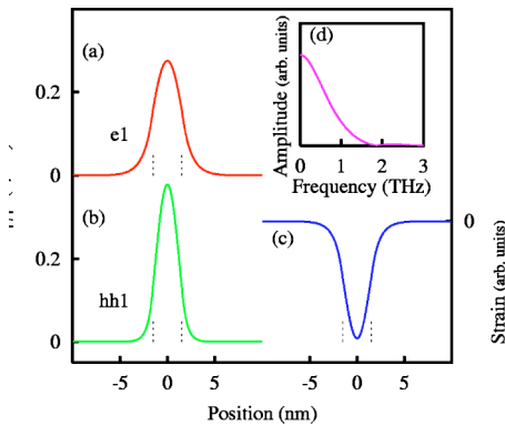
FIG. 5. (Color online) The value of |\phi|^2 for the envelope function of (a) the e1 electronic state and (b) the hh1 heavy hole state for a GaAs/Al 0.3 Ga 0.7 As quantum well of width 3 nm. The excitation of these states with an ultrashort light pulse generates the strain pulse (c) whose frequency spectrum is shown in (d). The dotted lines show the well width.
