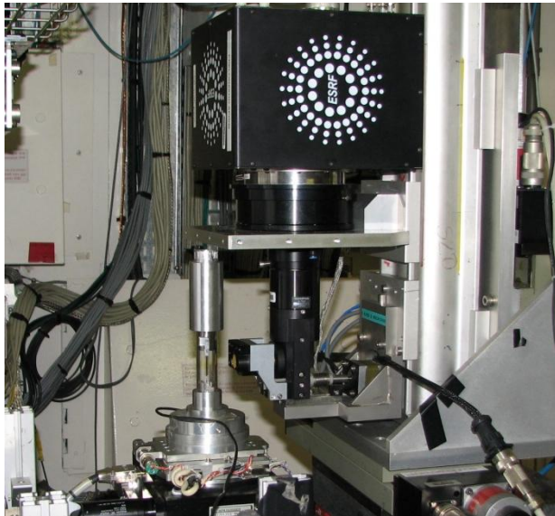
Photograph showing specimen during scanning at id19 - ESRF
