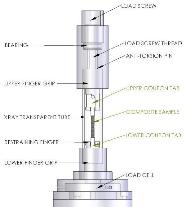
Schematic showing load frame used during testing
