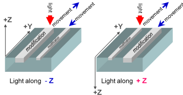
Fig. 3 The illustration of non-reciprocal laser writing - KaYaSo effect ((left and centre) and DIC images of wavy self-organized structures created when writing along the -Y axis and the +Y axis in lithium niobate (right).
