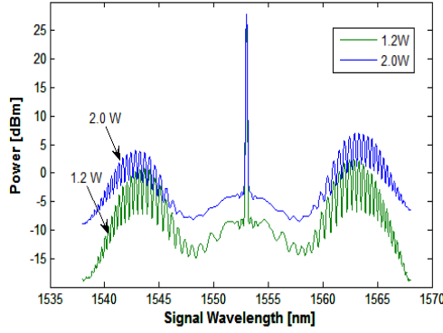
Fig. 2: FOPA2 output spectra when pump and ASE from FOPA1 are coupled into FOPA2 without mid-stage filtering.
