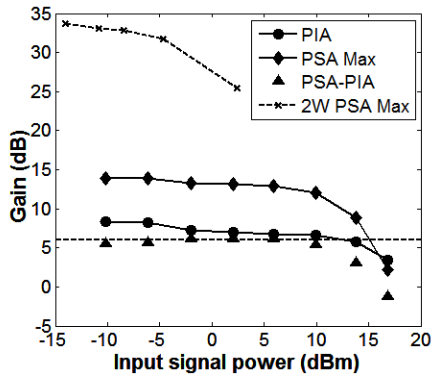
Fig. 6: Measured PIA (circles), PSA maximum (diamonds) and difference between PIA and PSA maximum (triangles) gains of FOPA2 versus input signal power at 1nm detuning and 1.2W pump. Dashed line shows PSA gain at the gain peak with 2W pump
