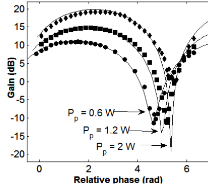
Fig. 3: PSA phase dependent gain at varying pump powers with signal and idler powers equalized. Lines are theoretical curves.
