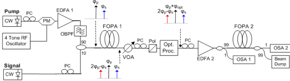
Fig 1: Phase sensitive amplifier setup based on cascaded FOPAs with precise phase and amplitude tuning between the two stages together with the sketch of the phases of the various waves as they propagate through the system. PM: phase modulator, EDFA: erbium doped fibre amplifier, PC: polarization controller.
