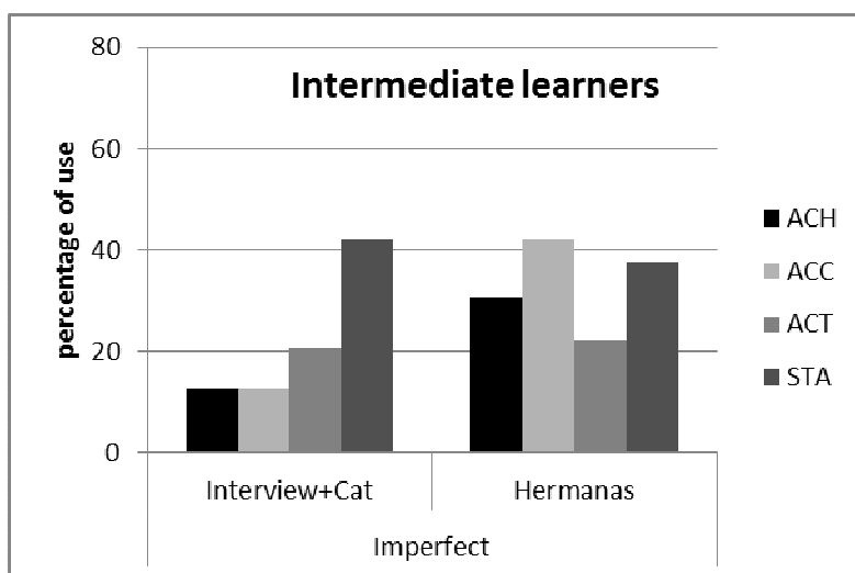
Fig.8. Use of imperfect according to four lexical classes in two tasks
