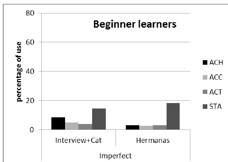
Fig.9. Use of imperfect according to four lexical classes in two tasks
