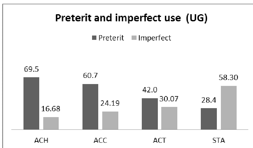
Fig 4. Average use of preterit and imperfect in the three oral tasks for advanced learners
