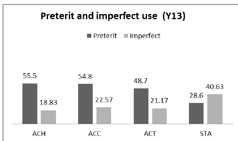
Fig. 3. Average use of preterit and imperfect in the three oral tasks for intermediate learners
