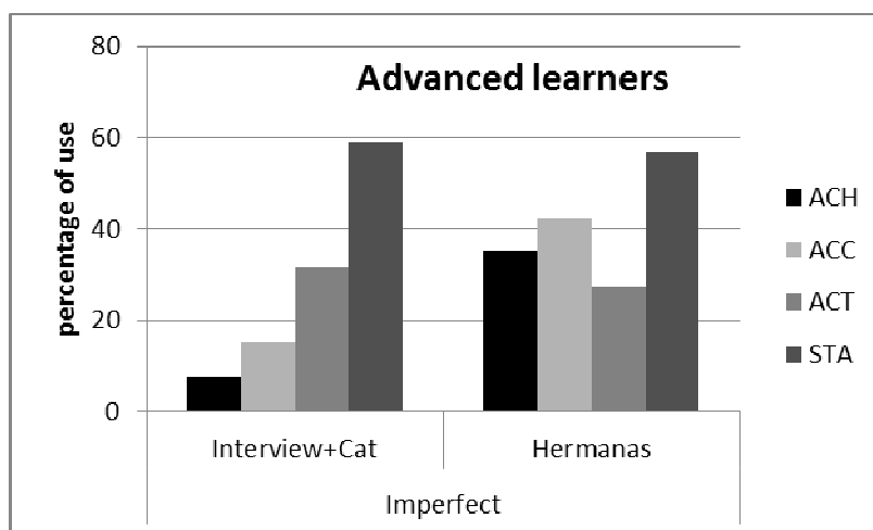
Fig.7. Use of Imperfect according to four lexical classes in two tasks
