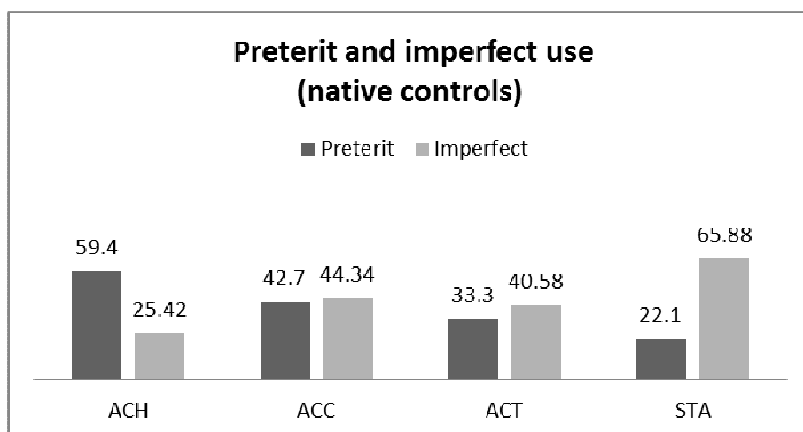
Fig.5. Average use of preterit and imperfect in the three oral tasks for native controls
