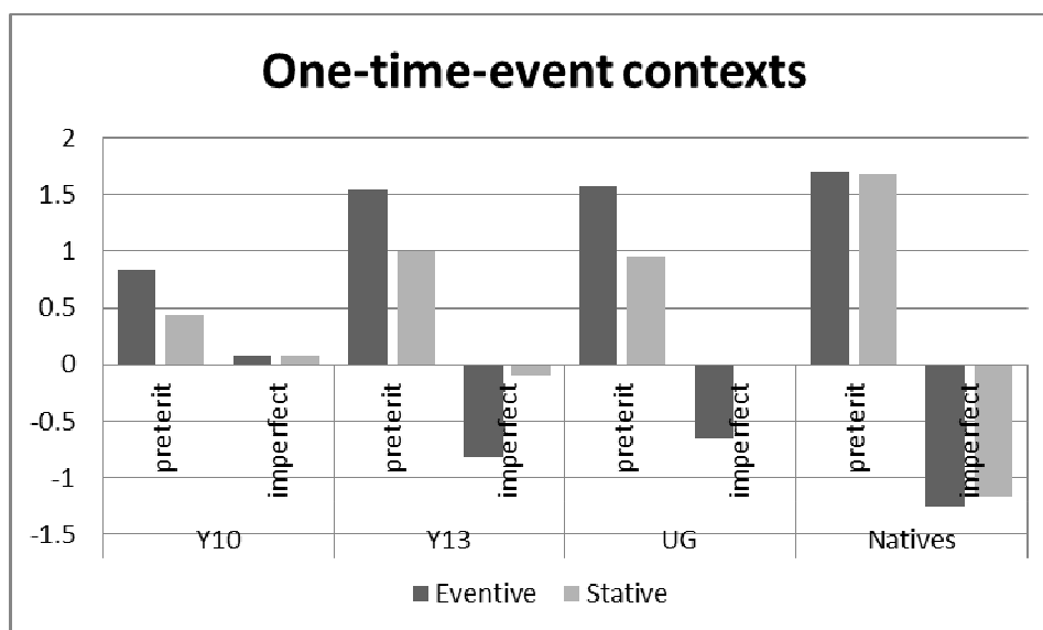
Fig. 11. Mean ratings of input sentences in one-time-event contexts
