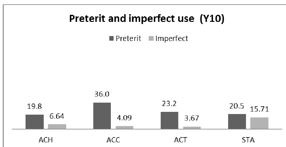
Fig 2. Average use of preterit and imperfect in the three oral tasks for beginner learners
