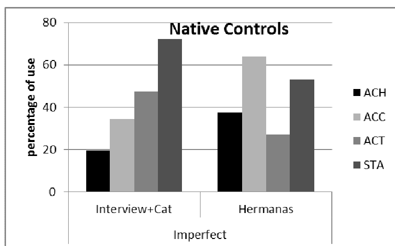
Fig.6. Use of imperfect according to four lexical classes in two controlled tasks
