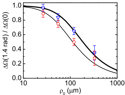
FIG. 6: (color online) (a) Experimental values of the spectral correlation width \Delta\Omega at 1.4 rad, normalized to the width at 0 rad, against beam waist \rho_0 , for \text{TiO}_2 slabs of 3.4 \mu\text{m} (circles, red) and 6.3 \mu\text{m} (triangles, blue) thickness. (lines) Calculated spectral narrowing of the C_T^{(1)} correlation of Eq. (11) for transmission.
