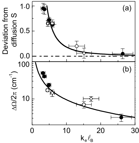
FIG. 10: (a) Experimentally observed deviation from the simple C^{(1)} CBS model, S , against k_e \ell_B . (Open symbols) Pairs of scattering samples before and after infiltration with dodecanol. Lines represent C^{(1)} value of S = 0 (dash-dotted line) and Eq. (17), S = \frac{27}{2}(k_e \ell_B)^{-2} (solid line). (b) Spectral 1/e half width \Delta\Omega of the C^{(1)} correlation function at exact backscattering \theta = 0 against k_e \ell_B for the different materials under study. Line denotes fit using the classical diffusion theory with \Delta\Omega \simeq D/\ell_B^2 \propto 1/k_e \ell_B .
