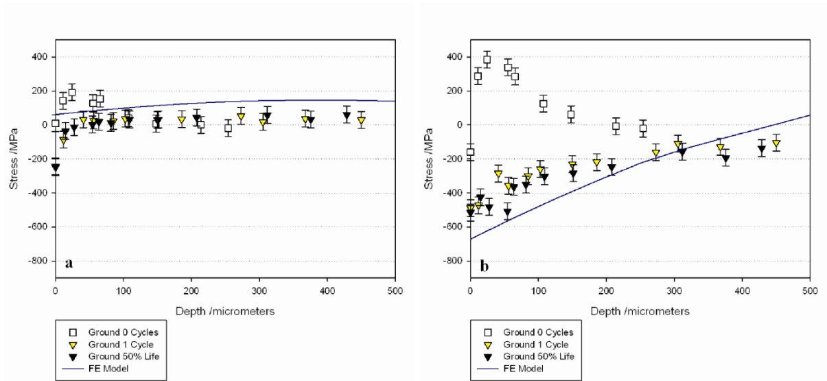
Figure 10: Grinding and post fatigue stresses in a. the transverse direction and b. the longitudinal direction, also showing comparison with residual stresses predicted after one cycle by FE model
