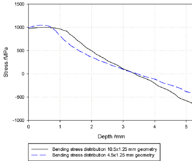
Figure 6: Bending stress (longitudinal direction) in samples tested at strain range 10.5 \times 10^{-3} (determined using FE model)
