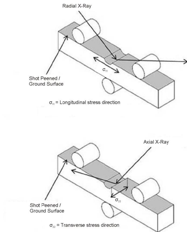
Figure 1: X-Ray diffraction set up
