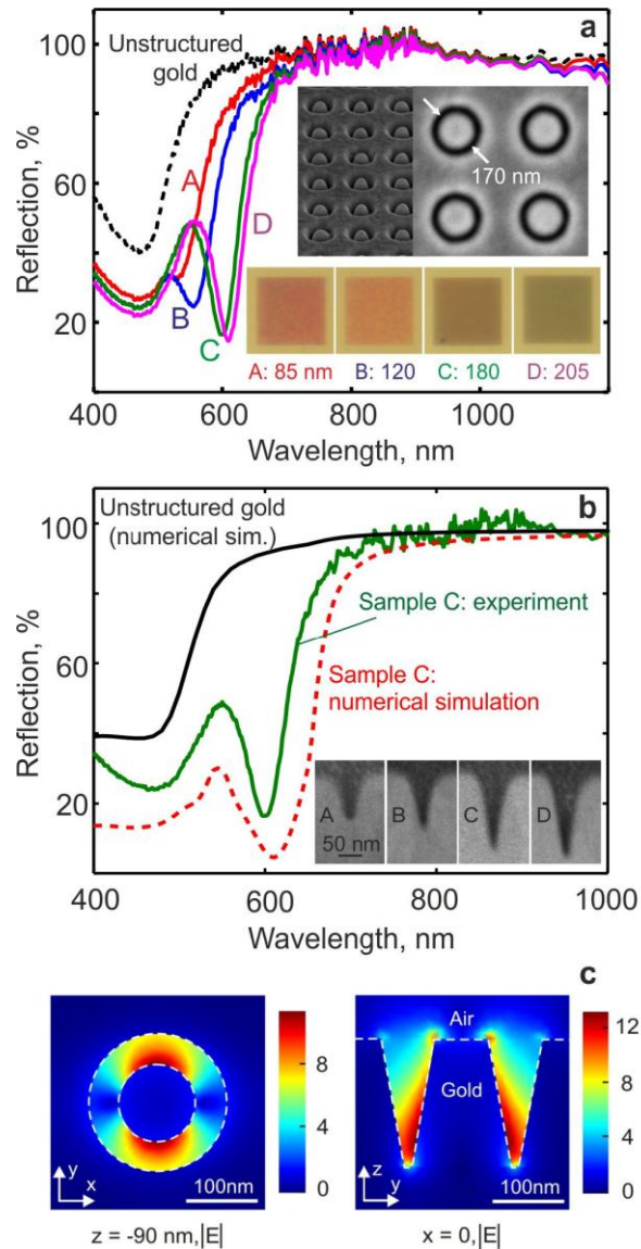
Fig. 2. Changing the color of gold † : (a) Normal incidence reflection spectra for an unstructured gold surface and for the same surface patterned with intaglio metamaterial arrays of 170 nm diameter rings cut to depths ranging from 85 to 205 nm (as labeled, depths derived from FIB calibration). The insets show electron microscope images of the design (at oblique incidence and in plan view) and optical microscope images of the different patterned domains; (b, c) Numerical modeling of gold intaglio metamaterials: (b) Comparison between simulated and experimentally measured reflection spectra. For clarity, data for one of the four designs presented in part (a) are shown on a magnified wavelength axis; (c) Maps of total electric field intensity in a z -plane 90 nm below the top surface of the metal (left) and in the x -plane diametrically bisecting a ring (right). The structure is illuminated at normal incidence with y -polarized plane waves at 610 nm.
