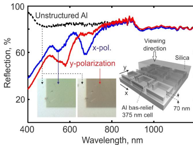
Fig. 3. Anisotropic color control on aluminum † : (a) Normal incidence reflection spectra for an unstructured aluminum/silica interface and for the same surface patterned with a bas-relief metamaterial array of 375 nm asymmetric split rings having a height of ~70 nm. Data are presented for two orthogonal incident polarizations parallel [x] and perpendicular [y] to the split in the rings. The insets show a schematic of the sample structure [with part of the silica layer cut away] and optical microscope images of the patterned domain under the two incident polarizations.
