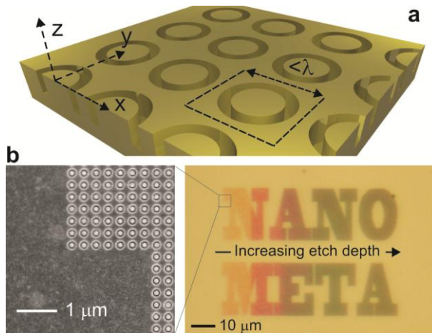
Fig. 1. Metallic structural color † : (a) Artistic impression of a generic intaglio metamaterial array of sub-wavelength single ring meta-molecules inscribed into a metal surface; (b) The realization of this concept in gold: The words 'NANO META' seen under an optical microscope on the right are formed from arrays of 170 nm diameter rings (as shown in the electron microscope image, left) milled to a depth that increases in six steps from 60 to 200 nm across the sample.
