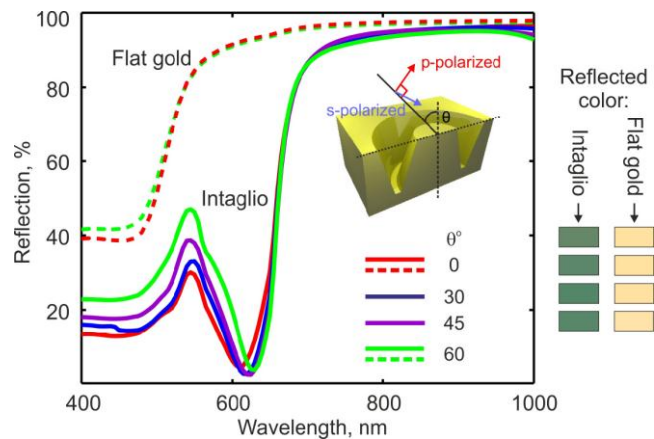
Fig. 5. Color invariance with viewing angle: Numerically simulated reflection spectra and associated perceived colors for a gold intaglio metamaterial array of 170 nm diameter rings with a depth of 180 nm viewed at normal incidence and a selection of oblique angles (as labeled, averaged over incident s- and p-polarizations). For comparison, the corresponding perceived color of an unstructured gold surface is shown for each viewing angle and reflection spectra for the unstructured metal at 0° and 60° angles are plotted.
