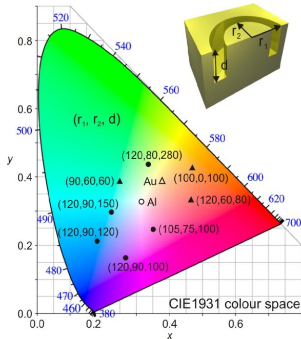
Fig. 4. Metallic color palette † : CIE1931 chromaticity diagram overlaid with points corresponding to the simulated reflected colors of single ring intaglio metamaterial designs in aluminum (circular symbols) and gold (triangles), labeled according to their structural parameters (external radius r_1 , internal radius r_2 , depth d , array period = 300 nm in all cases). Points for the unstructured metals are indicated by open symbols.
