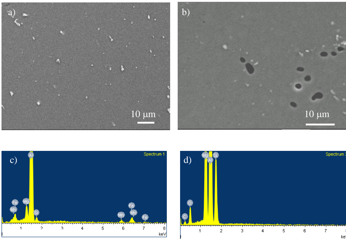
Fig. 3 SEM images of four turns of HPT processed ( a ) Al-1Mg at edge of sample and ( b ) Al-3Mg at centre of sample and particles identification by EDS. ( c ) dark and ( d ) white particles in ( b ) are identified as \alpha -Al 12 (Fe,Mn)Si and Mg 2 Si, respectively.
