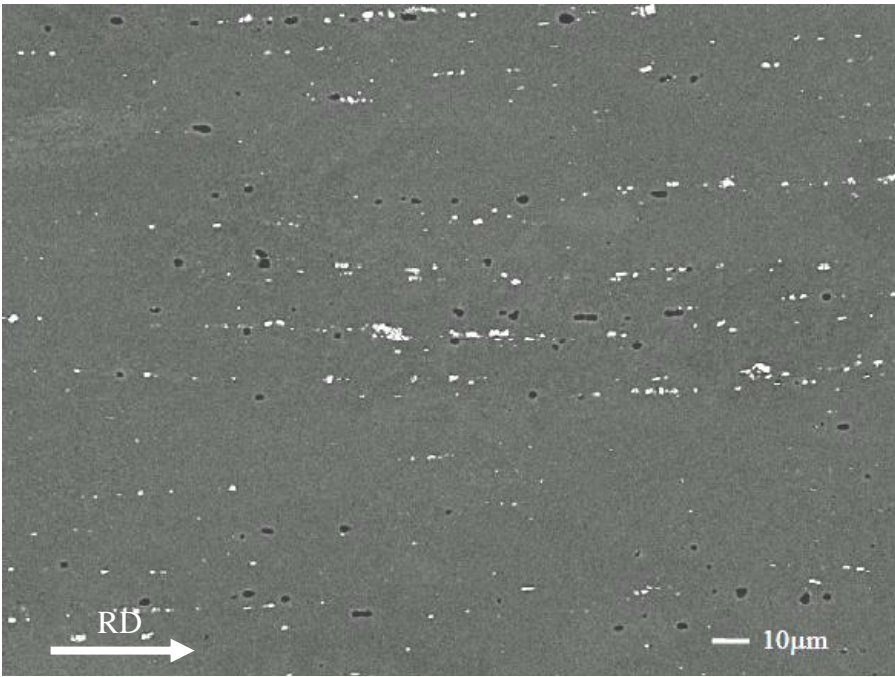
Fig. 1 SEM image of rolled Al-3Mg alloy (i.e. pre-HPT). The particles are aligned in the rolling direction.
