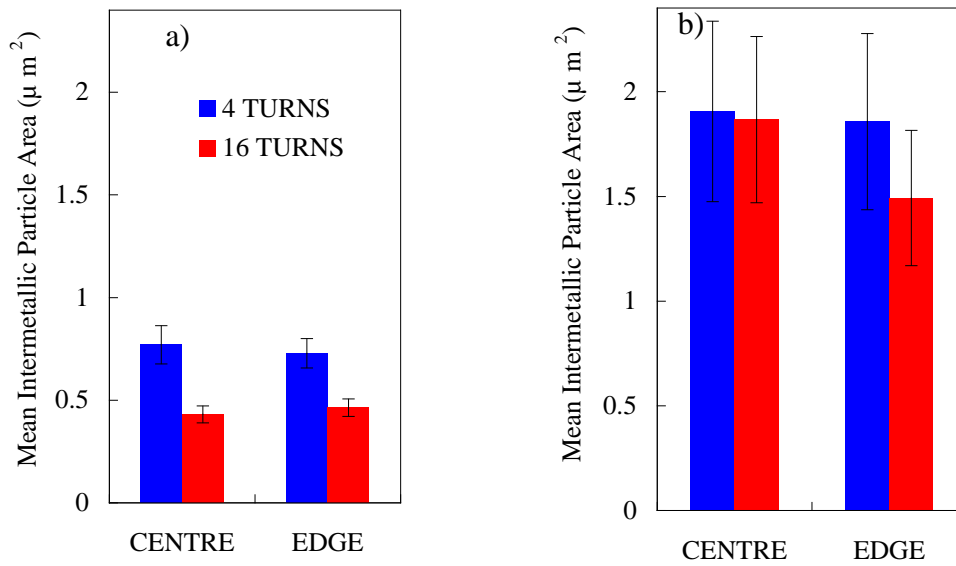
Fig. 7 Effect of HPT turn number on the mean size of intermetallic particles of Al-3Mg measured by SEM. (a) \alpha -Al 12 (Fe,Mn) 3 Si, (b) Mg 2 Si. Error bars represent the standard error of the mean.
