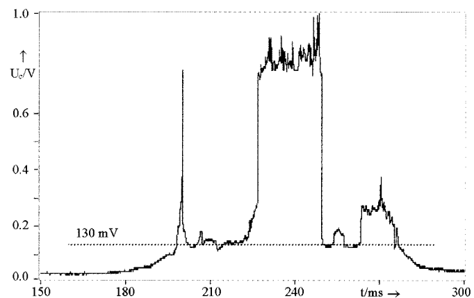
Fig. 8. Softening and melting voltages are often exceeded (Cycle 145, F_C = 500 mN, U_S = 14.0 V; I_C \approx 54 mA; v = 0.1 mm/s).
