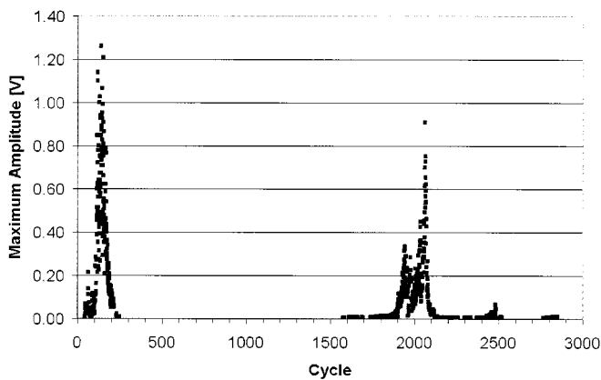
Fig. 4. Maximum voltage-drop over fretting cycle ( F_C = 500 mN, U_S = 14.0 V; I_C \approx 54 mA; v = 0.1 mm/s).
