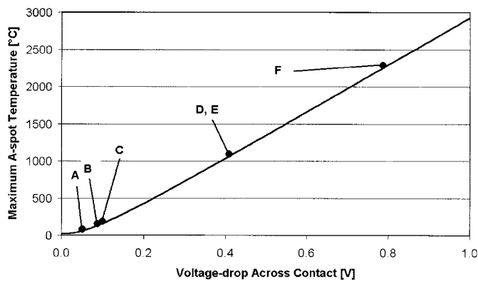
Fig. 1. Relation between contact voltage-drop and maximum \alpha -spot temperature.
