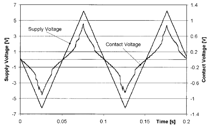
Fig. 10. Supply voltage and contact voltage-drop over time for stationary contacts.
