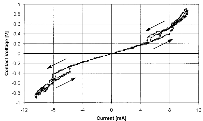
Fig. 13. Voltage/current characteristic for a stationary contact.
