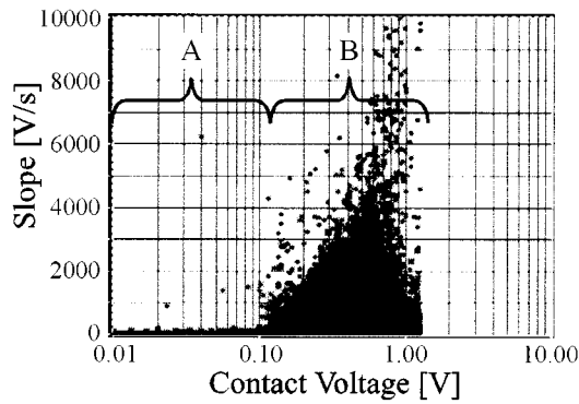
Fig. 9. Slope of all recorded events during one experiment (Cycle 1...600, F_C = 500 mN, U_S = 14.0 V; I_C \approx 54 mA; v = 0.1 mm/s).
