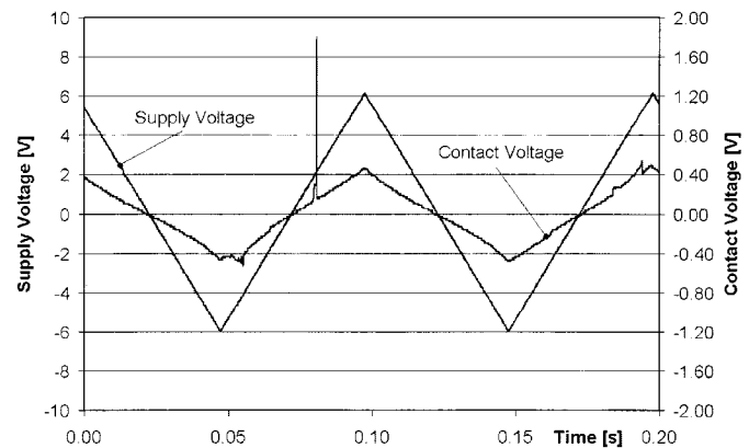
Fig. 12. Supply voltage and contact voltage-drop after 4 min (Note the difference in scale).
