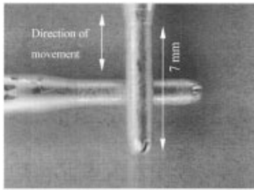
Fig. 3. Crossed-rod configuration used in this study. The lower contact terminal moves in the direction indicated by the arrows.
