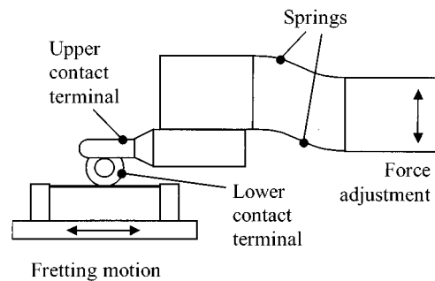
Fig. 2. Schematic diagram of the test rig.
