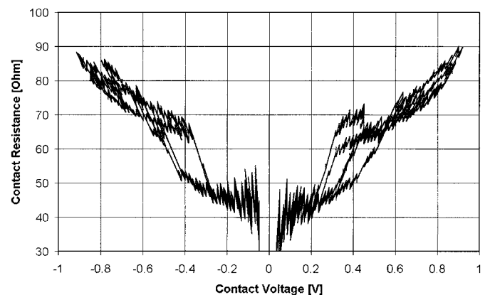
Fig. 14. Resistance/voltage characteristic for a stationary contact.
