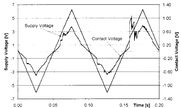
Fig. 11. Supply voltage and contact voltage-drop after 2 min.
