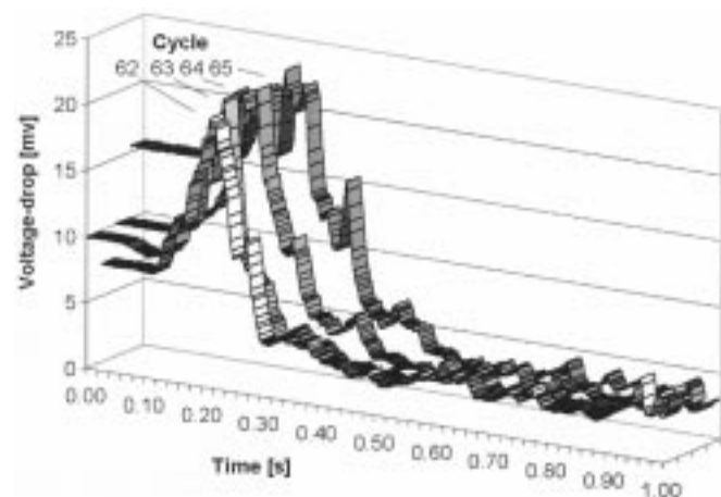
Fig. 7. Repetition of events in consecutive cycles ( F_C = 500 mN, U_S = 14.0 V; I_C \approx 54 mA; v = 0.1 mm/s; trigger level: 20 mV).
