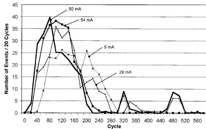
Fig. 6. Average number of events per 20 cycles for currents of 9 mA, 29 mA, 54 mA, and 92 mA at 14 V supply voltage.
