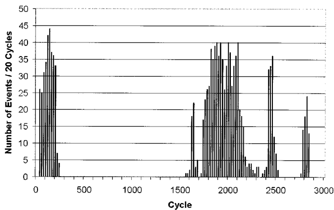
Fig. 5. Number of events per 20 cycles ( F_C = 500 mN, U_S = 14.0 V; I_C \approx 54 mA; v = 0.1 mm/s).
