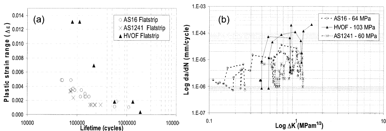
Figure 5: (a) \Delta\varepsilon vs N_f data for AS16, AS1241 and HVOF flat strip linings (b) short crack growth rate comparison in AS16, AS1241 and HVOF flat strip linings.
