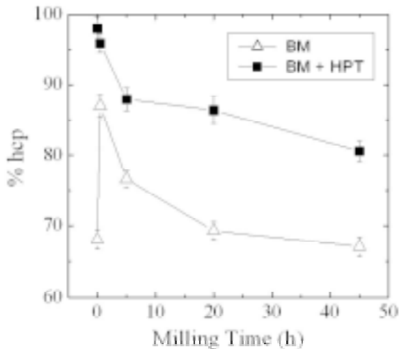
Fig. 3.3. Milling time dependencies of the hcp weight percentage for as-milled (pre-compacted) Co powders ( \Delta -) and powders ball milled (BM) and consolidated by HPT ( \blacksquare -). The lines are guides to the eye.
