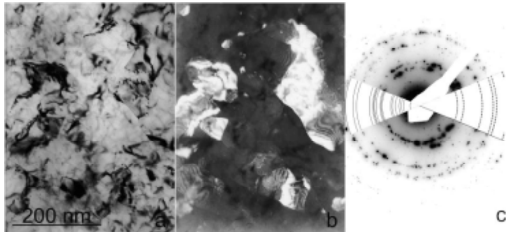
Fig. 5.4. BF (a), DF (b) images and SAED TEM pattern (c) of the Al-4%Mg-10%Zn alloy after HPT deformation.
