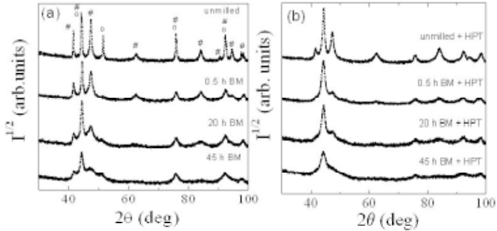
Fig. 3.1. (a) XRD patterns of Co before milling and after ball milling (BM) for 0.5, 20 and 45 h. (b) XRD patterns obtained after subjecting to high pressure torsion (HPT) unmilled Co powders and Co milled for 0.5, 20 and 45 h. The symbols # and o denote the hcp and fcc phases, respectively.
