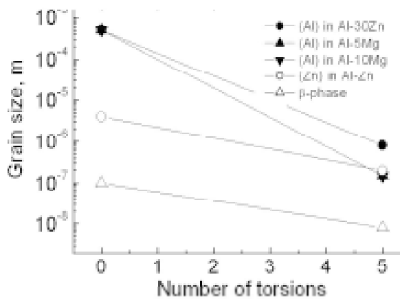
Fig. 5.5. Grain size of (Al) solid solution and second phases (Zn) and \text{Al}_3\text{Mg}_2 before and after HPT.
