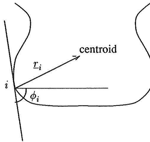
Figure 23.1: Shape Representation Using The GHT
