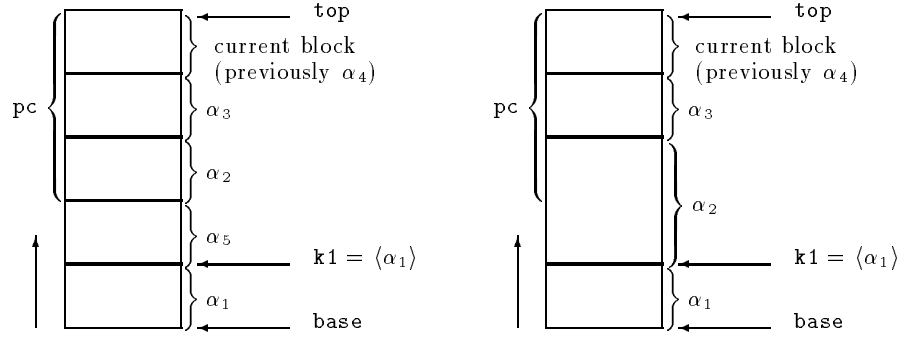
Fig. 4. Stack representation after invocation of a partial continuation preserving marks
