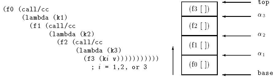
Fig. 1. Program 1 and stack representation
