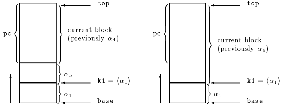
Fig. 5. Stack representation after invocation of a partial continuation without preservation of marks
