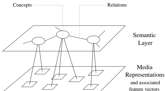
Figure 1: Multimedia Thesaurus Architecture
