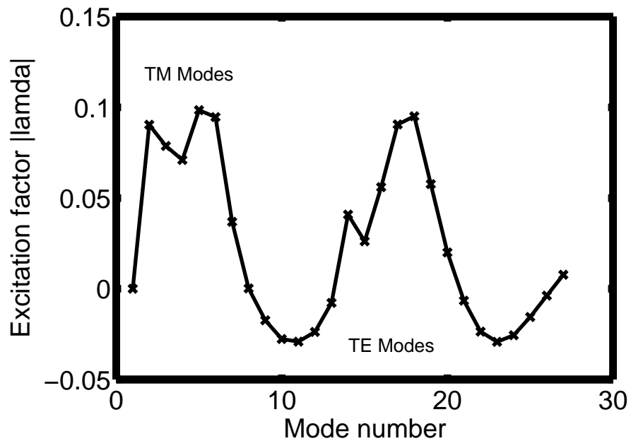
Excitation factor shift
