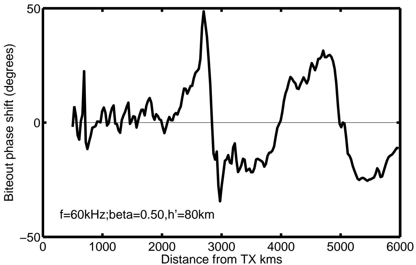
Phase shift due to biteout
