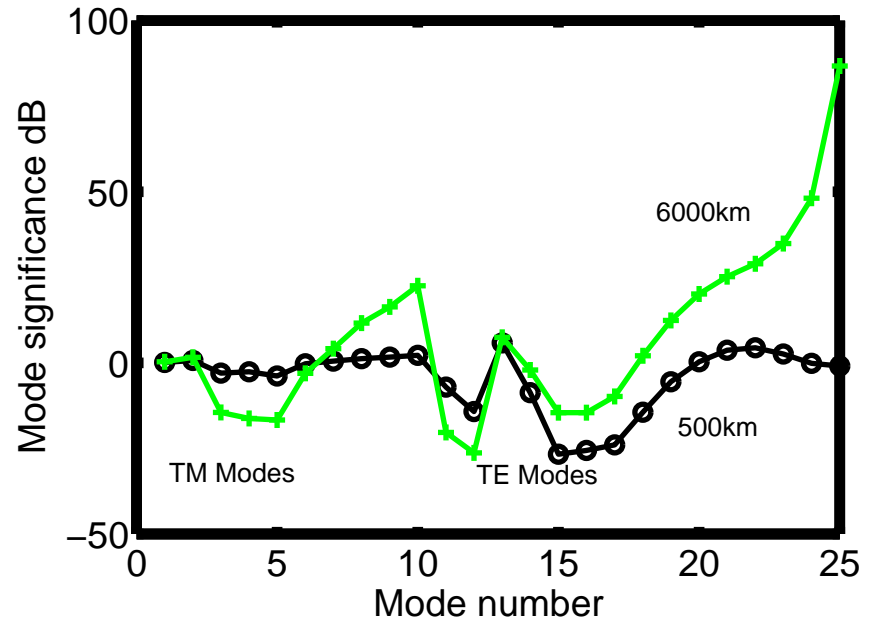
Mode amplitude shift/range=500,6000km
