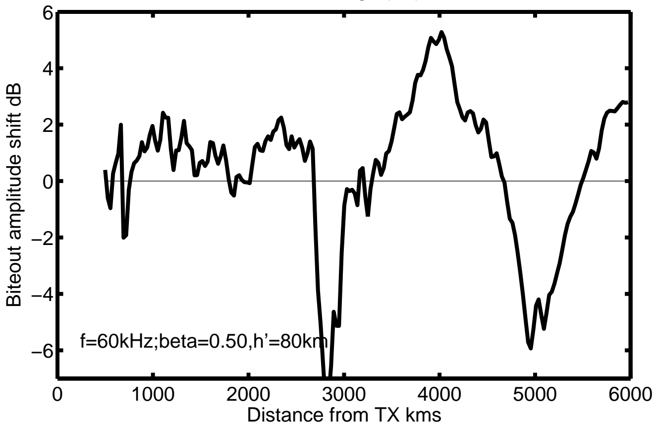
Received VLF field change (dB) due to biteout
