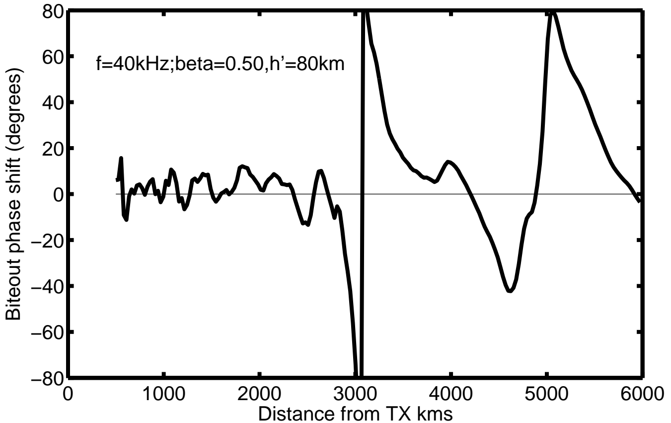
VLF phase shift due to biteout
