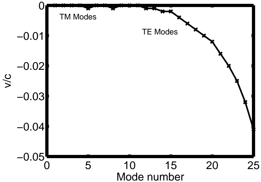
v/c shift due to biteout; F=40kHz
