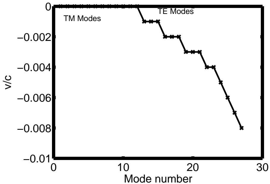
v/c shift due to biteout; F=80kHz
