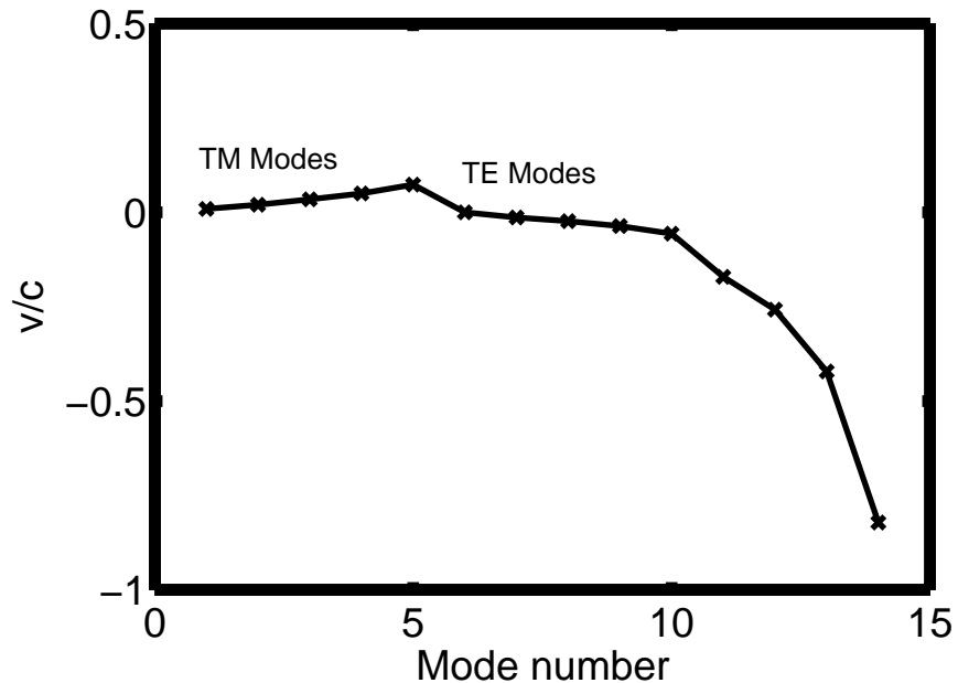
v/c shift due to biteout; F=20kHz
