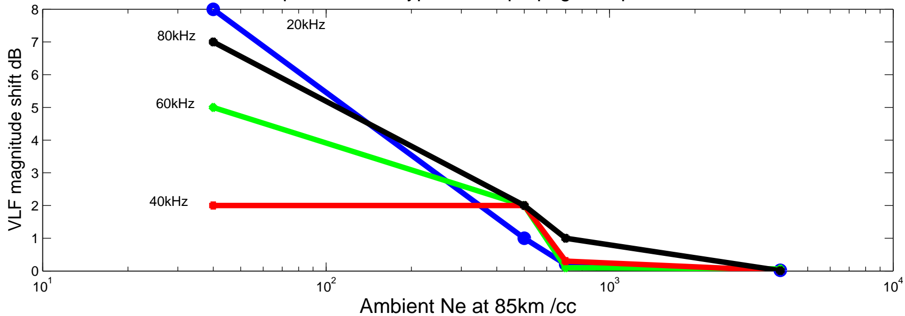
Profile dependence of typical VLF propagation perturbations
