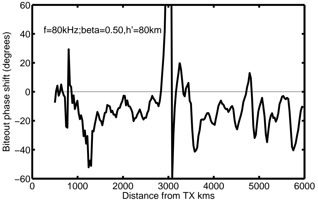
Phase shift due to biteout
