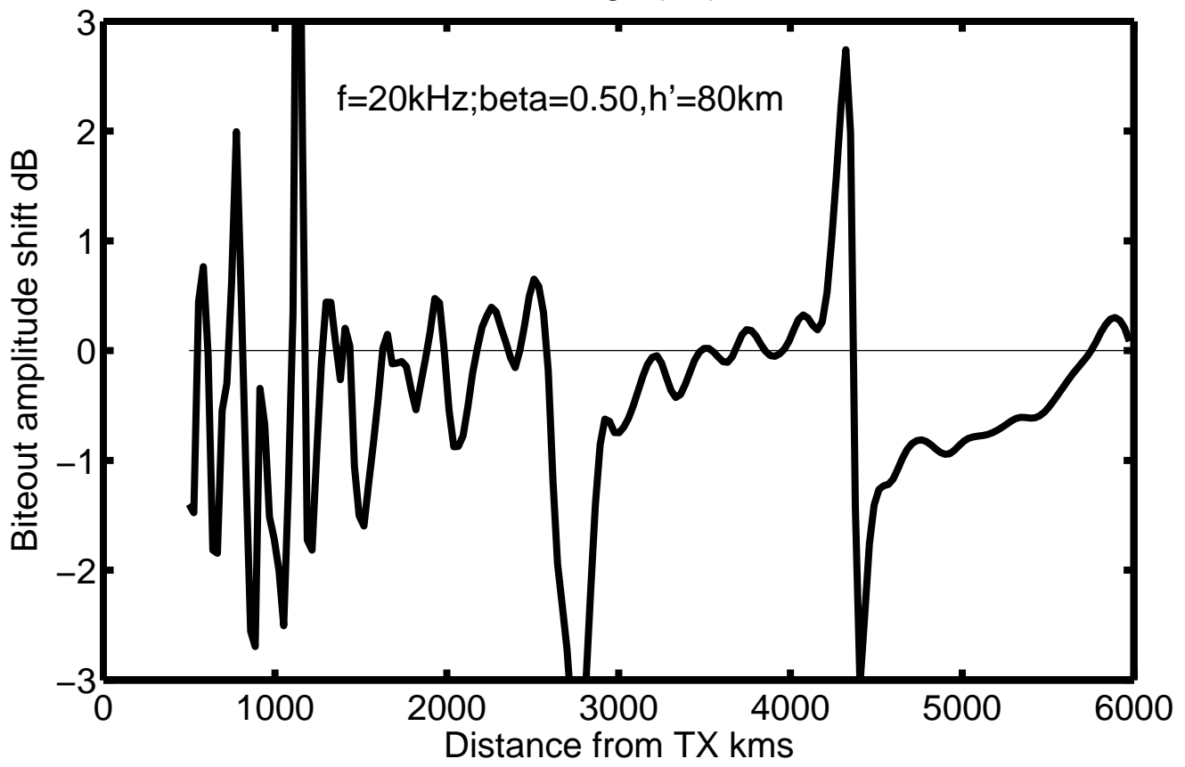
Received field change (dB) due to biteout
