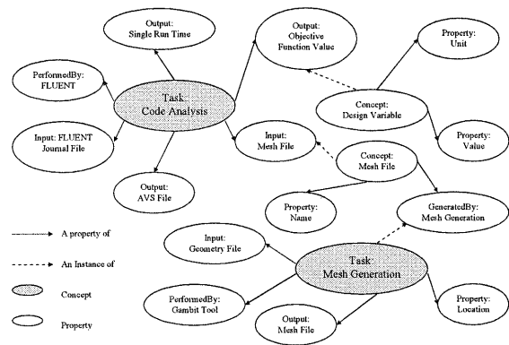
Figure 7: Example semantic task description
