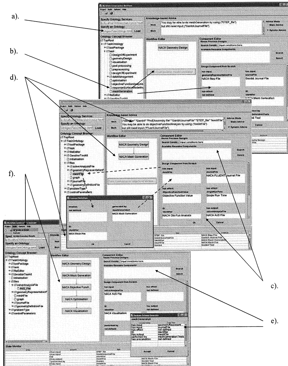
Figure 9: Screenshots of workflow construction environment
