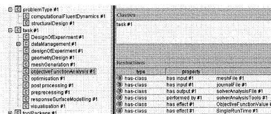
Figure 3: EDSO task ontology
