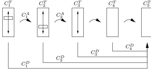
Fig. 5. mSpace column constraints
