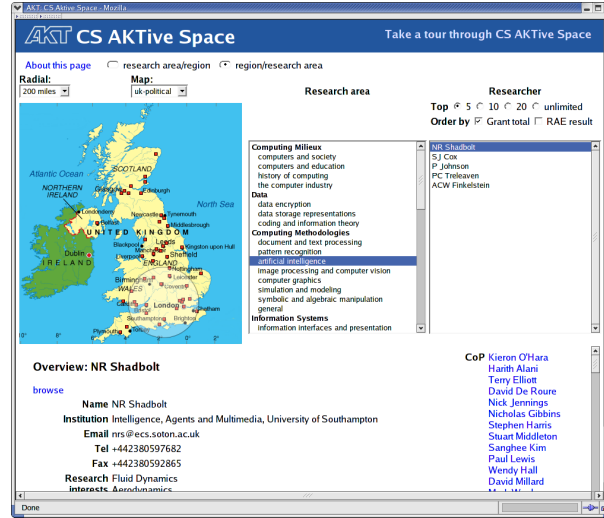
Fig. 2. CS AKTiveSpace: an example of an mSpace interface
