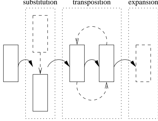
Fig. 7. mSpace operations
