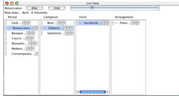
Fig. 1. Spatial multicolumn view for classical music slice
