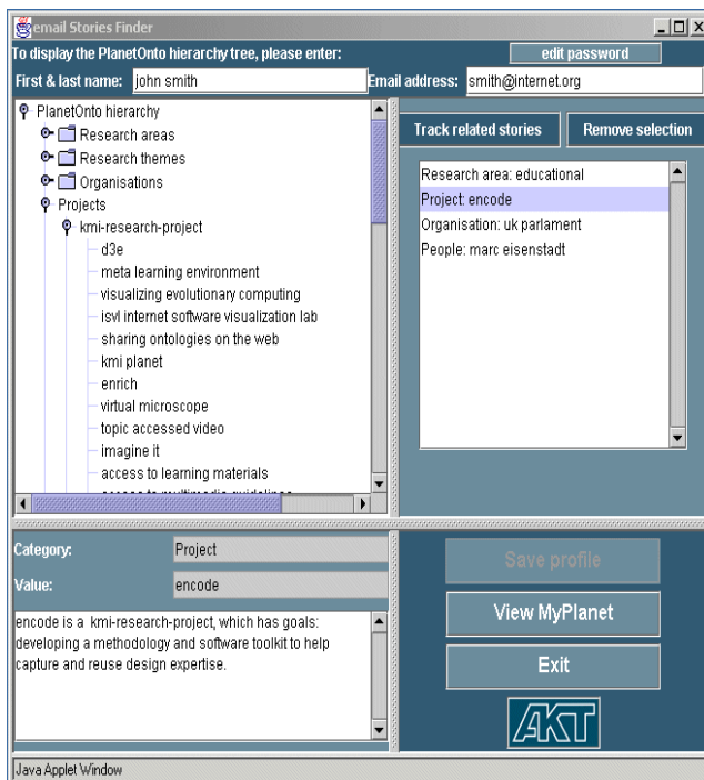
Figure 4: The designated user interface of MyPlanet.
