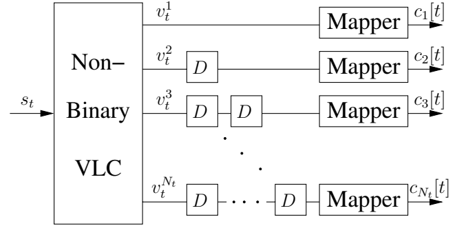
Figure 1: Block diagram of the VL-STCM encoder.
