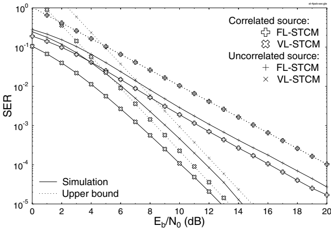
Figure 5: SER versus E_b/N_0 performance of the VL-STCM and FL-STCM schemes, when communicating over uncorrelated Rayleigh fading channels using 4PSK, N_t = 3 and N_r = 2 .
