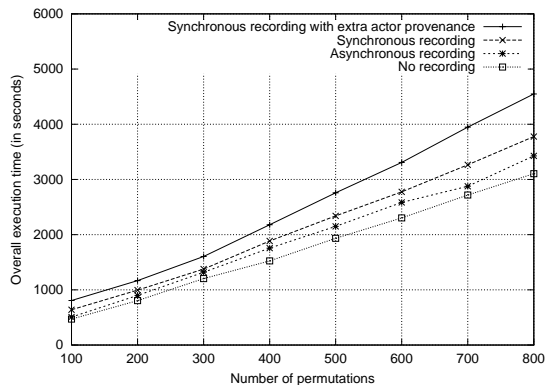
Fig. 2: Recording Performance
