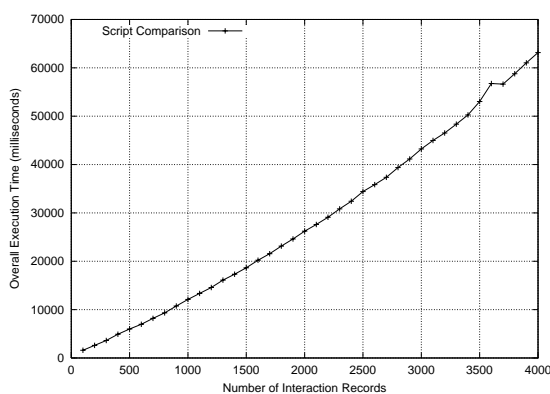
Fig. 3: Query Performance
