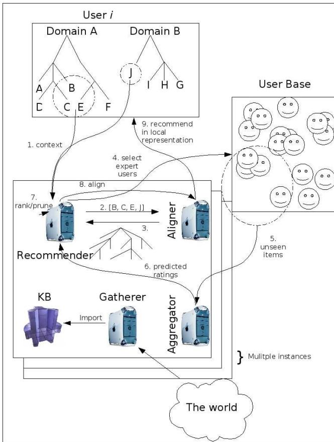
Figure 2: Overview of the recommender system architecture
