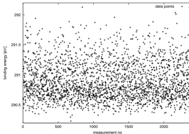
Fig. 1. Example spectral data for three sources ( M = 3 ). The parameters are \mu_1 = 290.7, \sigma_1 = 0.15, \phi_1 = 0.61, \mu_2 = 291.13, \sigma_2 = 0.18, \phi_2 = 0.33 , and \mu_3 = 291.55, \sigma_3 = 0.21, \phi_3 = 0.06 (modeled after the spectrum of NH_3 molecules; cf. [4])
