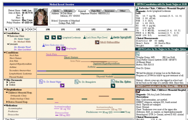
Figure 2: The LifeLines system. Related entities are shown, for example each doctor and their consultations, medications are shown by a colour, but the user must themselves link those actions by panning vertically.
