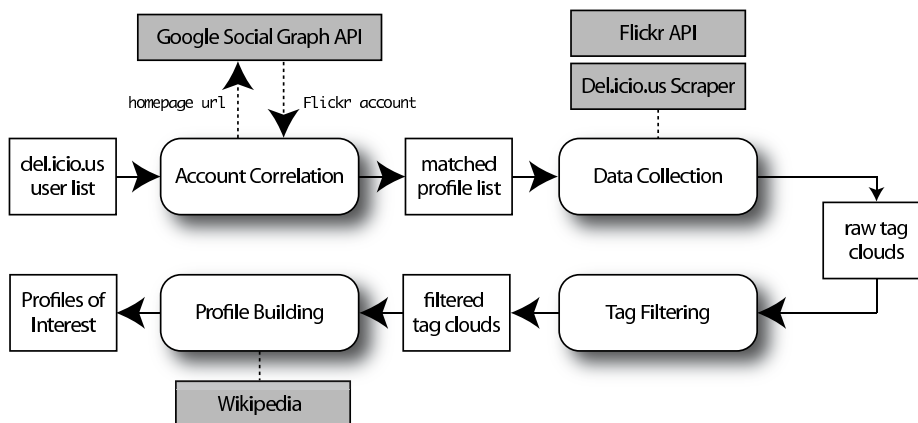
Fig. 1. An Architecture for building Semantic Profiles of Interest
