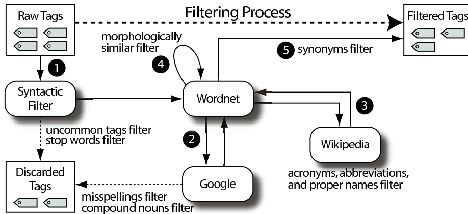
Fig. 2. The tag filtering process
