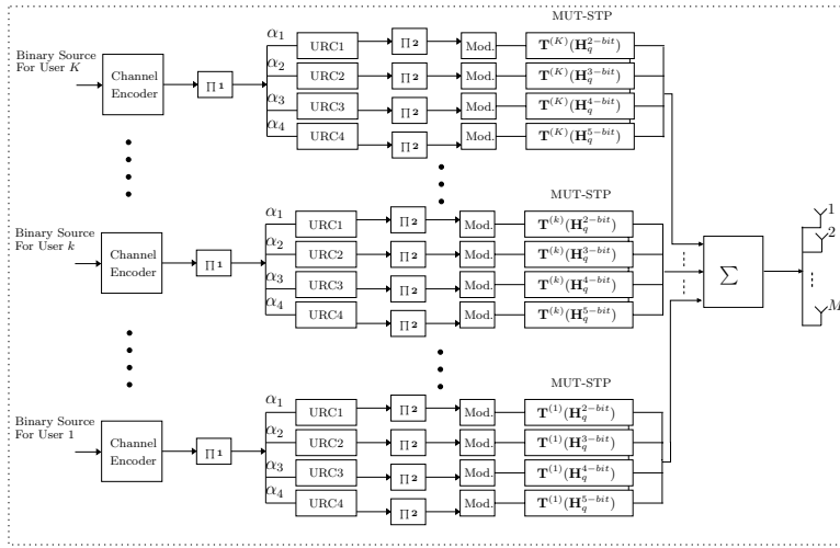
Fig. 4. The structure of the BS's transmitter in the iterative DL-SDMA system using ECO-CQ
