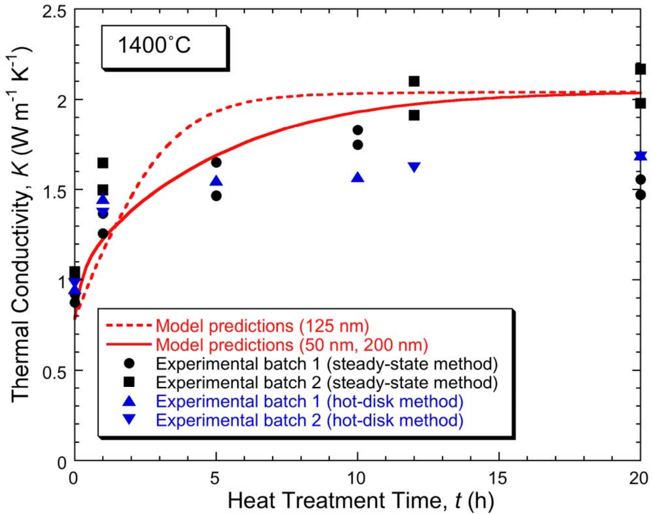
Fig.10 Comparison [77] between experimental data and model predictions for the through-thickness thermal conductivity, as a function of the duration of a prior heat treatment at 1400°C. The two predicted curves correspond to different assumptions about the range of values exhibited by the inter-splat spacings and the opening of the intra-splat microcracks.
