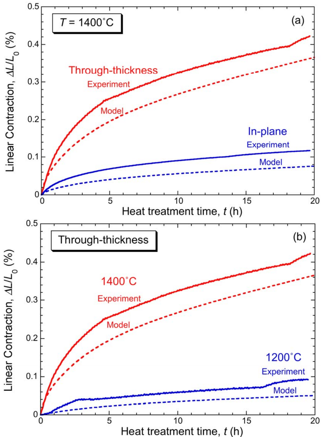
Fig.8 Comparison [77] between experimental data and model predictions for coating shrinkage, (a) at 1400^\circ\text{C} in both through-thickness and in-plane directions and (b) in the through-thickness direction, at both 1200^\circ\text{C} and 1400^\circ\text{C} .
