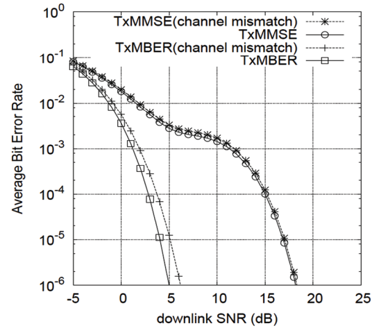
Figure 4. Average BER performance of the downlink Tx beamforming schemes with both the MMSE and MBER designs for the TDD-SDMA induced MIMO system which consists of a four-antenna BS to support four single-antenna BPSK MTs, when the downlink and uplink channels mismatch.
