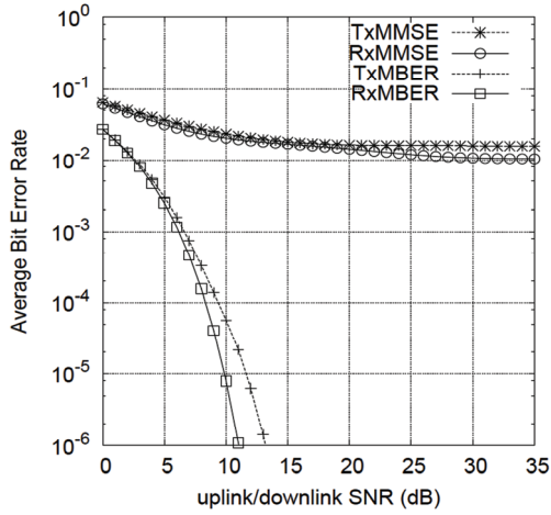
Figure 5. Average BER performance comparison of the uplink Rx and downlink Tx beamforming schemes with both the MMSE and MBER designs for the TDD-SDMA induced MIMO system which consists of a four-antenna BS to support six single-antenna BPSK MTs.
