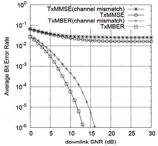
Figure 7. Average BER performance of the downlink Tx beamforming schemes with both the MMSE and MBER designs for the TDD-SDMA induced MIMO system which consists of a four-antenna BS to support six single-antenna BPSK MTs, when the downlink and uplink channels mismatch.
