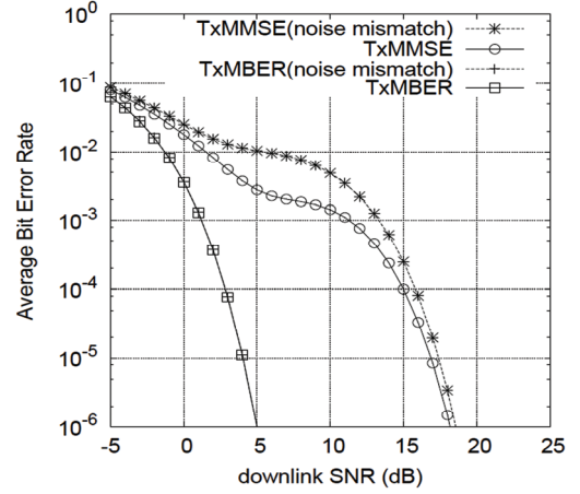
Figure 3. Average BER performance of the downlink Tx beamforming schemes with both the MMSE and MBER designs for the TDD-SDMA induced MIMO system which consists of a four-antenna BS to support four single-antenna BPSK MTs, when the downlink and uplink noise powers mismatch.
