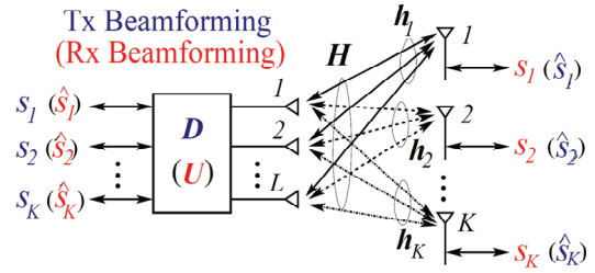
Figure 1. Schematic diagram of the TDD-SDMA induced MIMO system employing transmit and receive beamformings at the BS. The system employs L antennas at the BS to support K single-antenna MTs.
