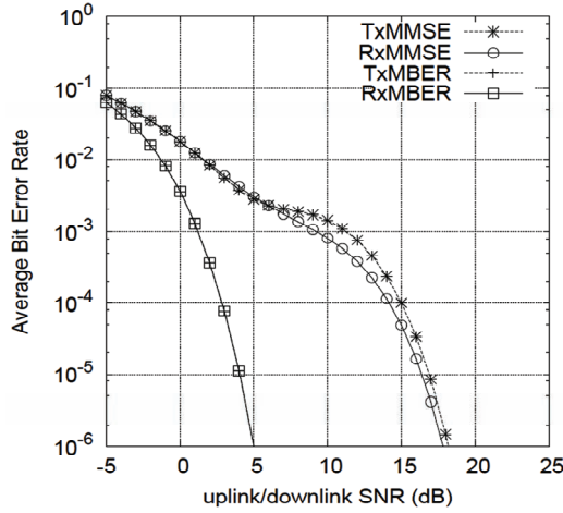
Figure 2. Average BER performance comparison of the uplink Rx and downlink Tx beamforming schemes with both the MMSE and MBER designs for the TDD-SDMA induced MIMO system which consists of a four-antenna BS to support four single-antenna BPSK MTs.
