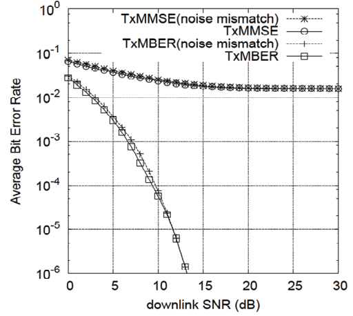
Figure 6. Average BER performance of the downlink Tx beamforming schemes with both the MMSE and MBER designs for the TDD-SDMA induced MIMO system which consists of a four-antenna BS to support six single-antenna BPSK MTs, when the downlink and uplink noise powers mismatch.
