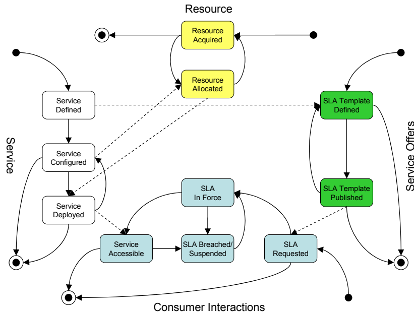
Fig. 2. Lifecycle Models
