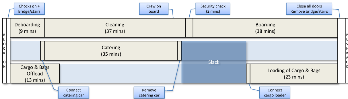
Fig. 7. Turn-Around Timeline Example
