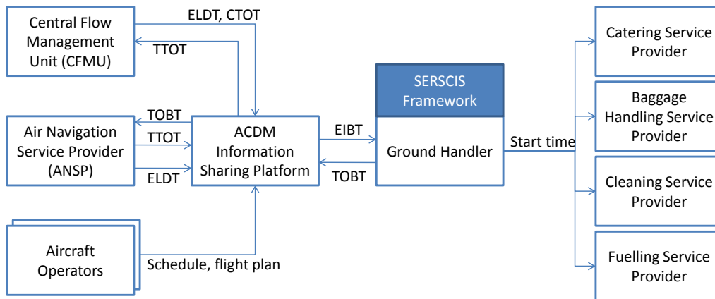
Fig. 10. SERSCIS Components and Services in the A-CDM Test Case
