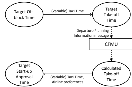
Fig. 9. Communication CFMU-ATC and TSAT Calculation
