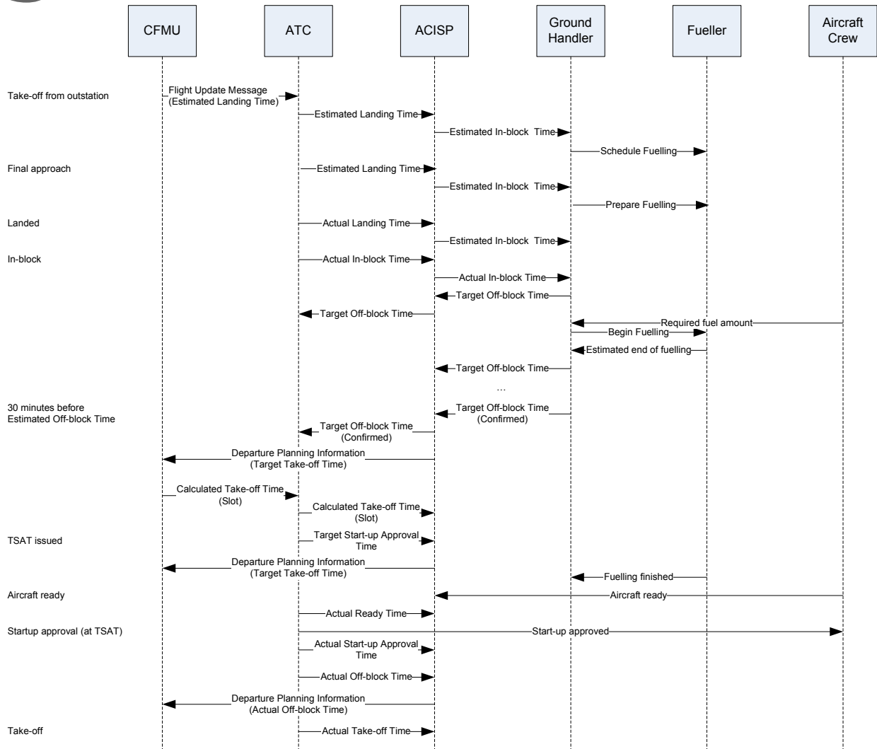
Fig. 8. Turnaround Sequence Diagram showing Information Flow
