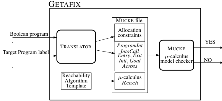
Figure 1. Architecture of the GETAFIX tool
