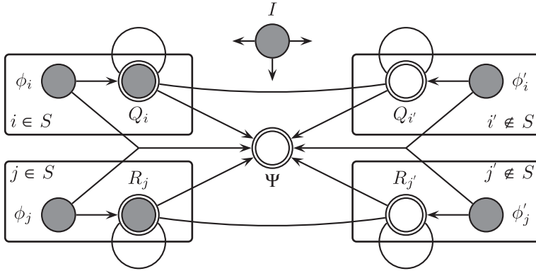
Fig. 1. Bayesian network for marginalizing hyperparameters using Bayesian Monte Carlo. Shaded nodes are known and double-circled nodes are deterministic given all their parents. All Q nodes are correlated with one another, as are all R nodes, and the context I is correlated with all nodes.
