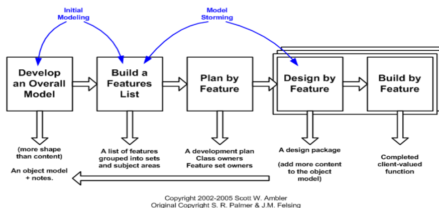
Figure 2.4: FDD Model diagram (Ambler 2005-2009)
