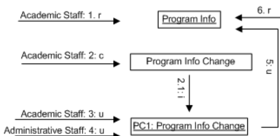
Figure 3 Modelling City University's SSPD
