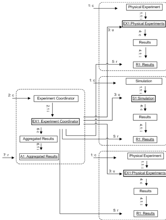
Figure 6 NEEsGrid Experiment RO Model
