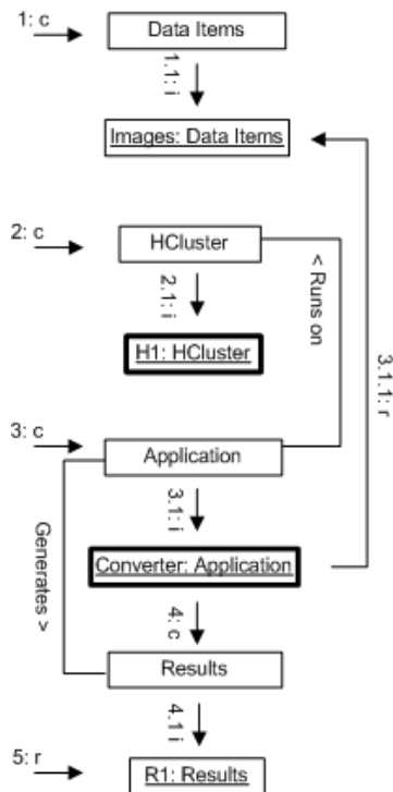
Figure 5 NYT Cloud Computing RO Model
