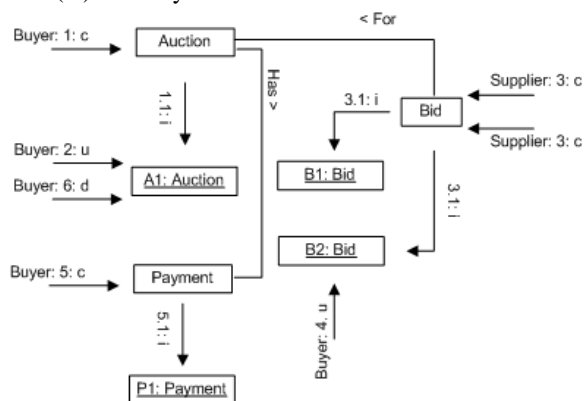
Figure 4 Modelling Reverse Auctioning
