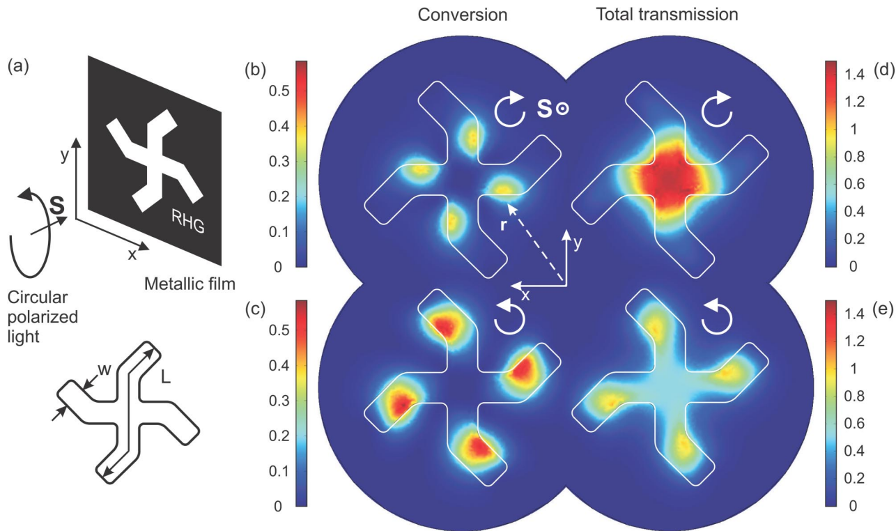
FIG. 1. (Color online) (a) General arrangement of the numerical simulations. Left field maps : Intensity [S_0^{\text{tr}}(\mathbf{r}) \pm S_3^{\text{tr}}(\mathbf{r})] / [2S_0^{\text{in}}(\mathbf{r})] of the polarization converted component of transmitted radiation for (b) RCP and (c) LCP incident waves. Right field maps : Intensity S_0^{\text{tr}}(\mathbf{r}) / S_0^{\text{in}}(\mathbf{r}) of total transmitted radiation for (d) RCP and (e) LCP incident waves. For all field maps, the incident wave propagates in the direction of the reader. The arrows illustrate the rotational direction of the electric field vector of the incident wave in the plane of the structure.
