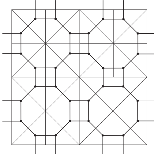
FIGURE 3. Tesselation of the euclidean plane given by the triangle group \Delta(2, 4, 4) , and its dual tesselation.
