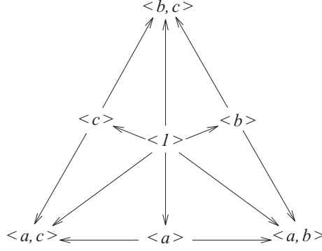
FIGURE 2. Davis complex (quotient) for a triangle group.
