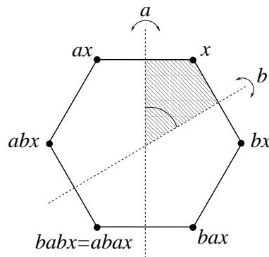
FIGURE 1. Coxeter cell for a dihedral group.
