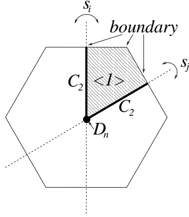
FIGURE 5. Coxeter cell of rank 2
