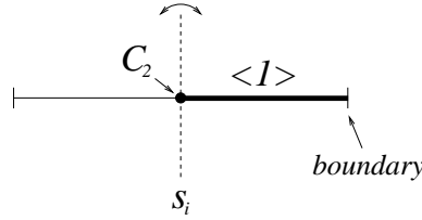
FIGURE 4. Coxeter cell of rank 1
