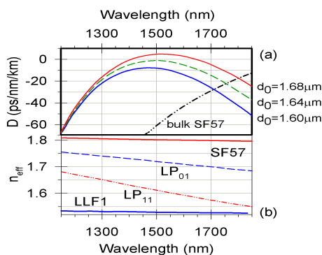
Fig. 1: Numerical simulation of (a) dispersion profile and (b) effective index n_{\text{eff}} of \text{LP}_{01} and \text{LP}_{11} modes of a SF57-LLF1 step-index fibre
