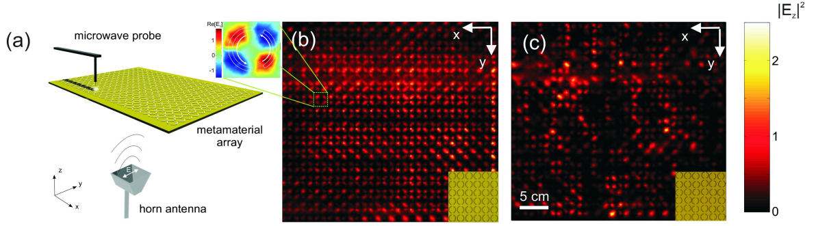
Fig. 1: (a) Drawing of the experimental setup. (b-c) Maps of the electric field intensity at the vicinity of the regular (b) and disordered (c) asymmetrically split-ring array. The inset in (b) shows the real part of the electric field for a single unit cell, where the arrows indicate the direction of the currents flowing on the arcs.
