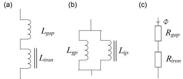
Fig. 4. Series equivalent circuit of inductances (a); parallel equivalent circuit of inductances (b); magnetic circuit of the limb in terms of reluctances (c).
