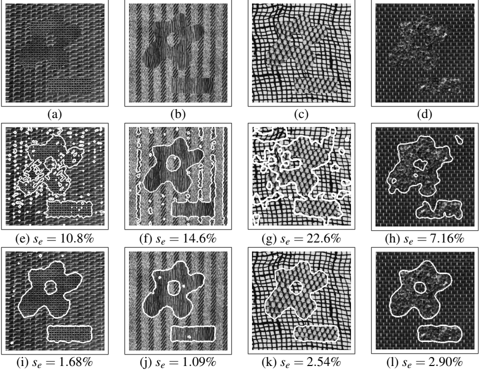
Figure 2: Segmentation Results. (a)-(d) the original images, (a) and (b) are 640 \times 640 and (c) and (d) are 256 \times 256 , (e)-(h) using CGMRF[ 14 , 15 ] and (i)-(l) using PL histogram. \mu = 10^{-7} and \lambda_i = 20 .
