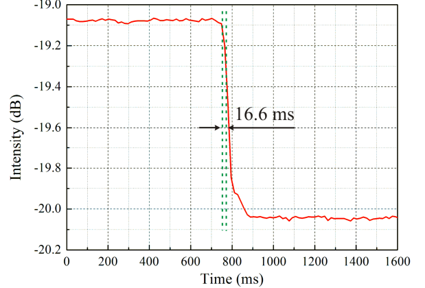
Fig. 4. Measurement of MFCT response time of sample 1: the temporal dependence of the MFCT reflected intensity was recorded for a rapid temperature change, resulting in a response time of \sim 16.6 ms.
