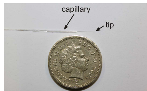
Fig. 2. Picture of a MFCT. The capillary has 600 \mu\text{m} outer diameter.
