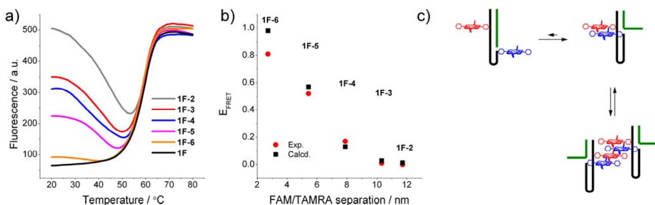
Fig. 2 a) Fluorescence melting curves of the DNA switch by monitoring FAM emission ( \lambda_{\text{exc}} 495 nm, \lambda_{\text{em}} 510 nm); calculated vs experimental FRET of the modified system; b) FAM and TAMRA system 1F ; c) putative intra- and intermolecular stacking of the porphyrins in the DNA systems.
