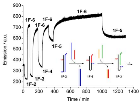
Fig. 3 Real-time monitoring of the switching between the five different switching states, recording acceptor emission ( \lambda_{\text{ex}} = 495 nm, \lambda_{\text{em}} = 583 nm), and schematic drawing of the first steps. The final switches between 1F-5 and 1F-6 show the reversibility and stability of the system.
