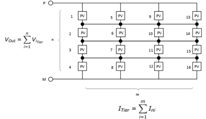
Figure 6: Total Cross Tied configuration
