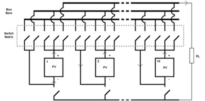
Figure 11: Switch Structure for fully dynamic IEq-DPVA
